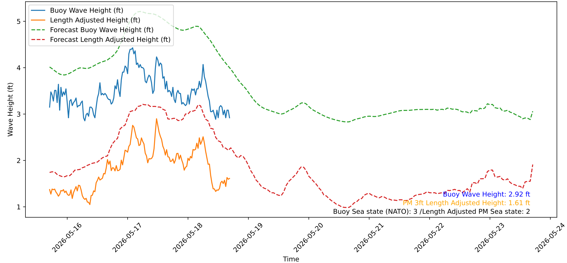
Wave Heights over Time for Green Beach at 2026-05-18 17:11:15
