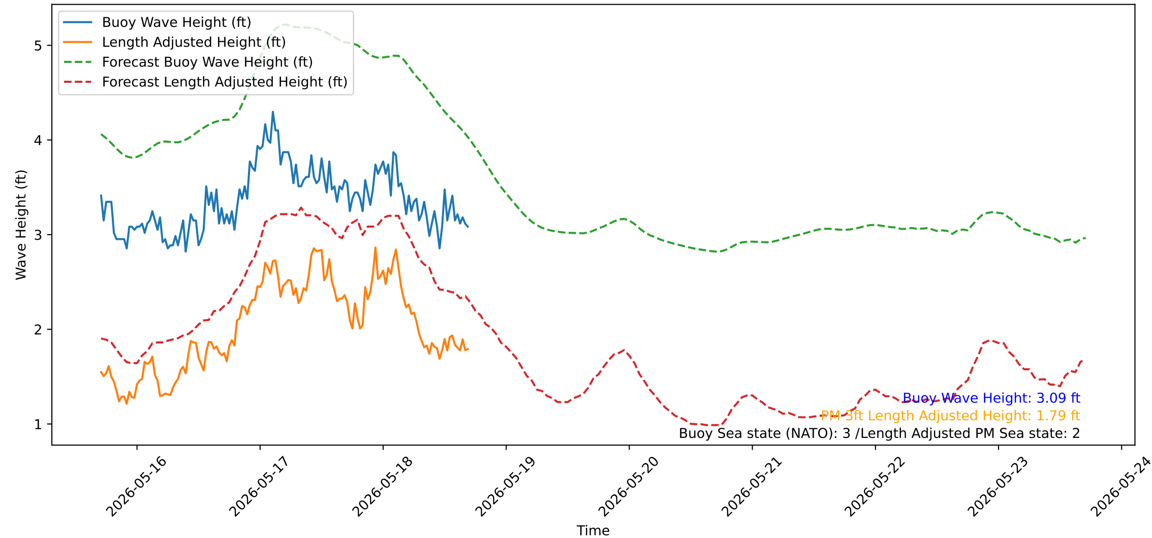
Wave Heights over Time for Oceanside Harbor at 2026-05-18 17:10:32
