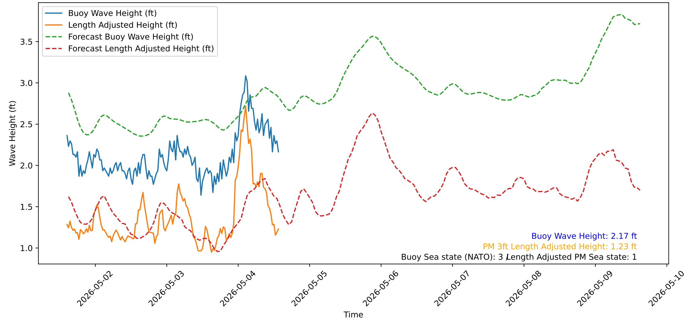
Wave Heights over Time for Oceanside Harbor at 2026-05-04 14:30:31
