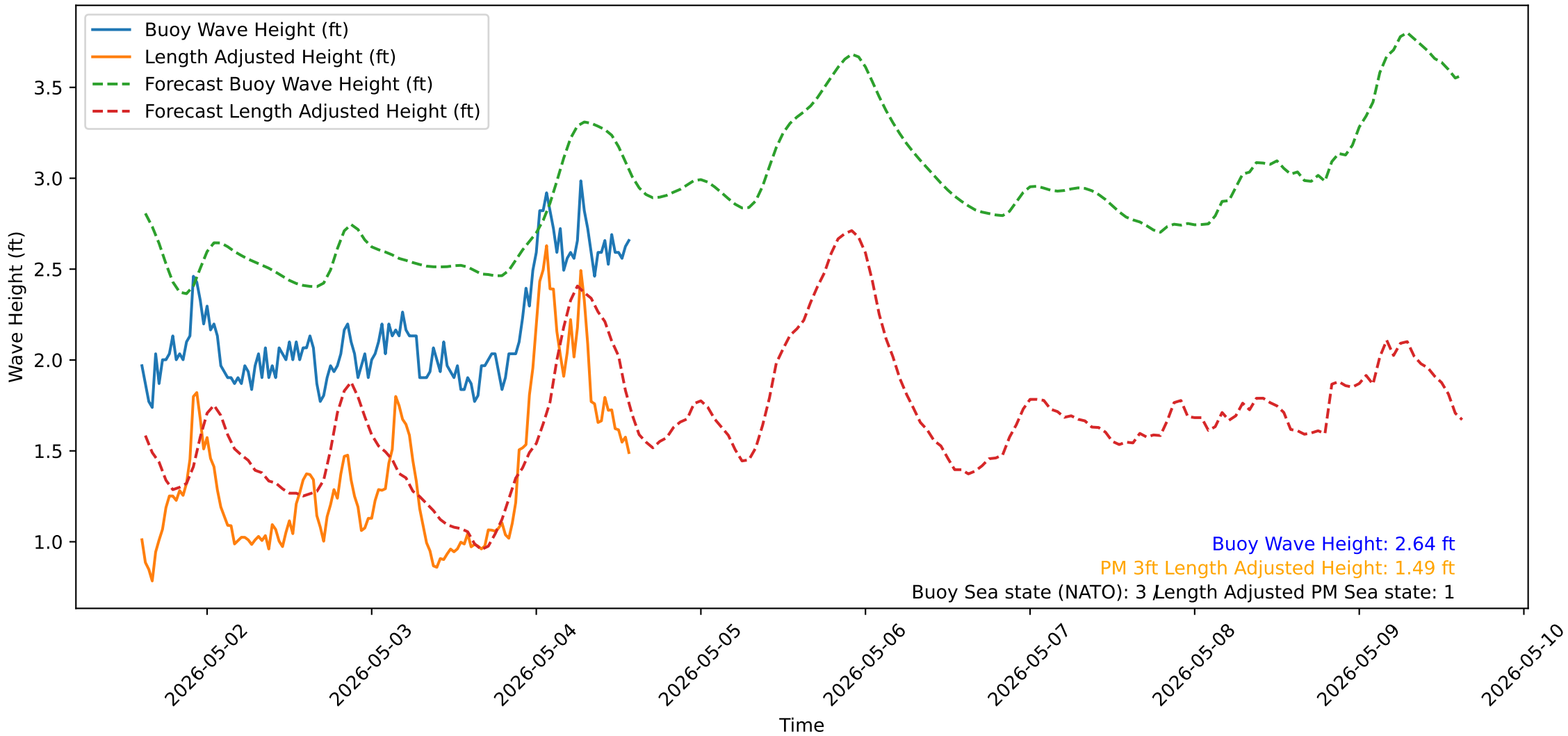
Wave Heights over Time for Green Beach at 2026-05-04 14:31:12
