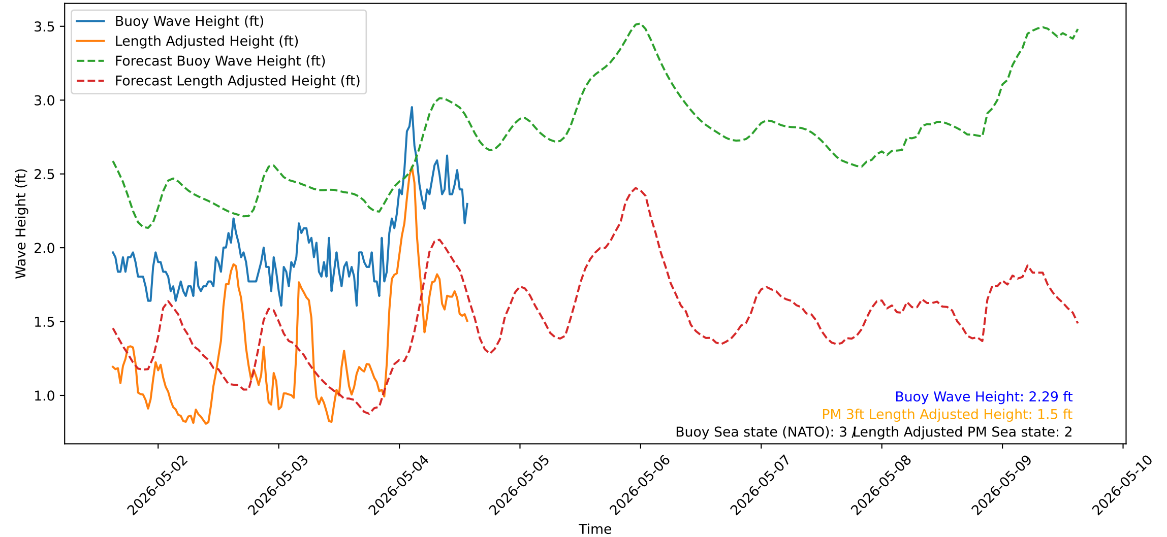
Wave Heights over Time for Red Beach at 2026-05-04 14:30:50
