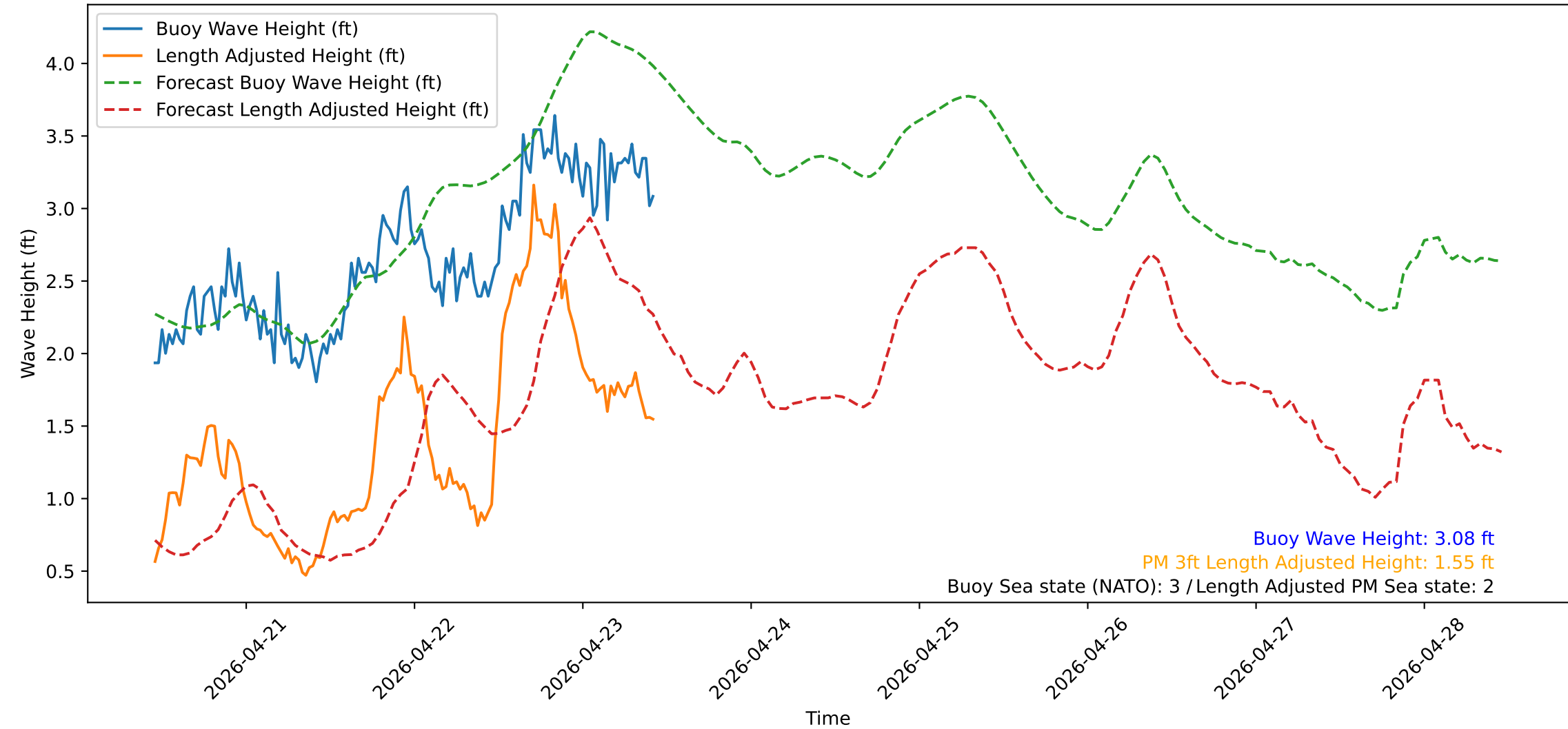
Wave Heights over Time for Red Beach at 2026-04-23 10:50:51
