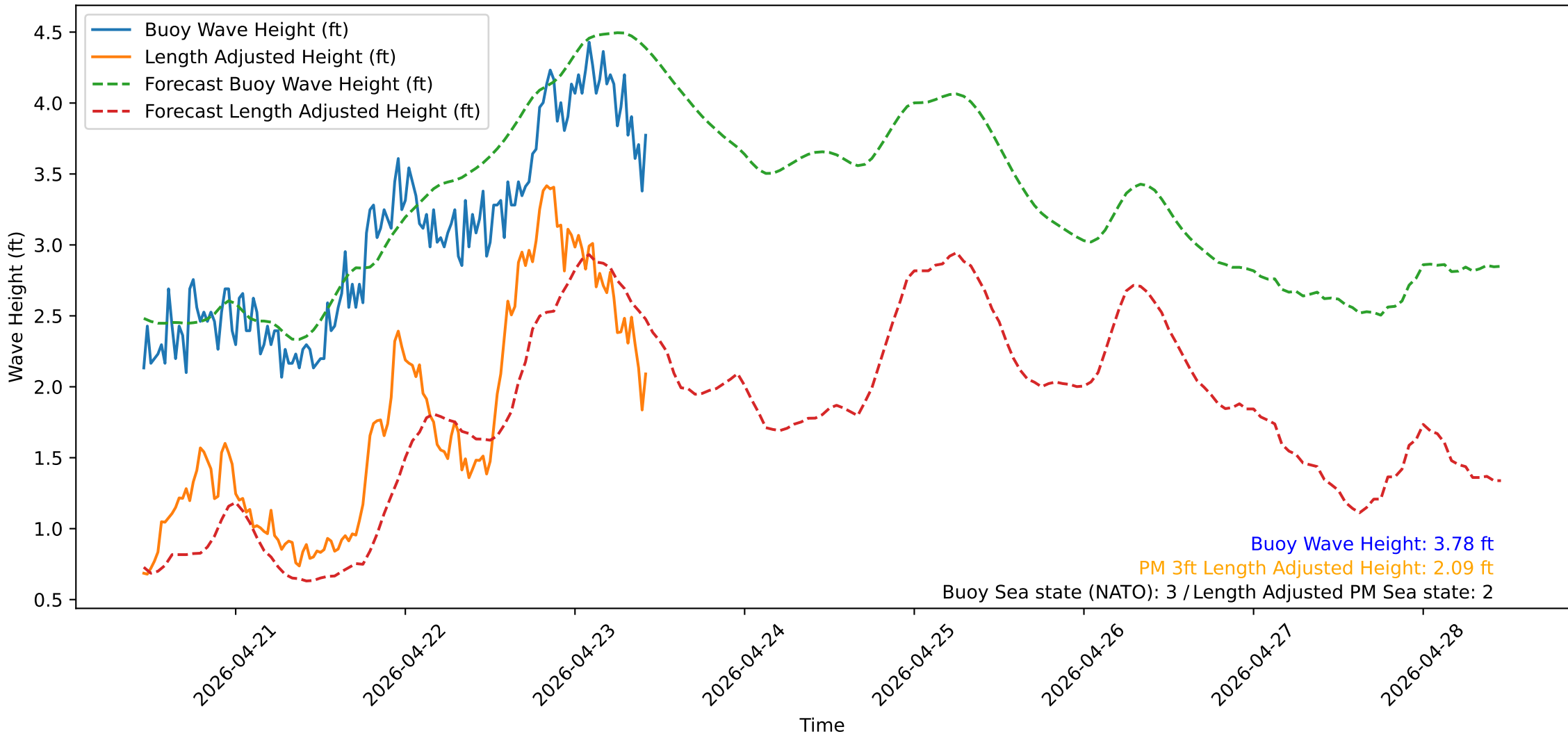
Wave Heights over Time for Oceanside Harbor at 2026-04-23 10:50:31
