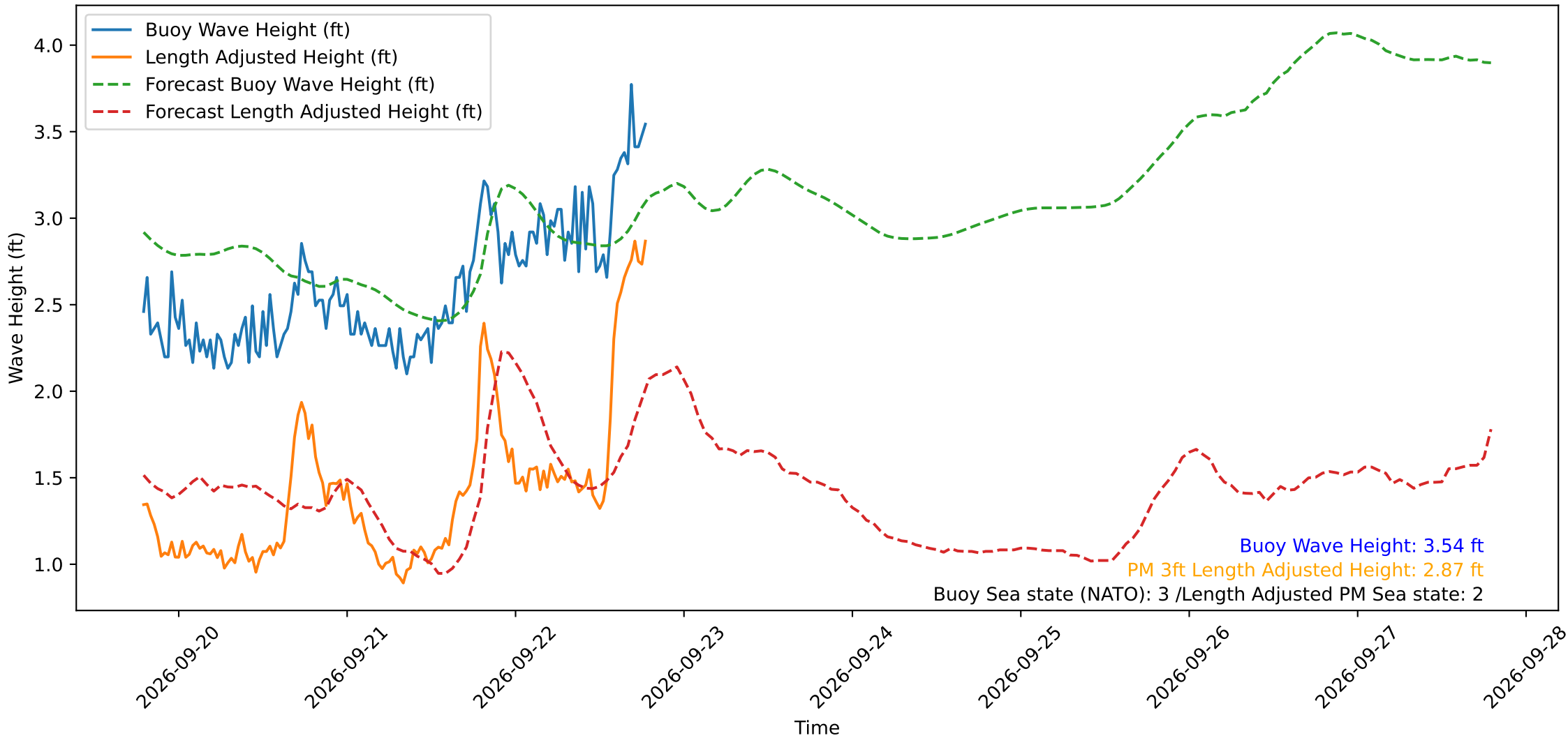
Wave Heights over Time for Oceanside Harbor at 2026-09-22 19:10:30
