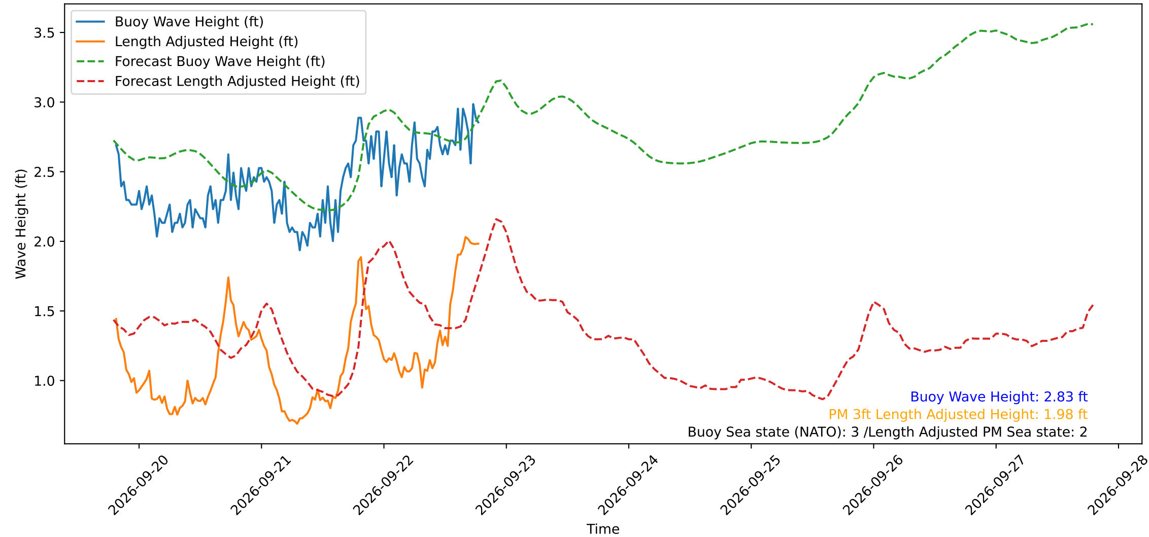
Wave Heights over Time for Red Beach at 2026-09-22 19:10:50
