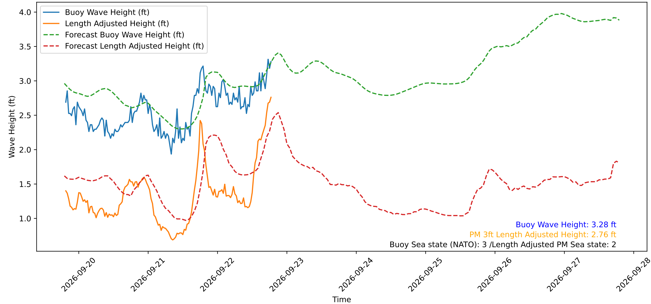
Wave Heights over Time for Green Beach at 2026-09-22 19:11:12
