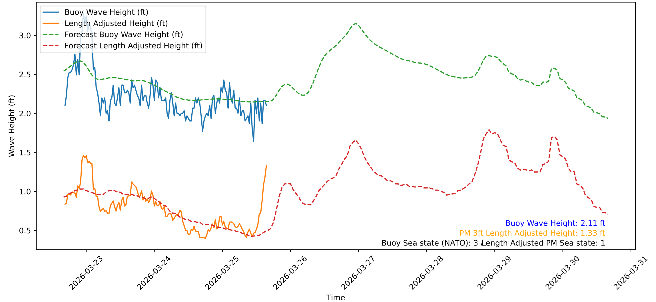
Wave Heights over Time for Green Beach at 2026-03-25 16:21:10
