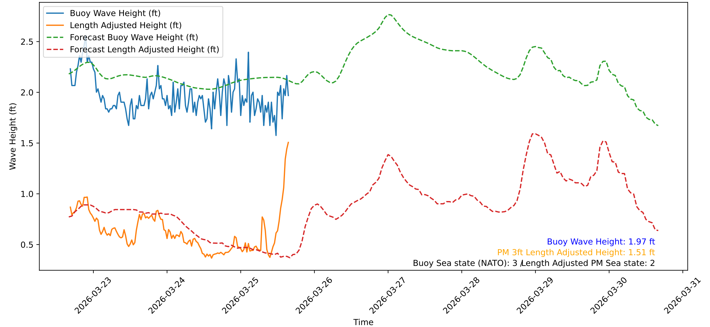
Wave Heights over Time for Red Beach at 2026-03-25 16:20:48
