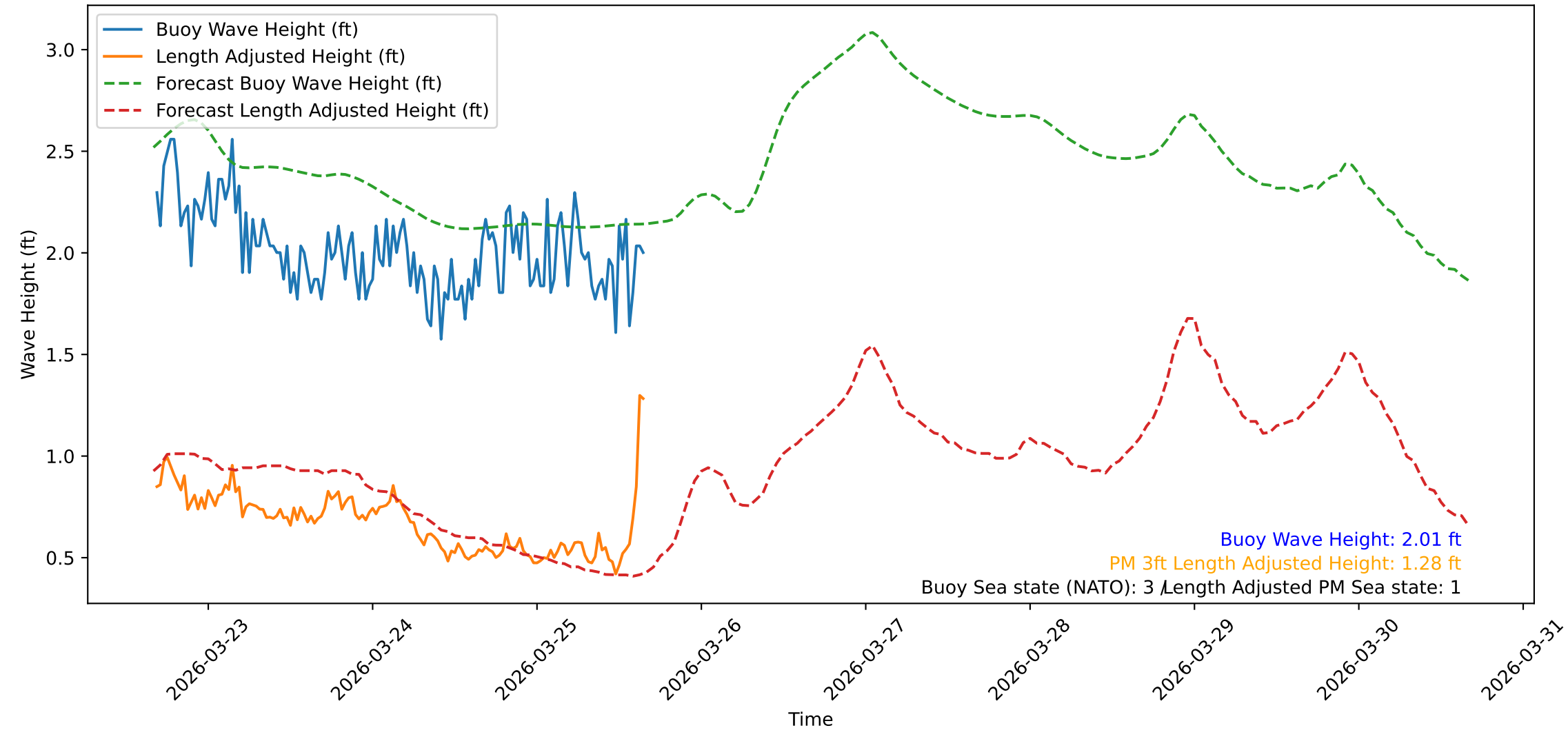
Wave Heights over Time for Oceanside Harbor at 2026-03-25 16:20:32
