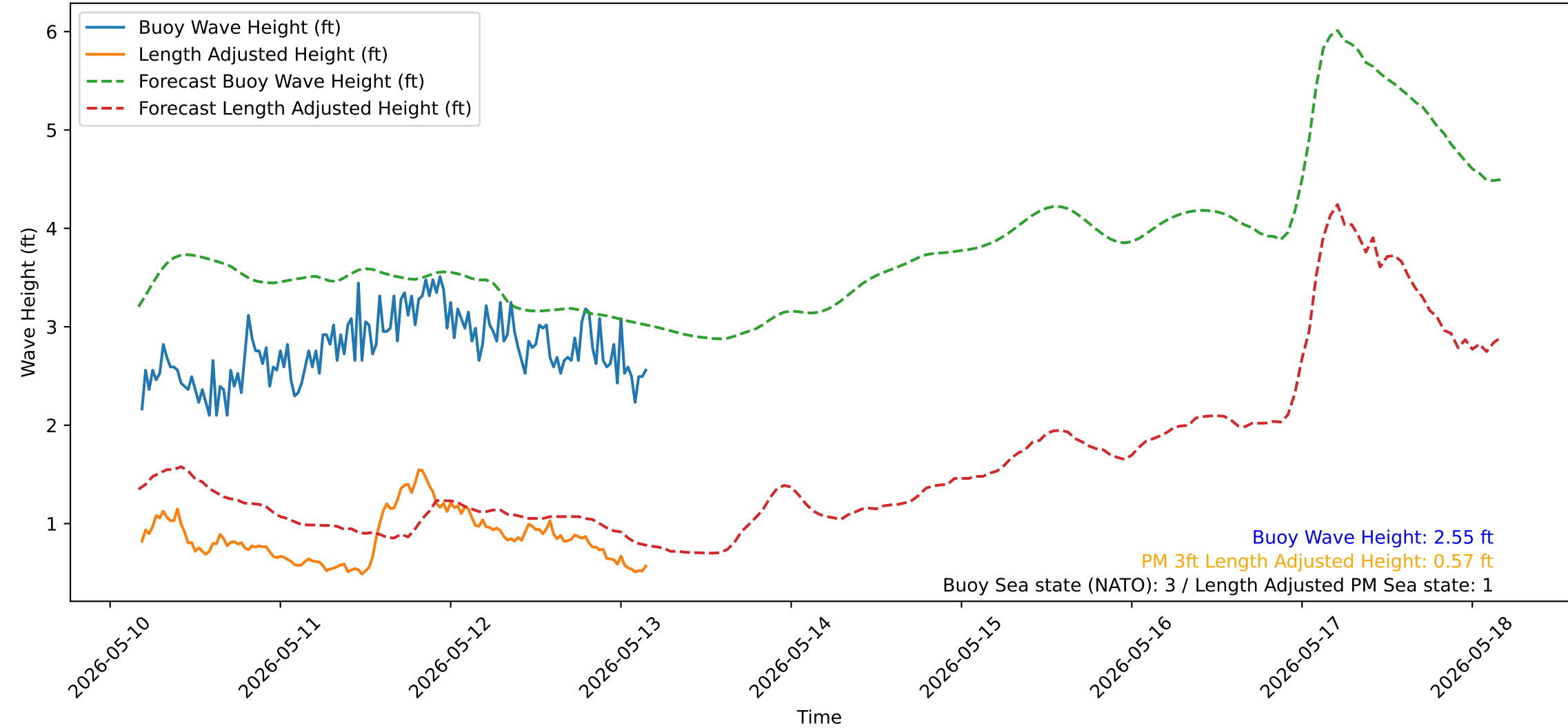
Wave Heights over Time for Green Beach at 2026-05-13 04:21:14
