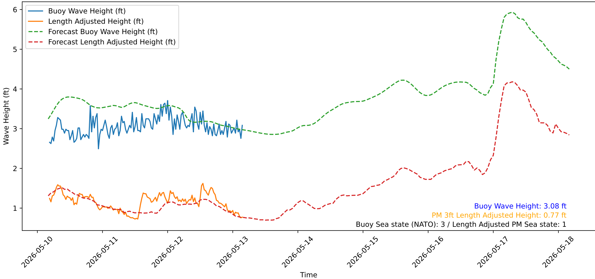
Wave Heights over Time for Oceanside Harbor at 2026-05-13 04:20:31
