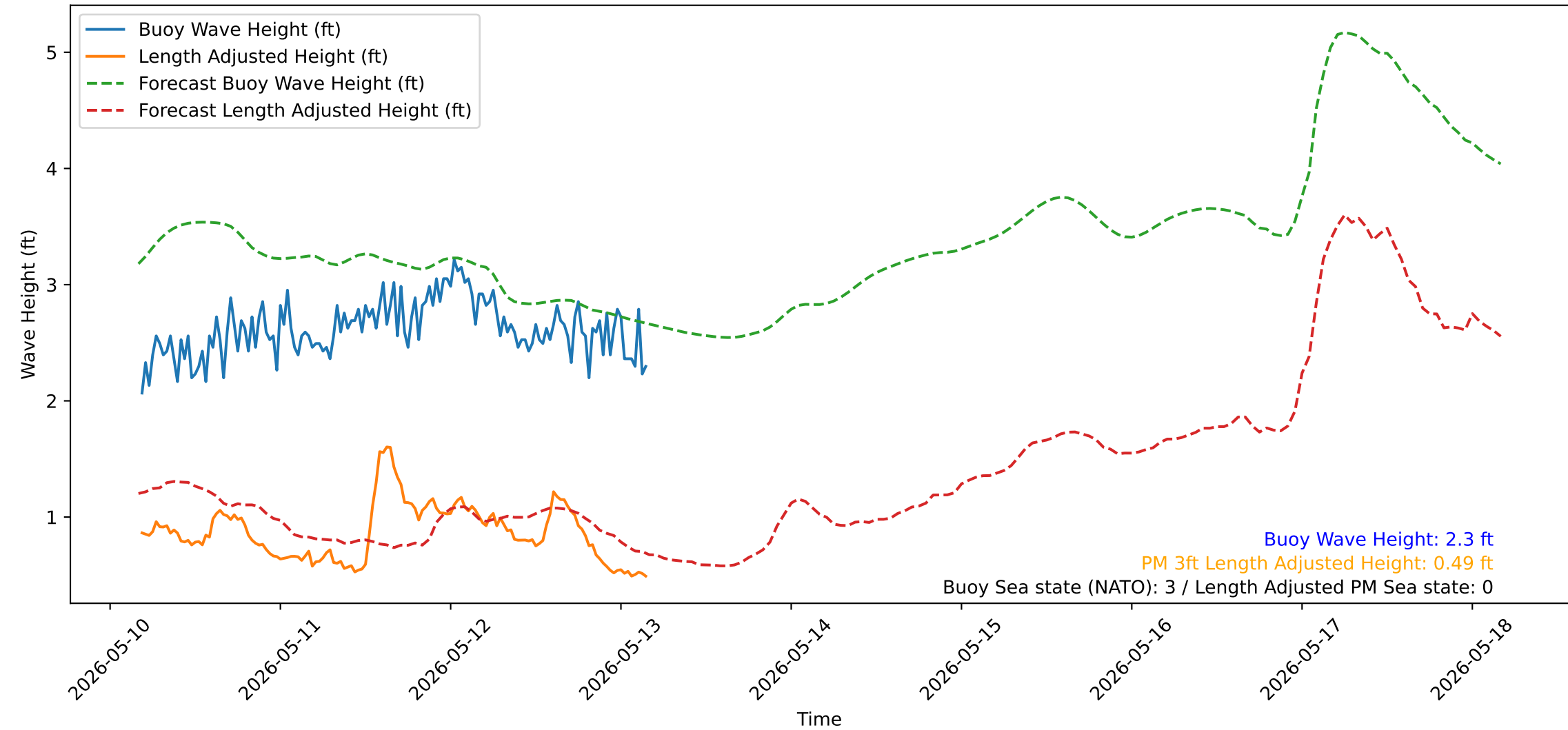
Wave Heights over Time for Red Beach at 2026-05-13 04:20:51
