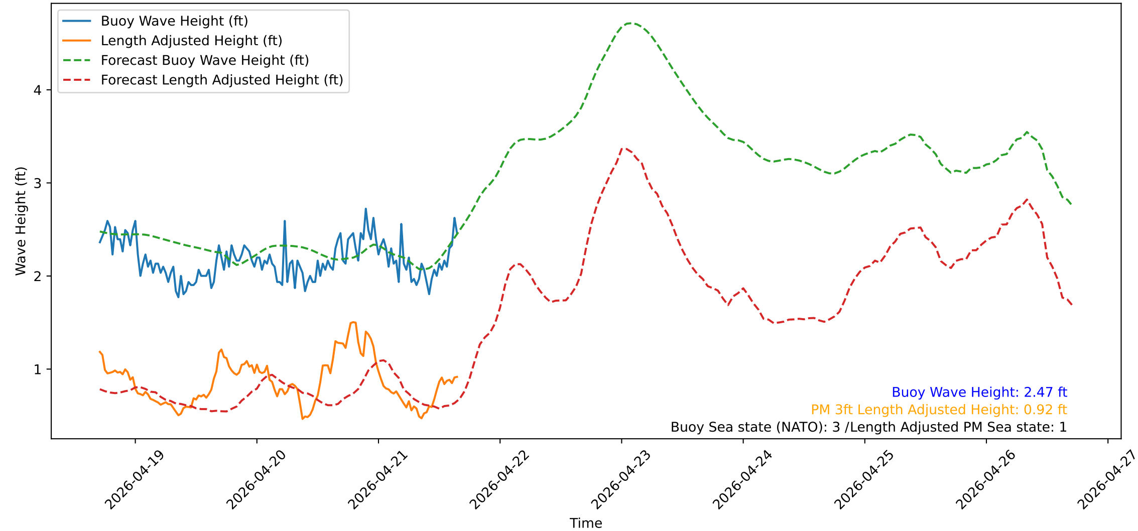
Wave Heights over Time for Red Beach at 2026-04-21 16:50:52
