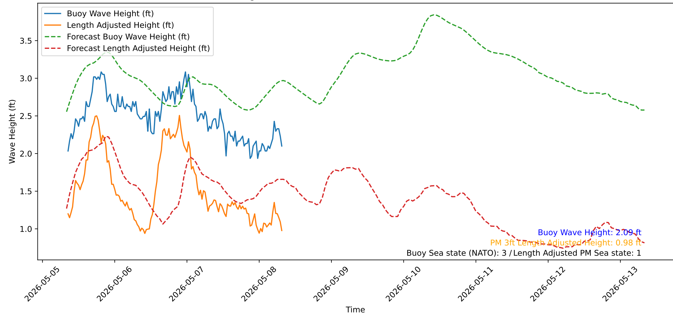
Wave Heights over Time for Red Beach at 2026-05-08 08:20:53
