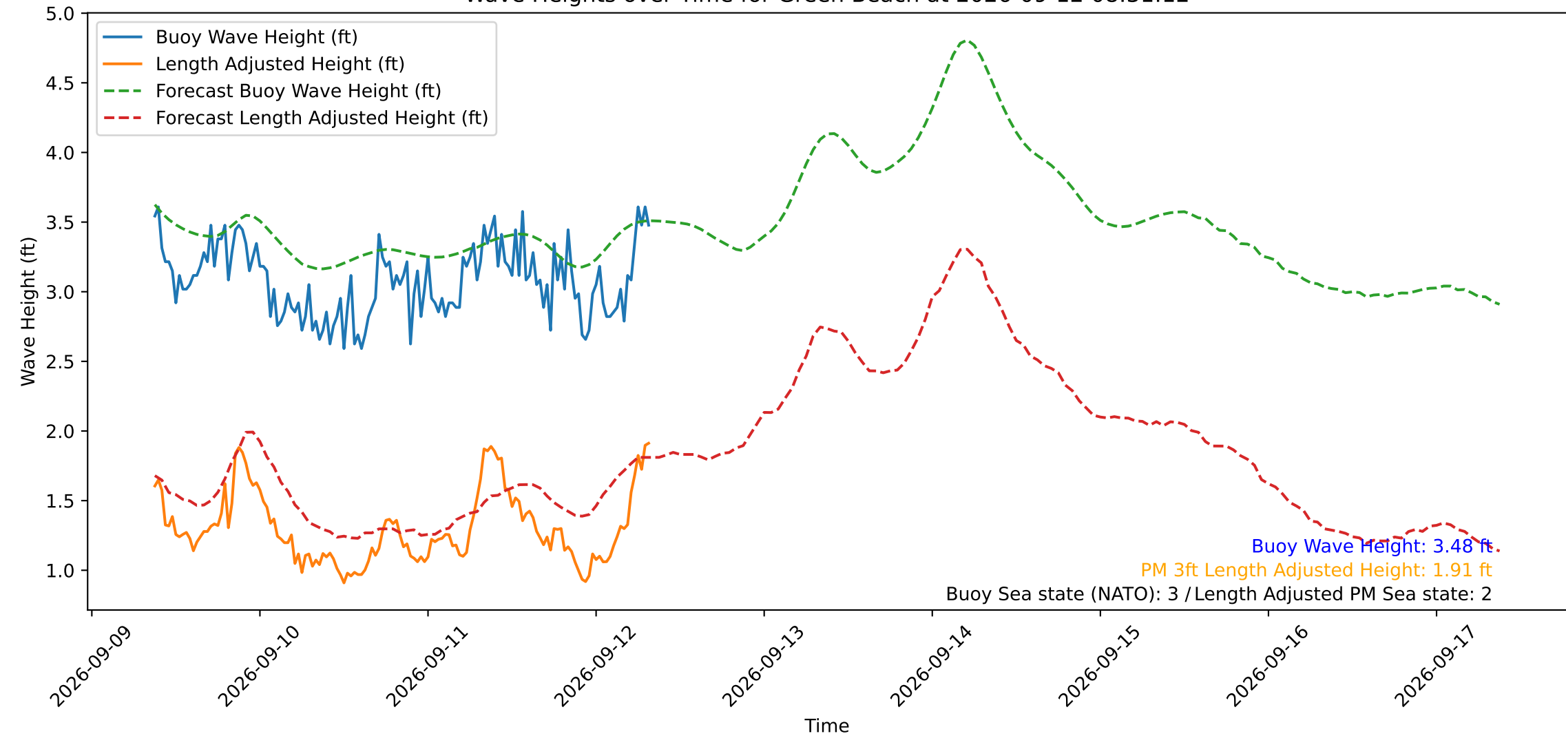
Wave Heights over Time for Green Beach at 2026-09-12 08:31:12
