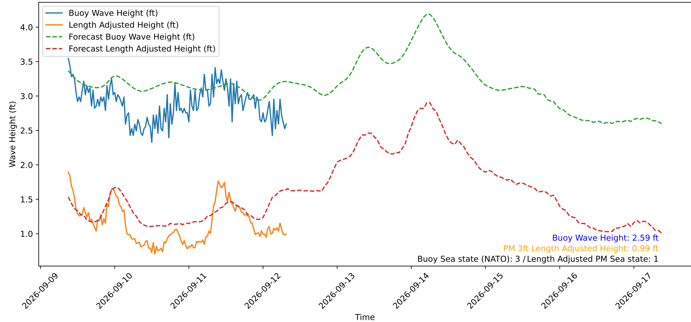
Wave Heights over Time for Red Beach at 2026-09-12 08:30:49
