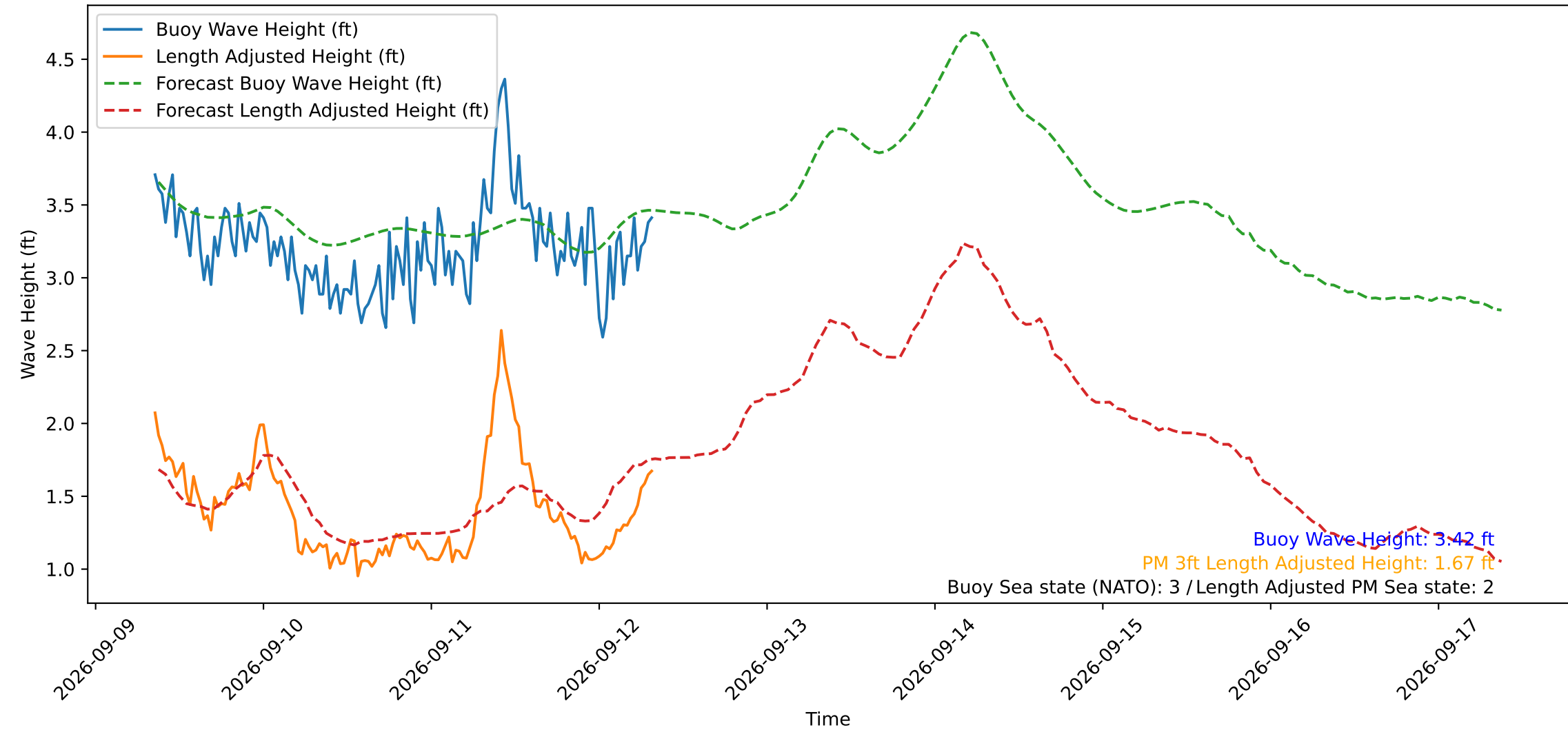
Wave Heights over Time for Oceanside Harbor at 2026-09-12 08:30:30
