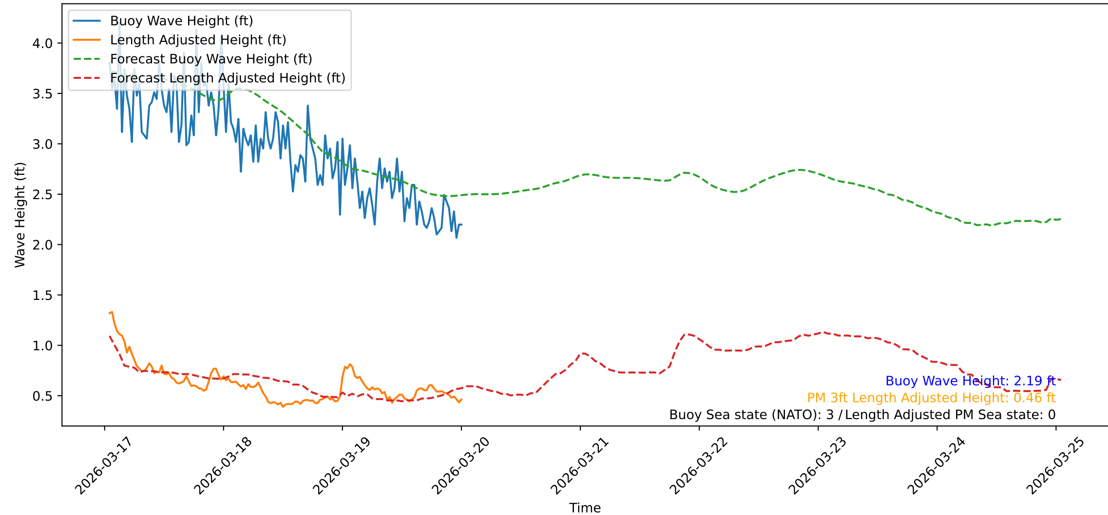
Wave Heights over Time for Green Beach at 2026-03-20 01:01:10
