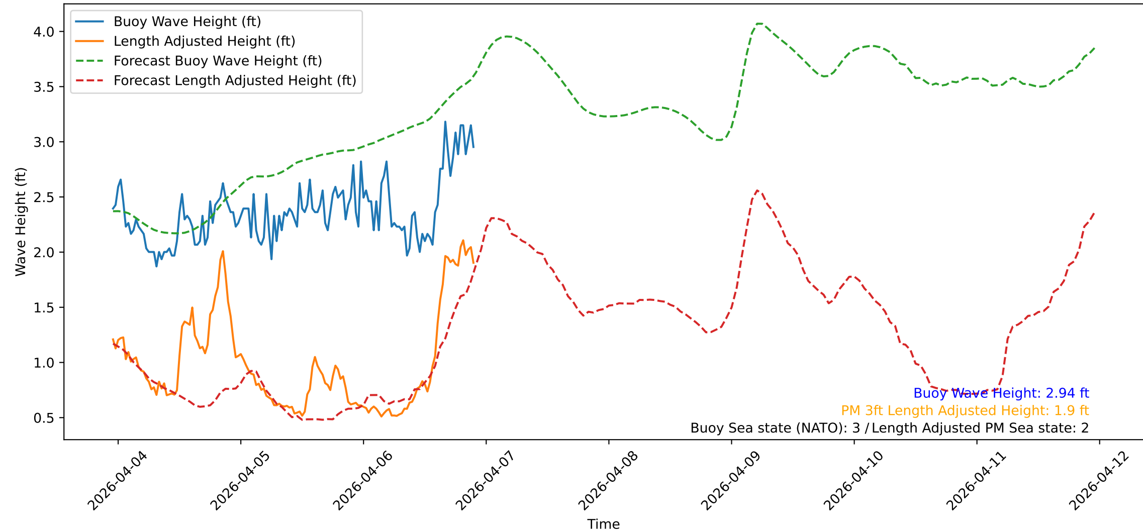
Wave Heights over Time for Red Beach at 2026-04-06 22:50:47
