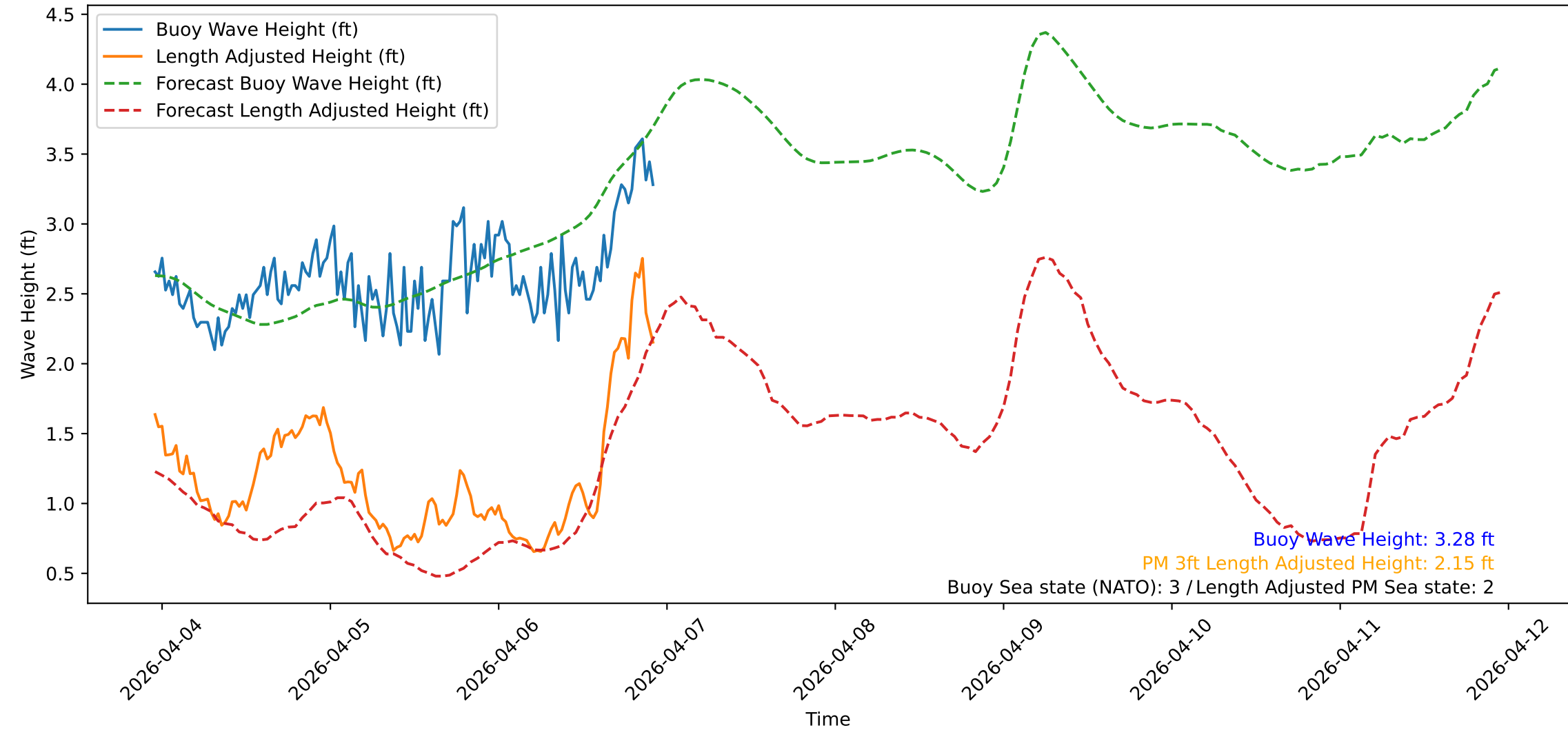
Wave Heights over Time for Oceanside Harbor at 2026-04-06 22:50:30
