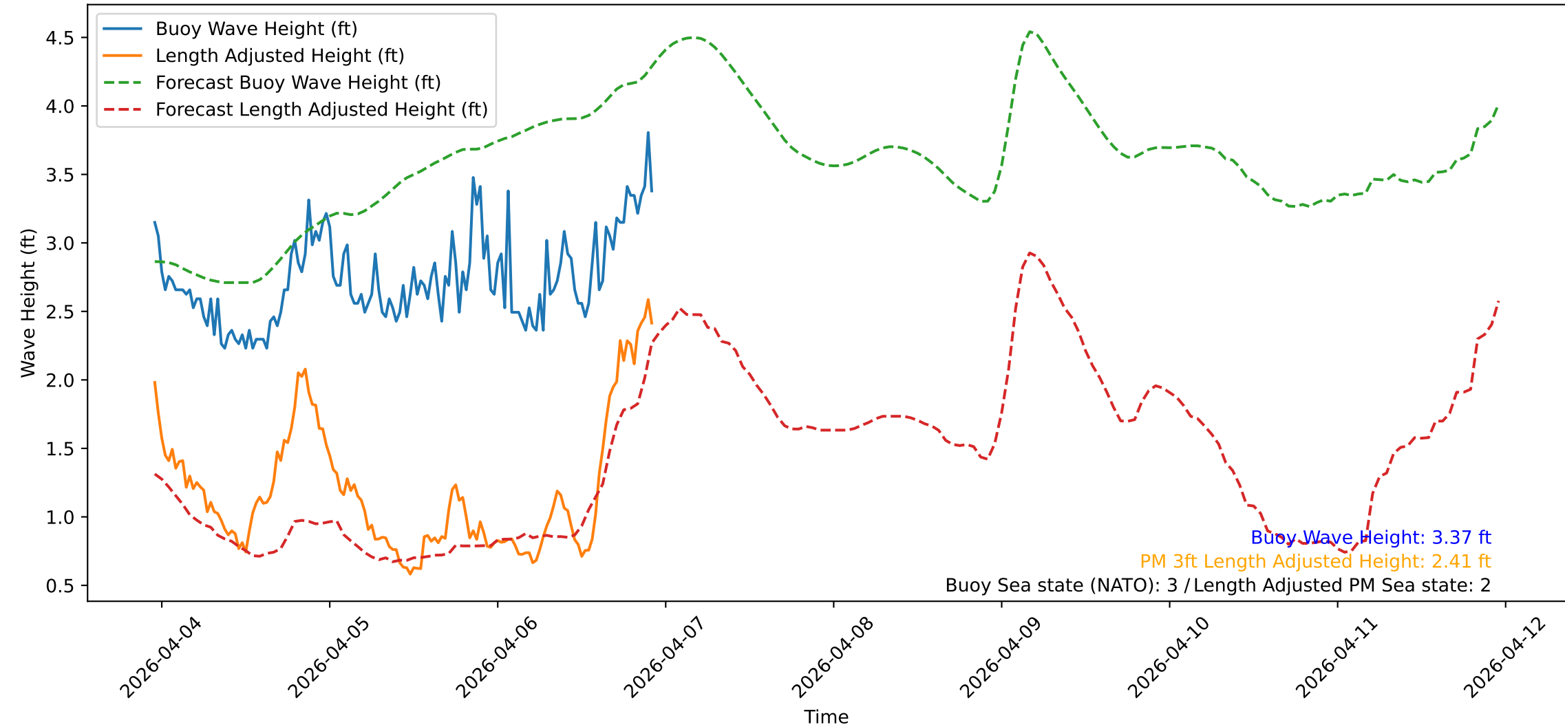
Wave Heights over Time for Green Beach at 2026-04-06 22:51:09
