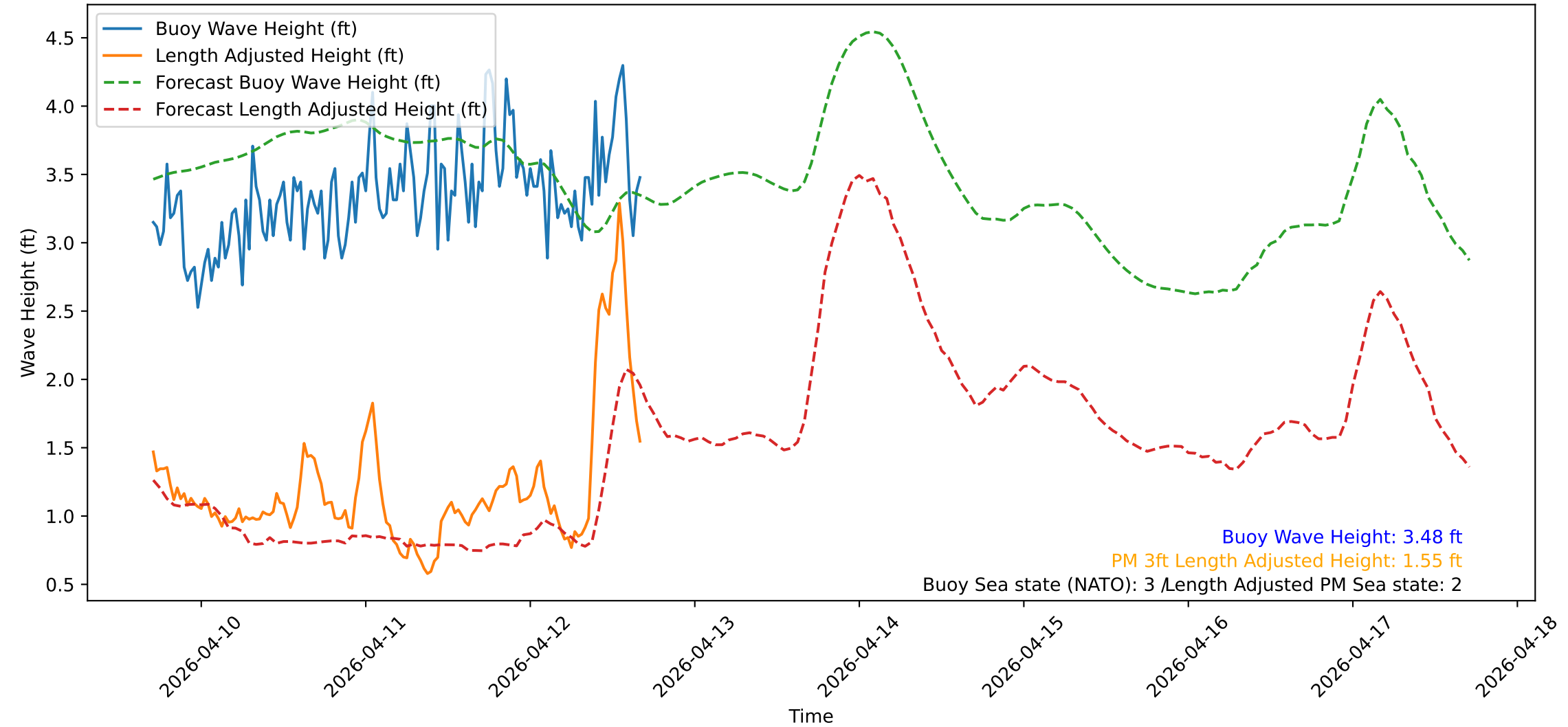
Wave Heights over Time for Red Beach at 2026-04-12 16:50:51
