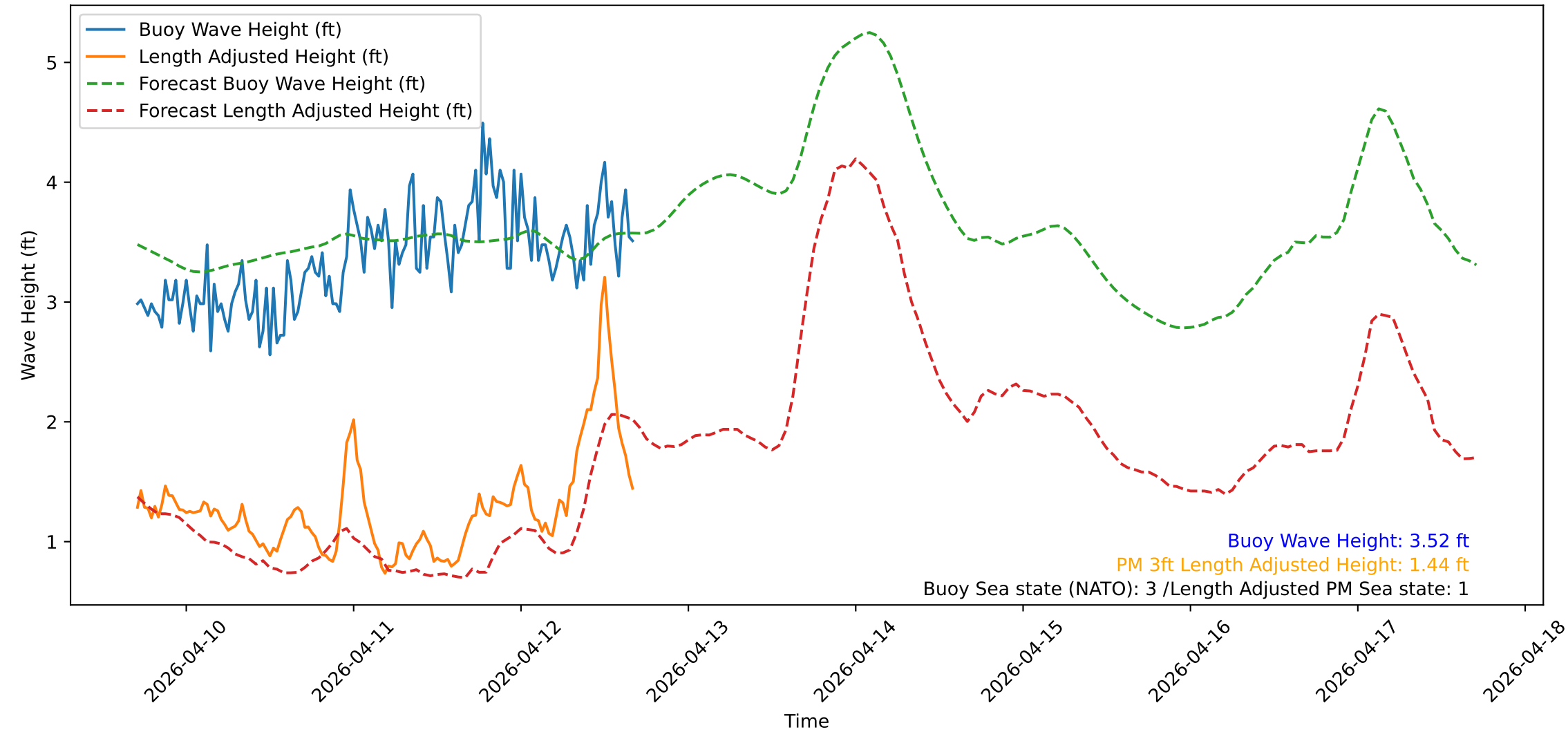
Wave Heights over Time for Green Beach at 2026-04-12 16:51:13
