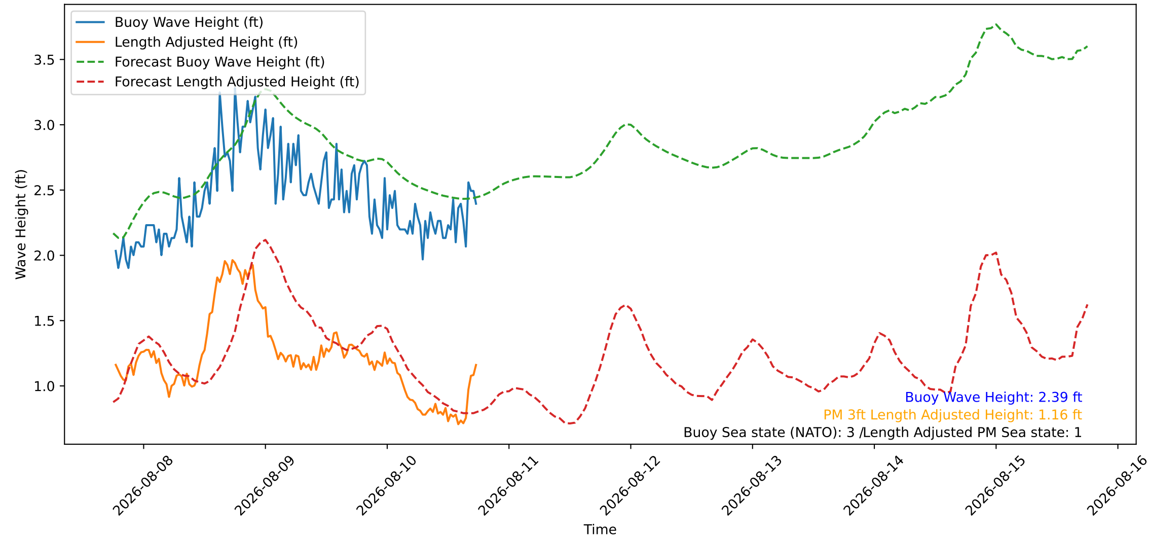
Wave Heights over Time for Oceanside Harbor at 2026-08-10 18:20:26
