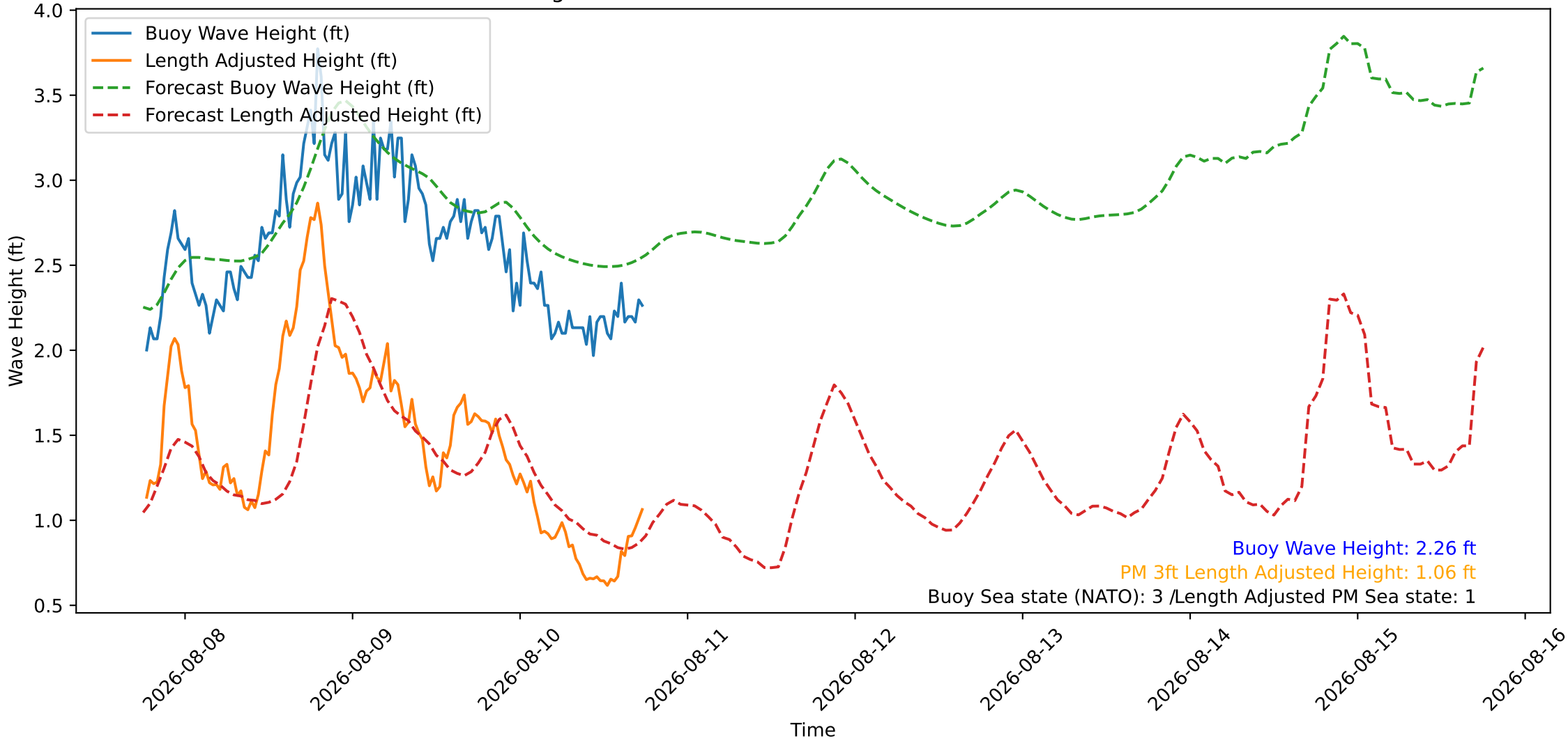
Wave Heights over Time for Green Beach at 2026-08-10 18:21:10
