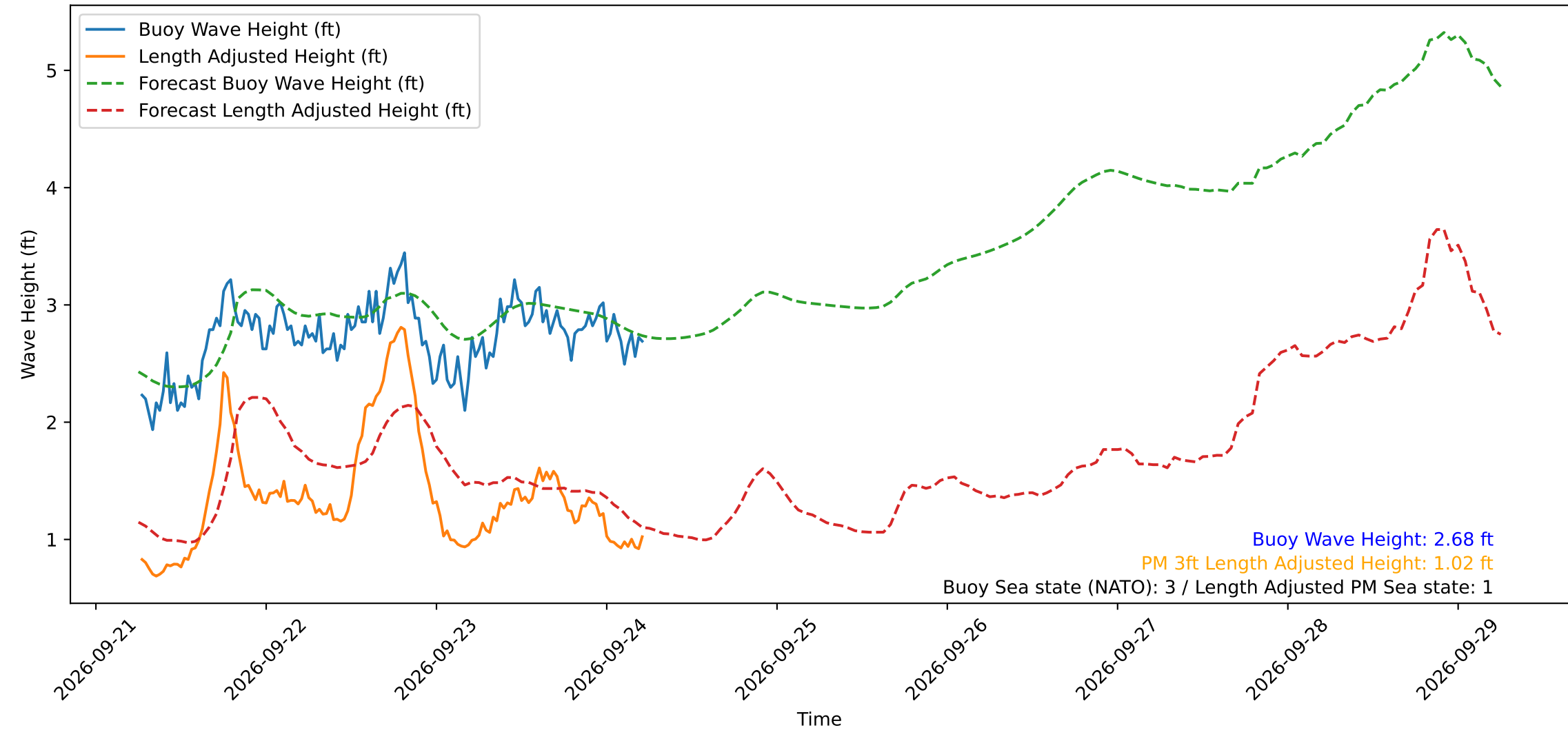
Wave Heights over Time for Green Beach at 2026-09-24 06:01:13
