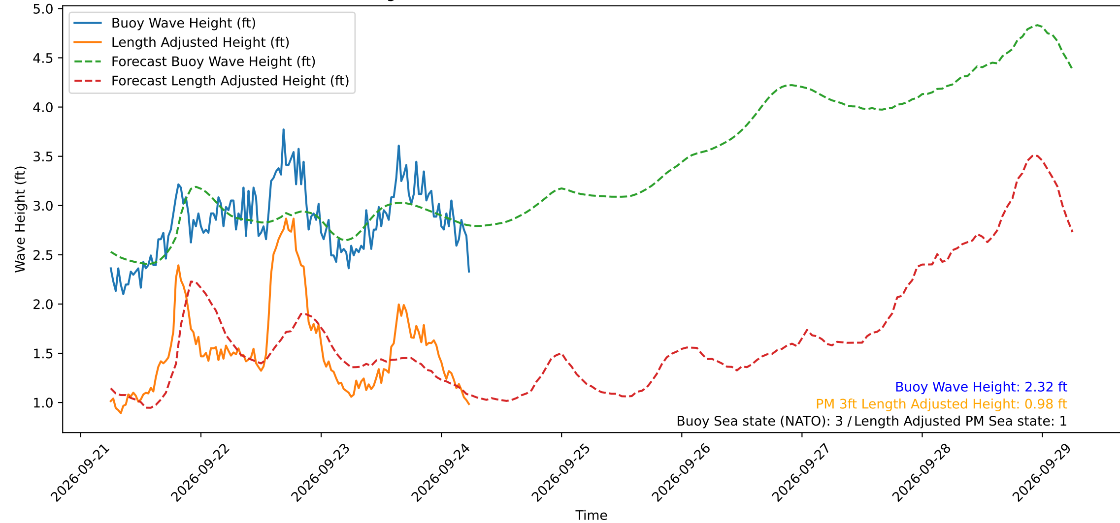
Wave Heights over Time for Oceanside Harbor at 2026-09-24 06:00:30
