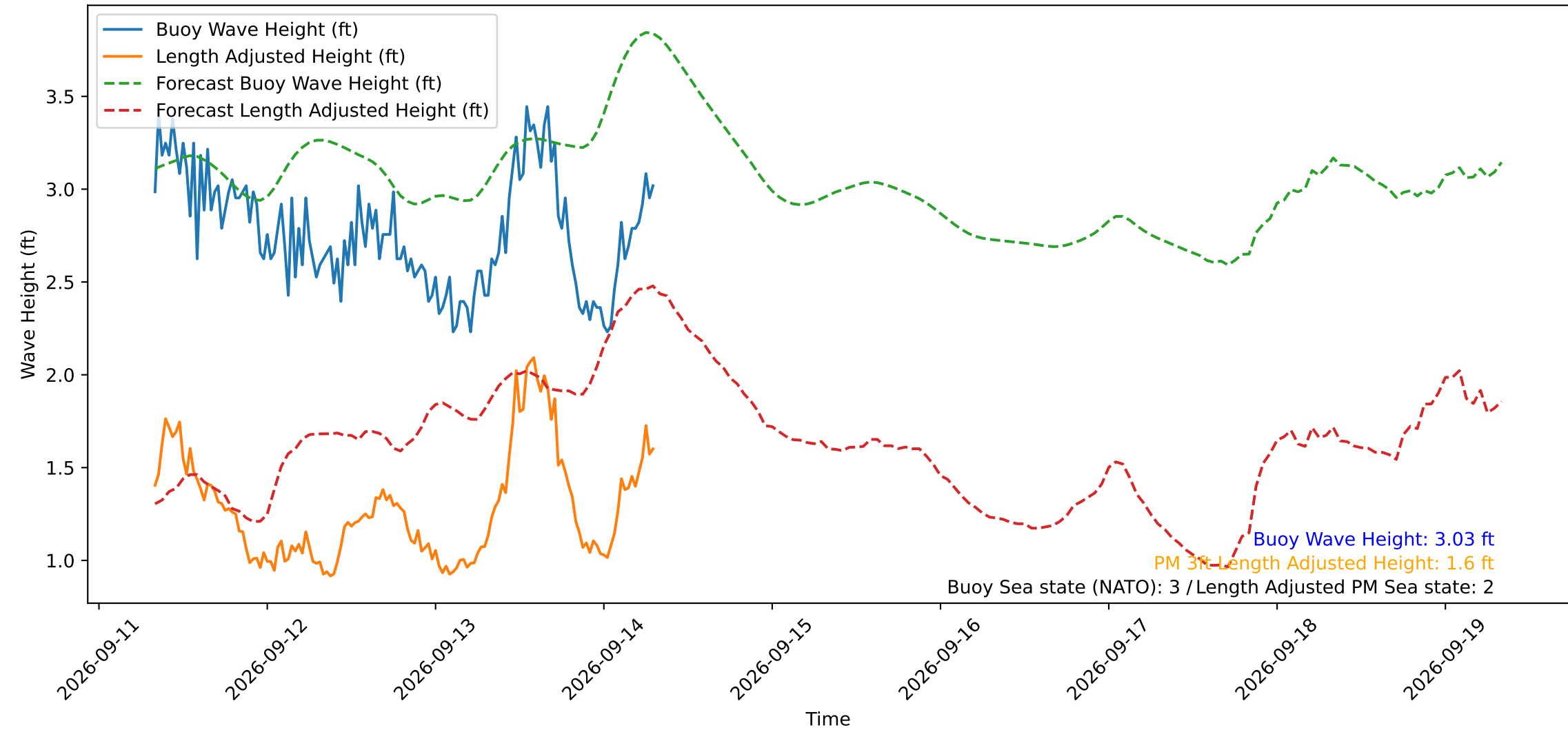
Wave Heights over Time for Red Beach at 2026-09-14 07:40:49
