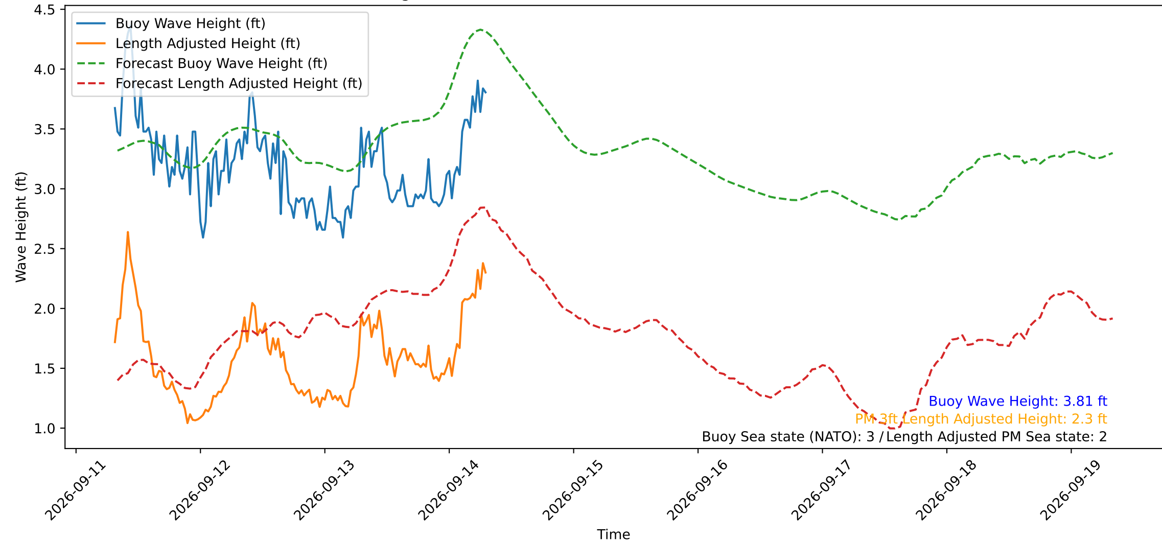
Wave Heights over Time for Oceanside Harbor at 2026-09-14 07:40:29
