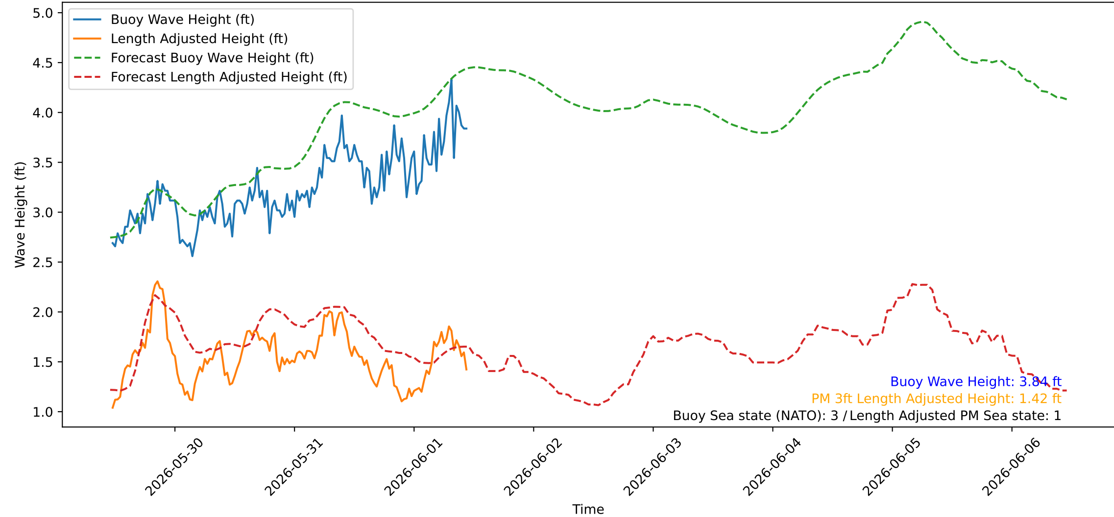
Wave Heights over Time for Green Beach at 2026-06-01 11:21:08
