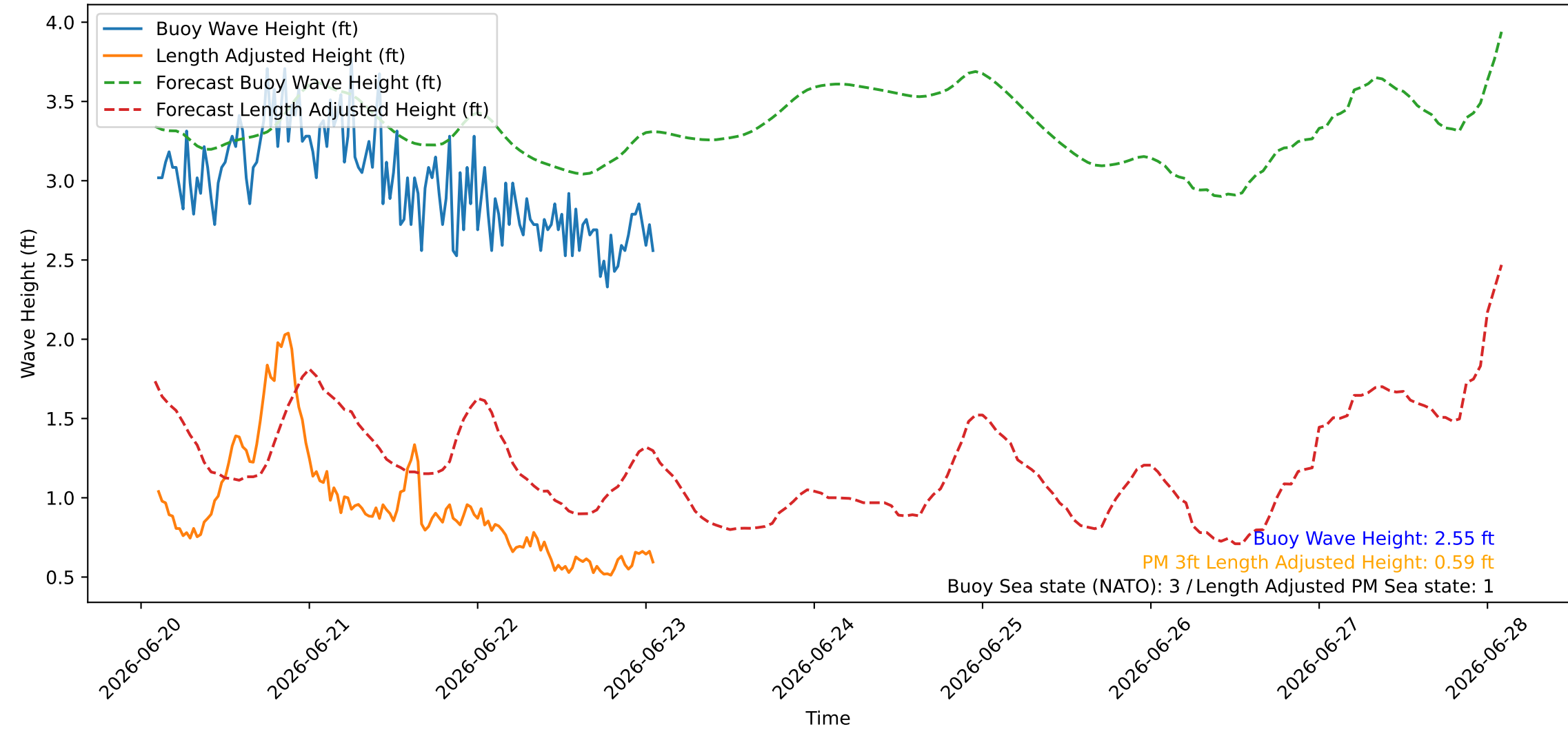
Wave Heights over Time for Red Beach at 2026-06-23 02:00:45
