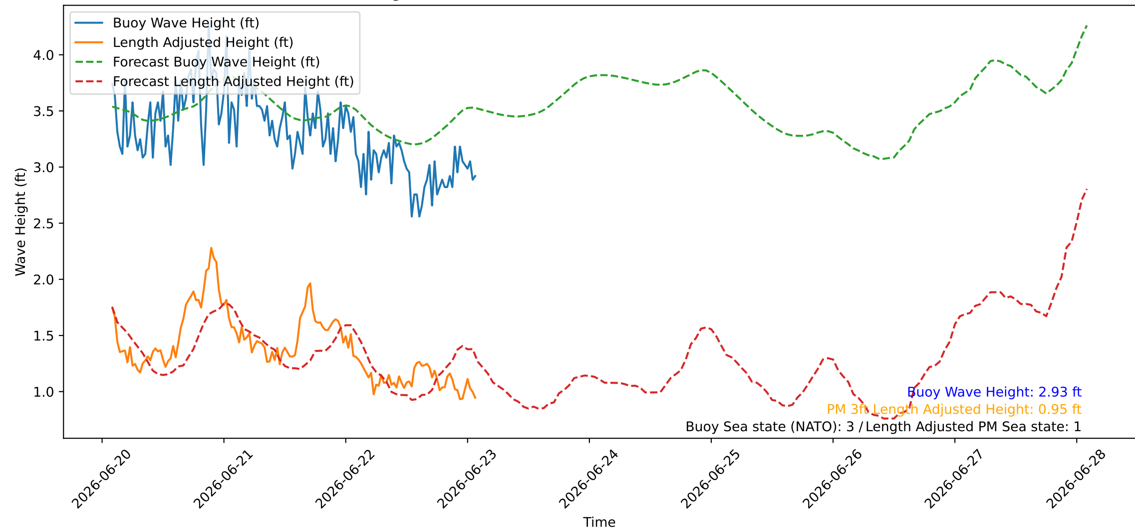
Wave Heights over Time for Oceanside Harbor at 2026-06-23 02:00:26
