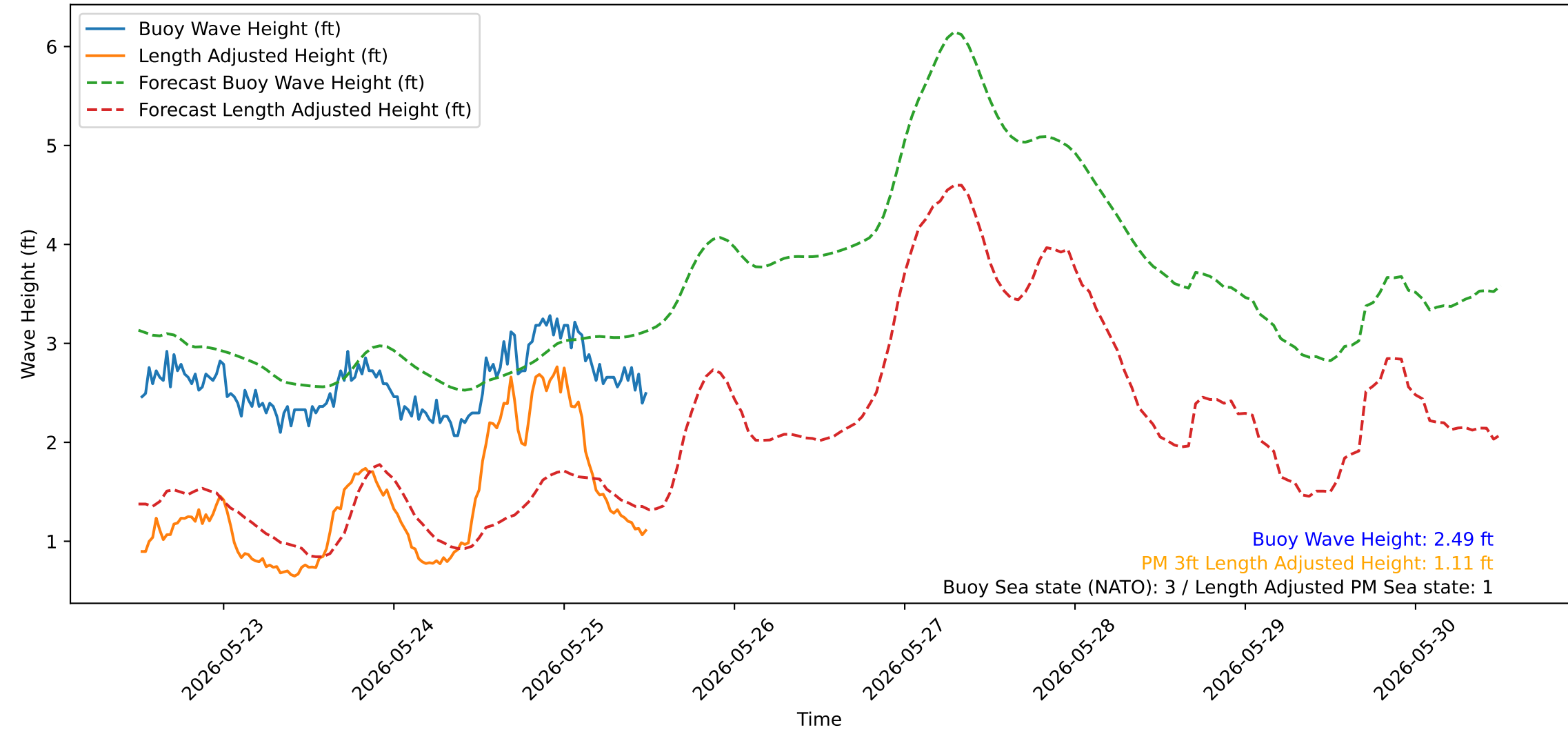
Wave Heights over Time for Green Beach at 2026-05-25 12:21:14
