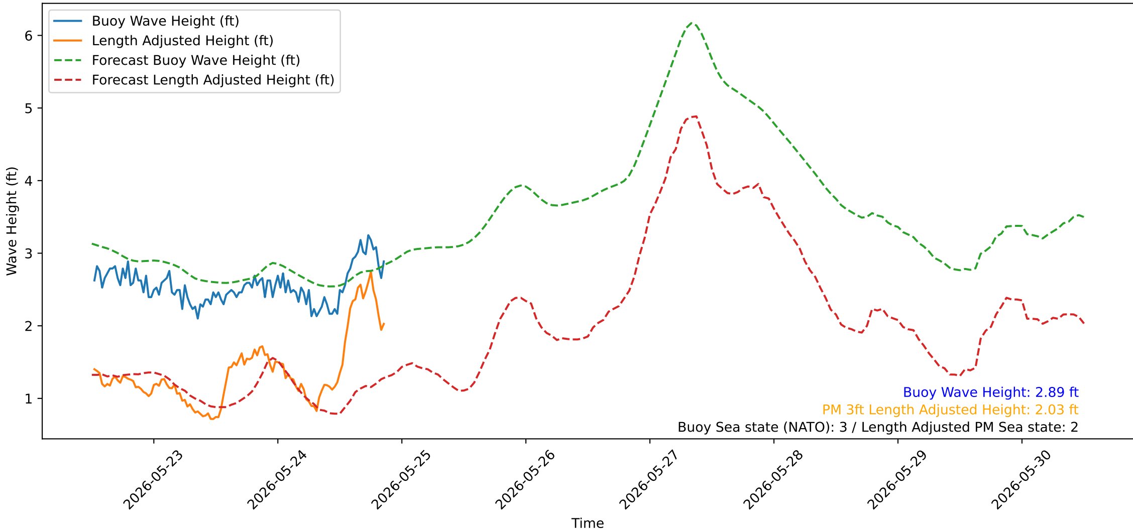
Wave Heights over Time for Oceanside Harbor at 2026-05-25 12:20:30
