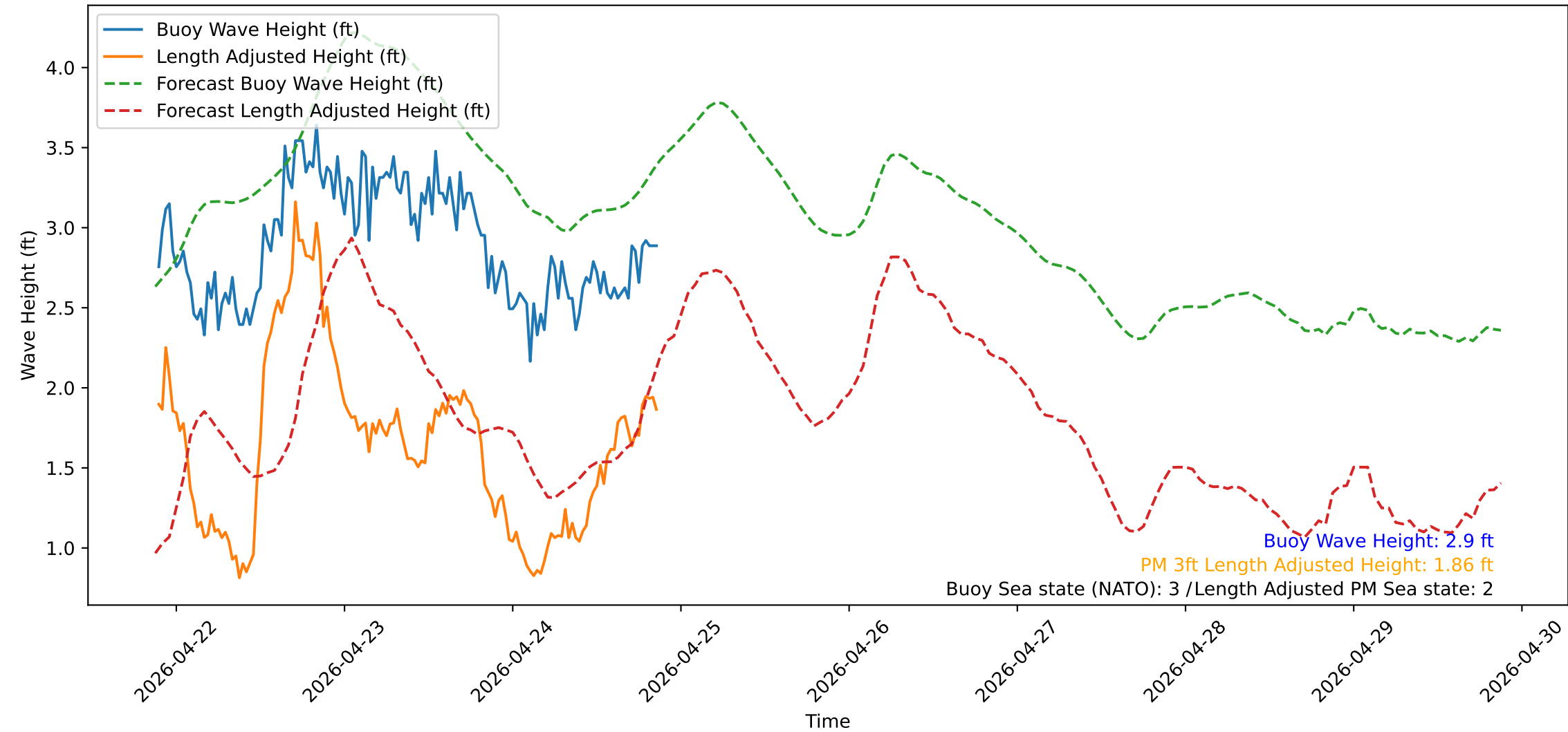
Wave Heights over Time for Red Beach at 2026-04-24 21:20:52
