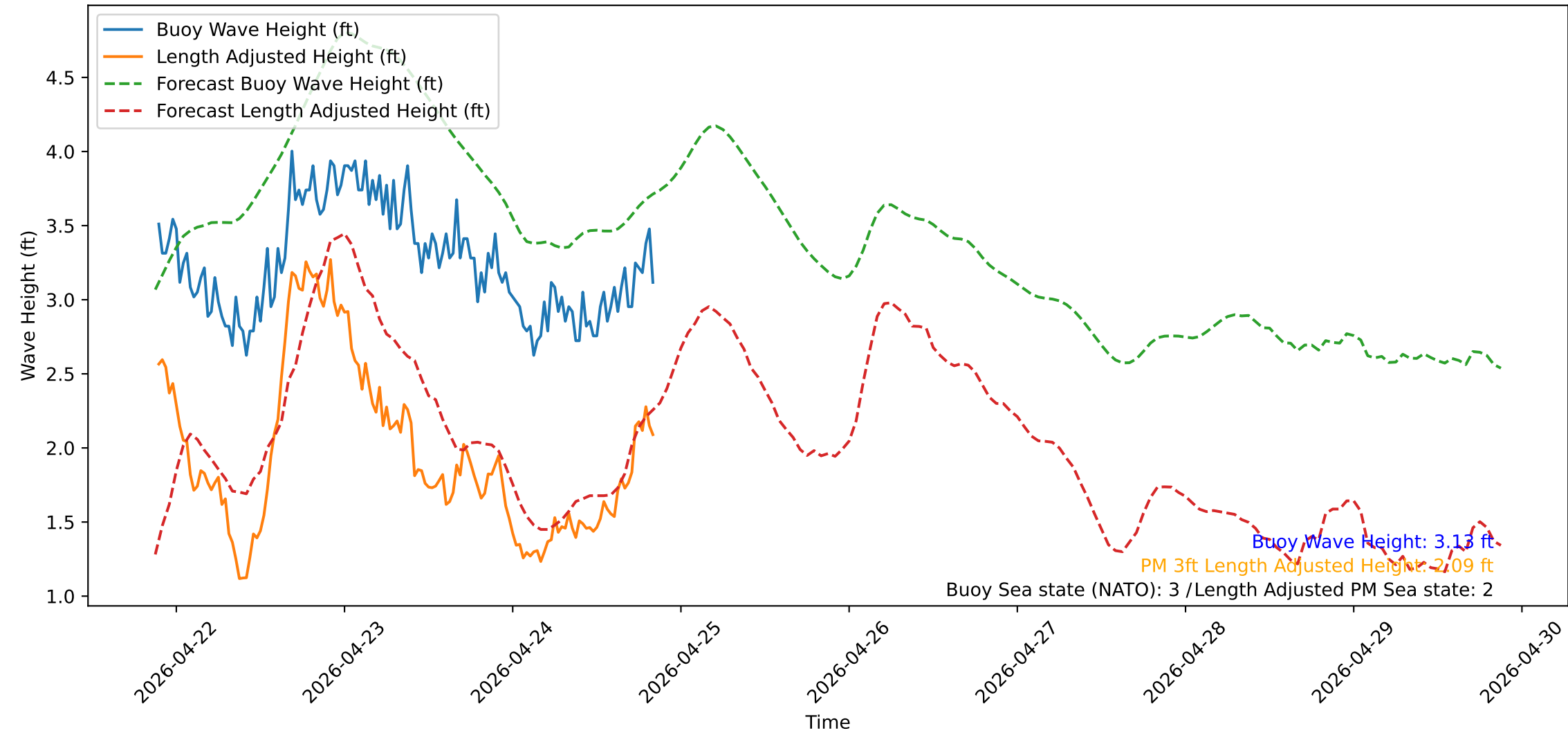
Wave Heights over Time for Green Beach at 2026-04-24 21:21:14
