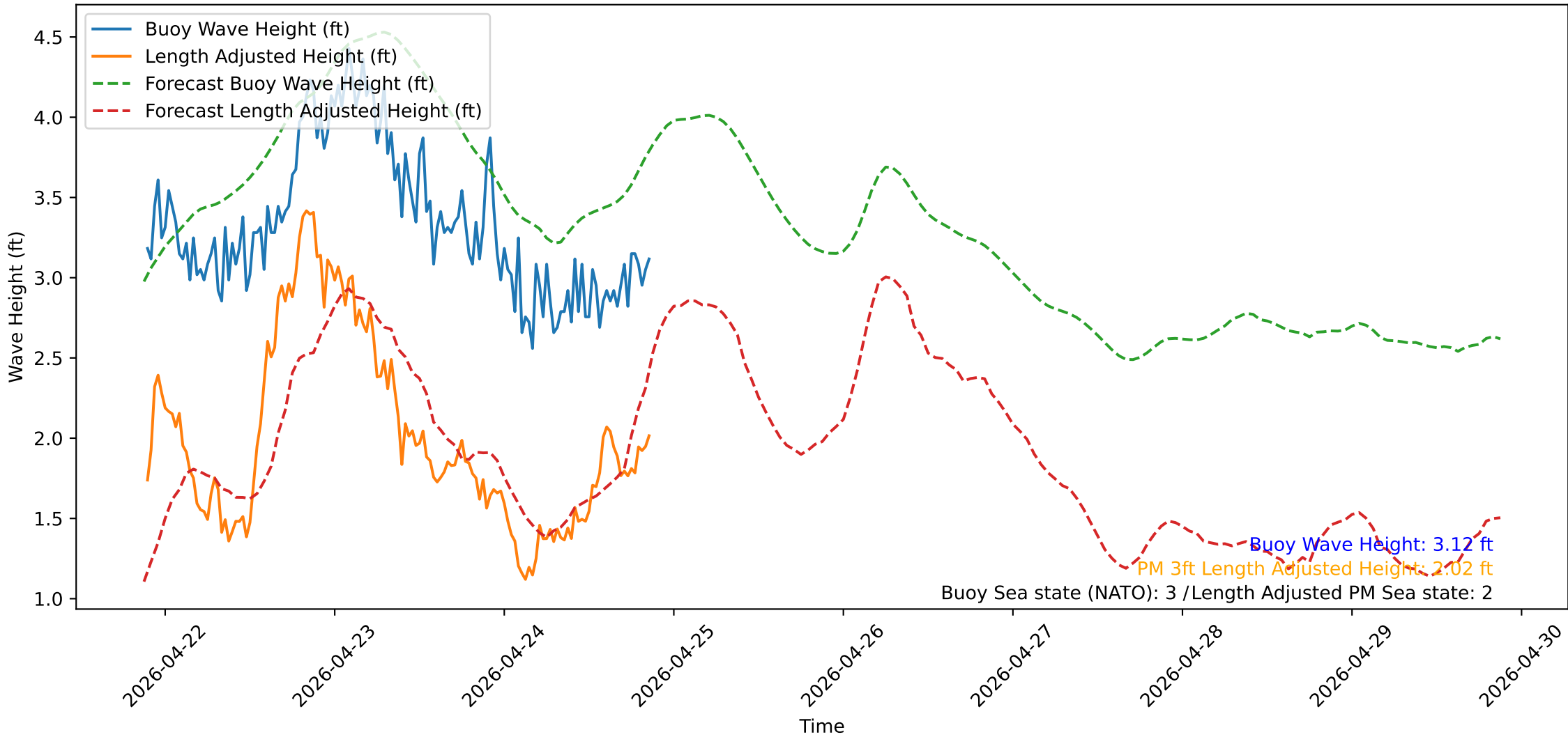
Wave Heights over Time for Oceanside Harbor at 2026-04-24 21:20:32
