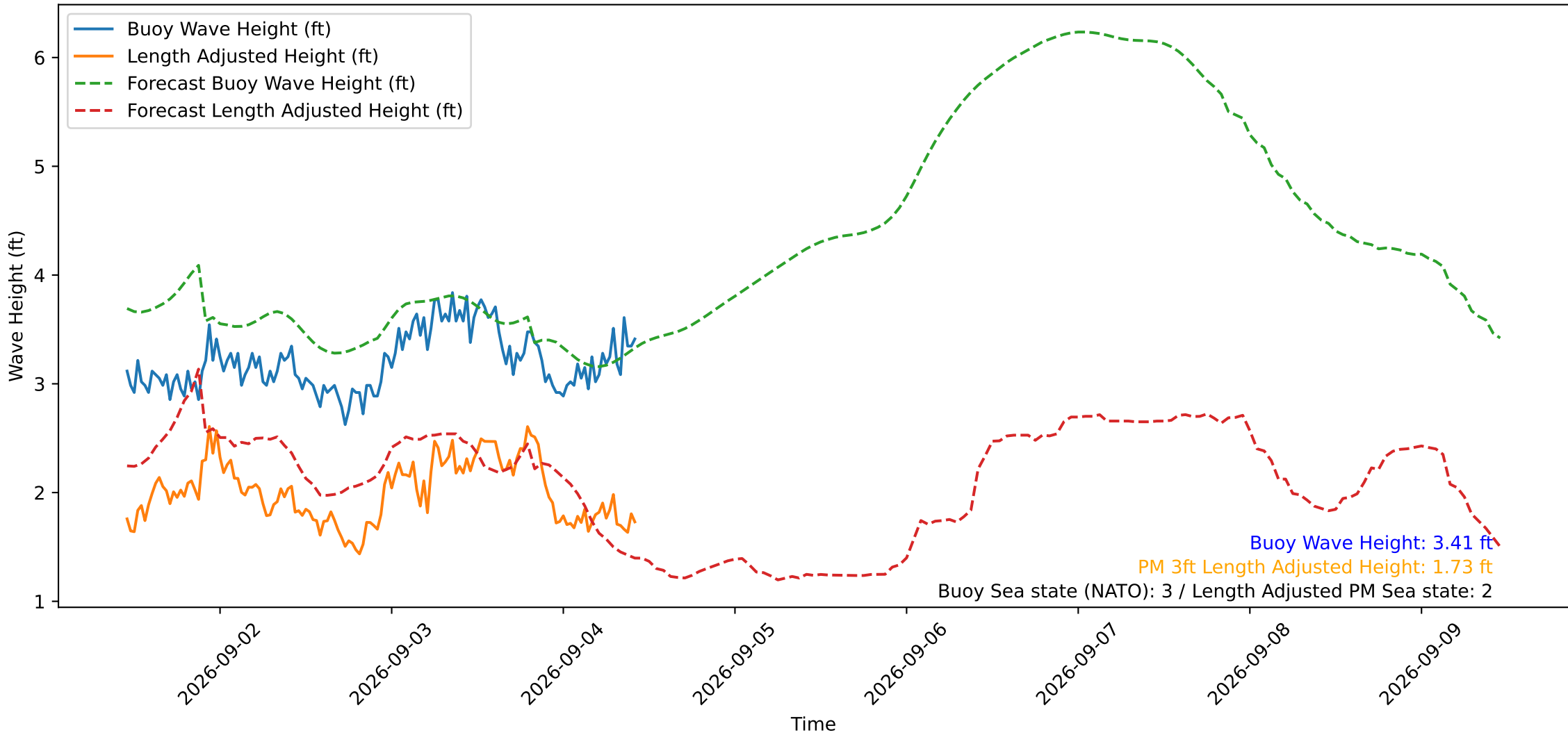
Wave Heights over Time for Oceanside Harbor at 2026-09-04 10:50:29
