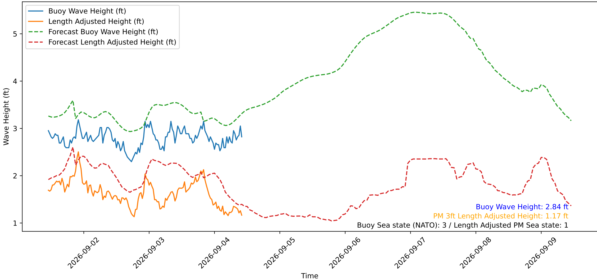
Wave Heights over Time for Red Beach at 2026-09-04 10:50:50
