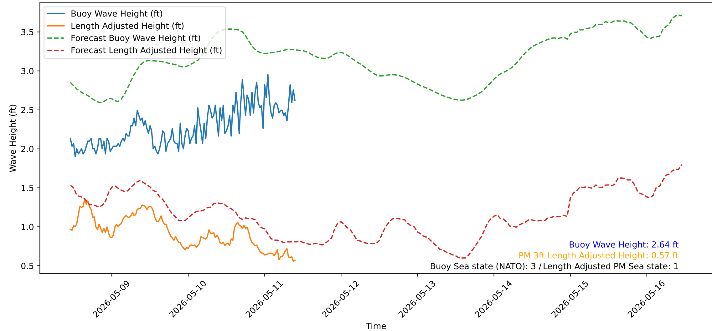
Wave Heights over Time for Red Beach at 2026-05-11 10:30:51
