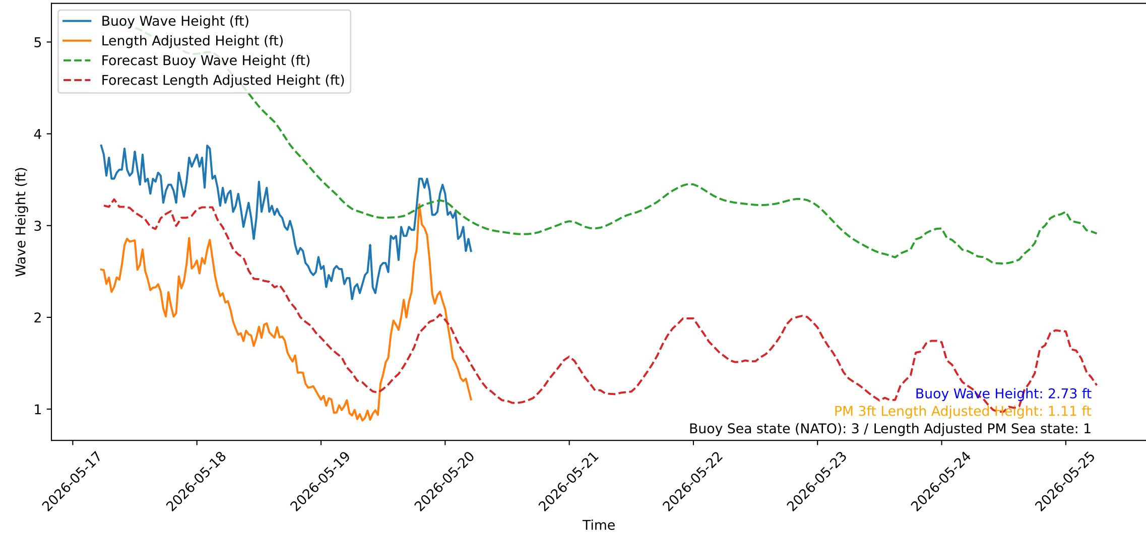
Wave Heights over Time for Oceanside Harbor at 2026-05-20 05:30:32
