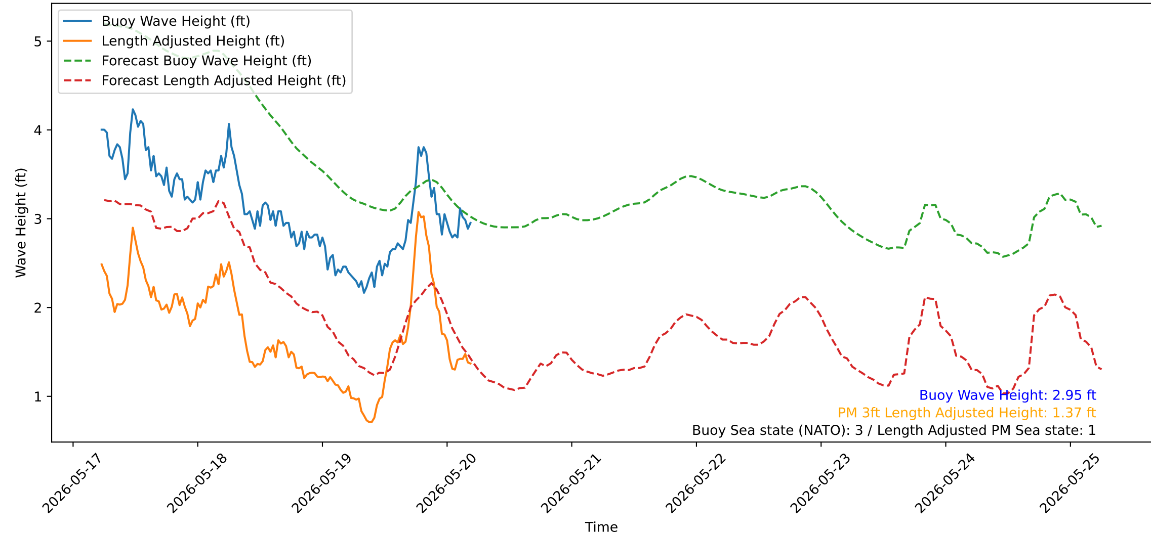
Wave Heights over Time for Green Beach at 2026-05-20 05:31:13
