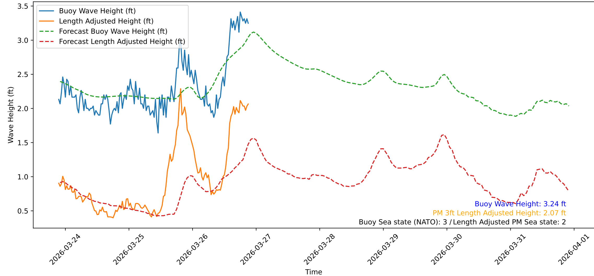
Wave Heights over Time for Green Beach at 2026-03-26 21:41:09
