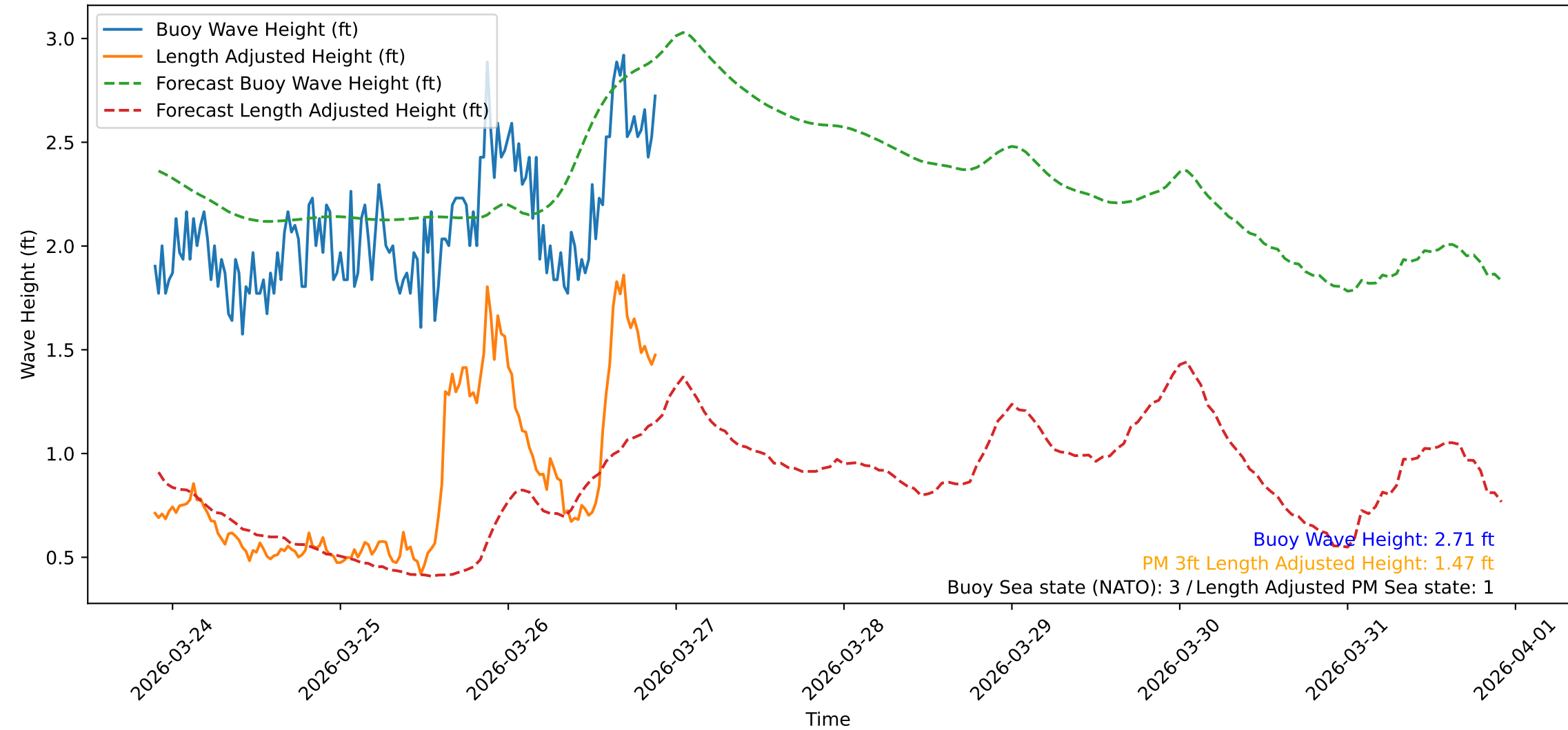
Wave Heights over Time for Oceanside Harbor at 2026-03-26 21:40:30
