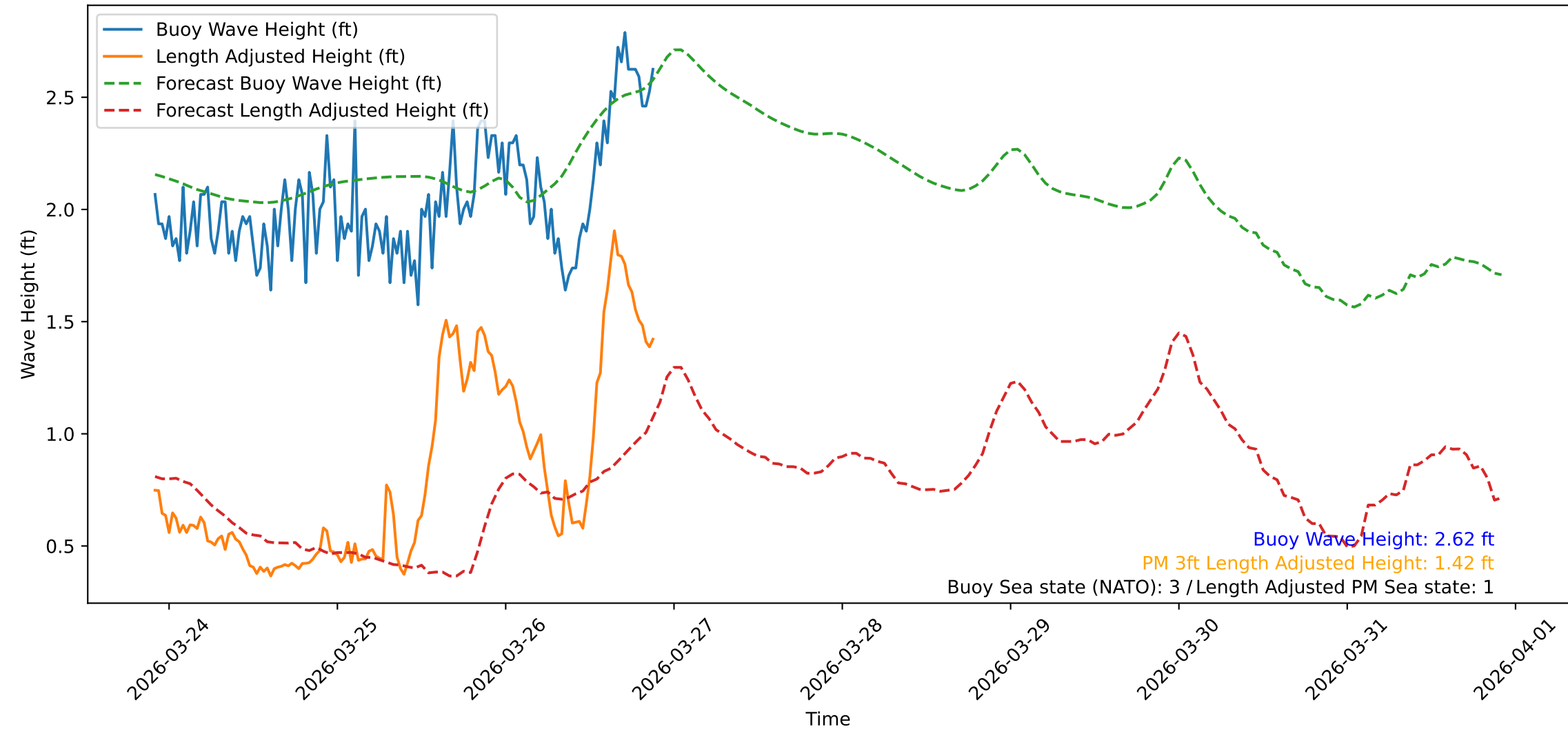
Wave Heights over Time for Red Beach at 2026-03-26 21:40:47
