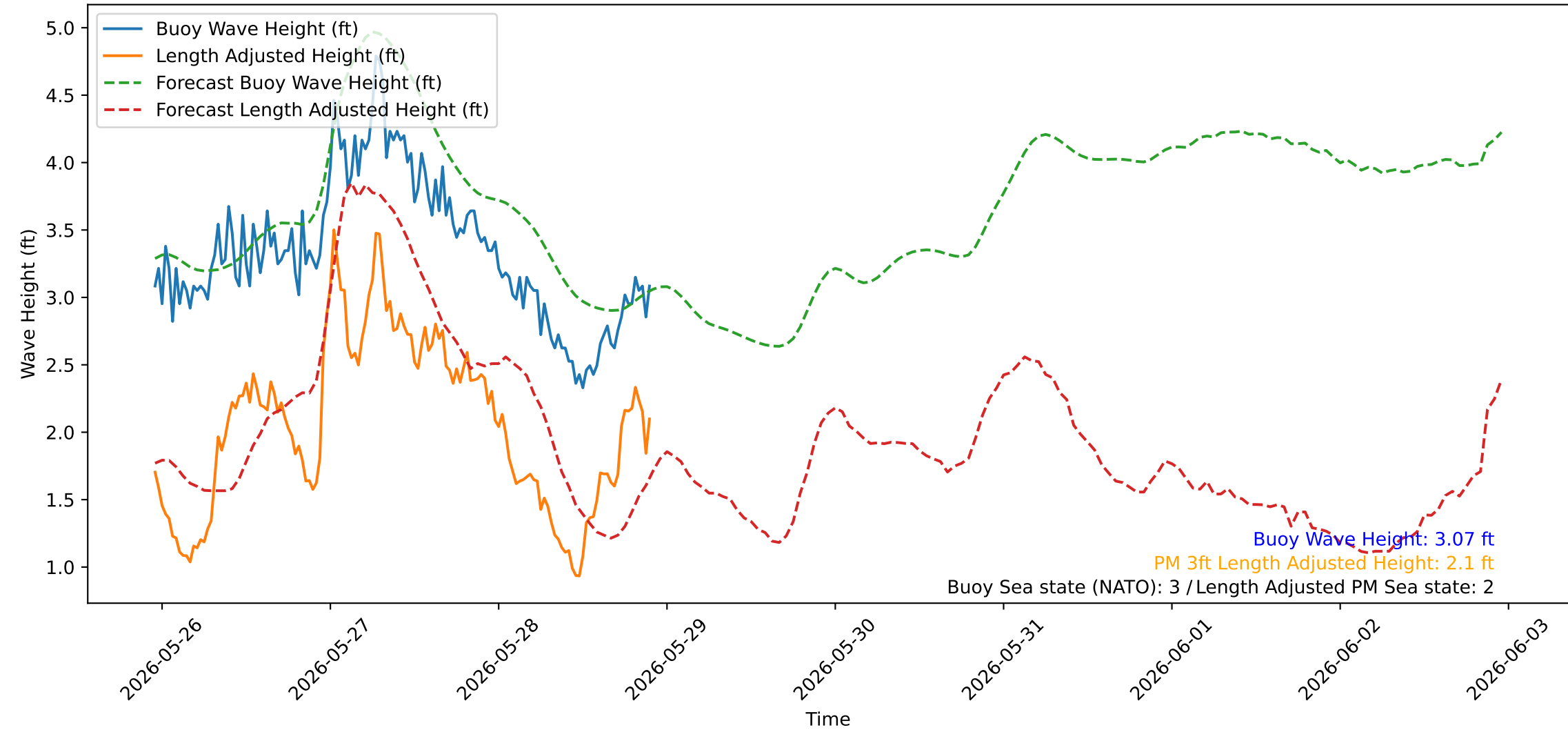
Wave Heights over Time for Red Beach at 2026-05-28 22:30:38
