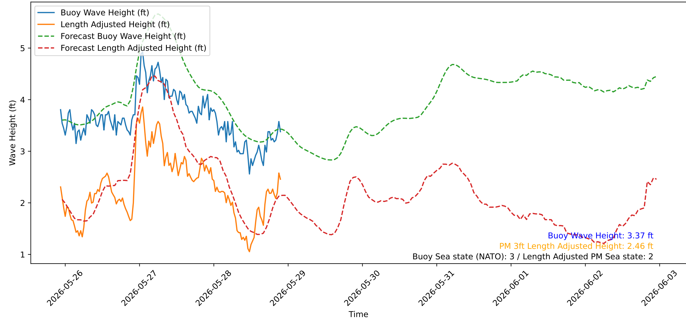
Wave Heights over Time for Green Beach at 2026-05-28 22:31:00
