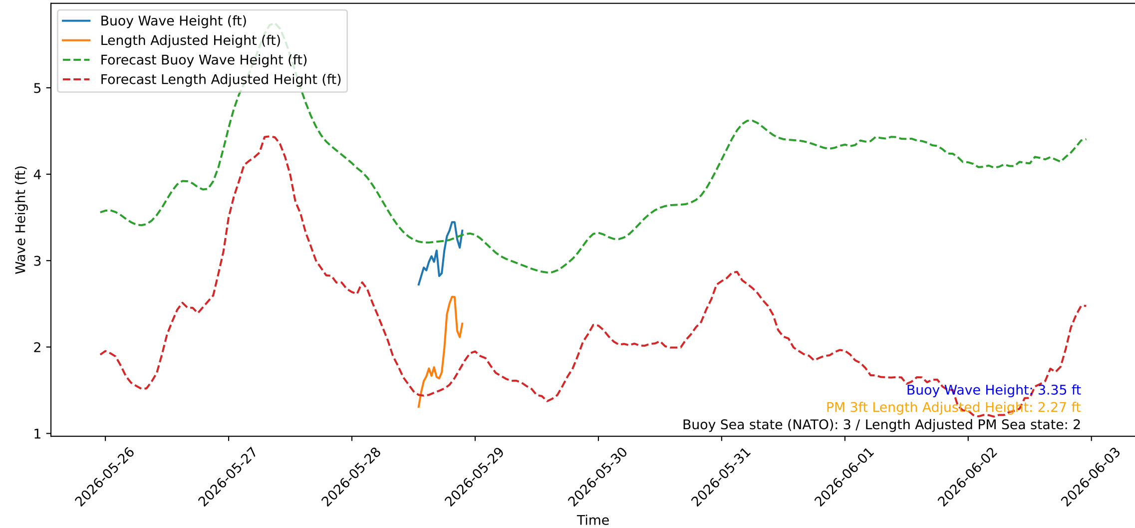
Wave Heights over Time for Oceanside Harbor at 2026-05-28 22:30:19
