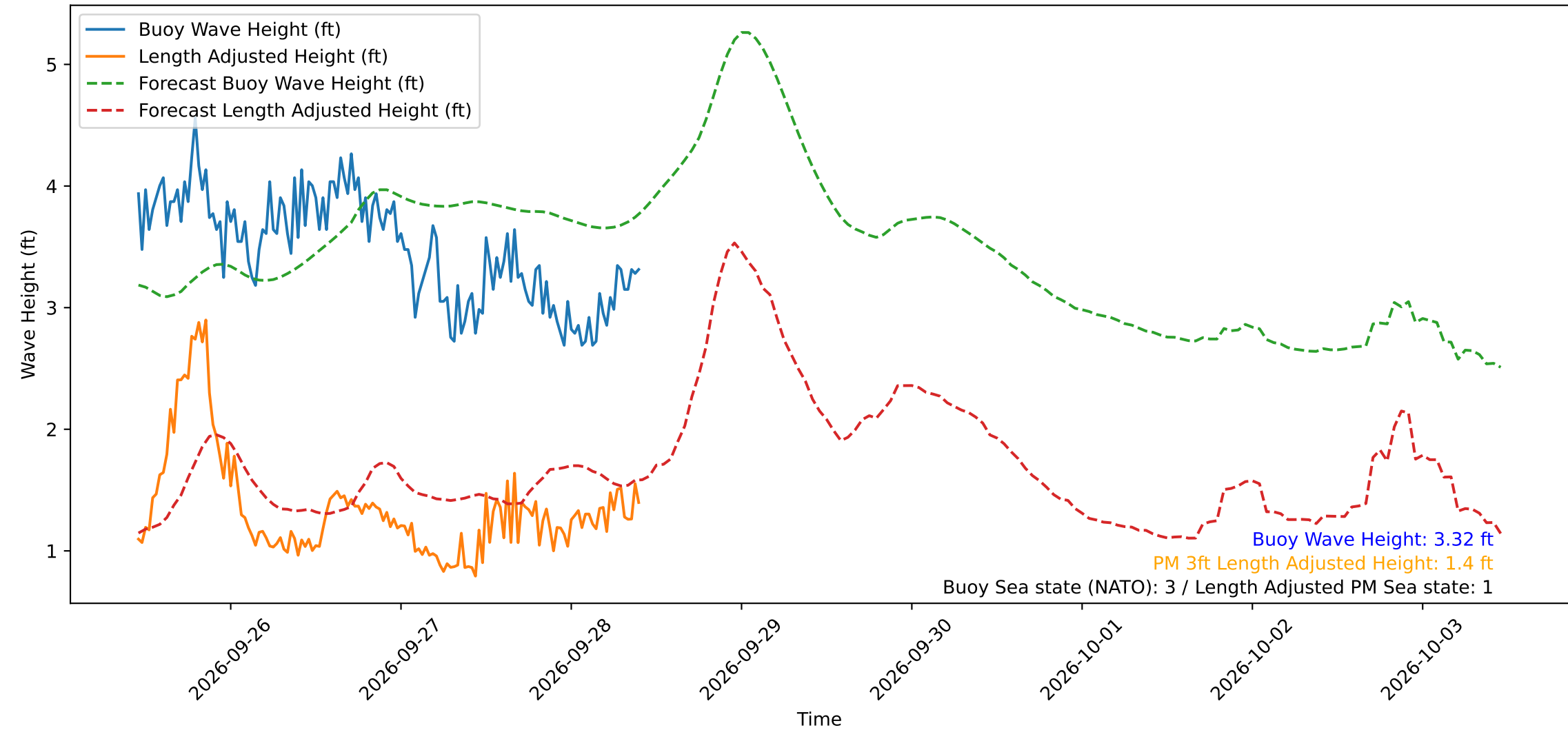
Wave Heights over Time for Green Beach at 2026-09-28 10:31:12
