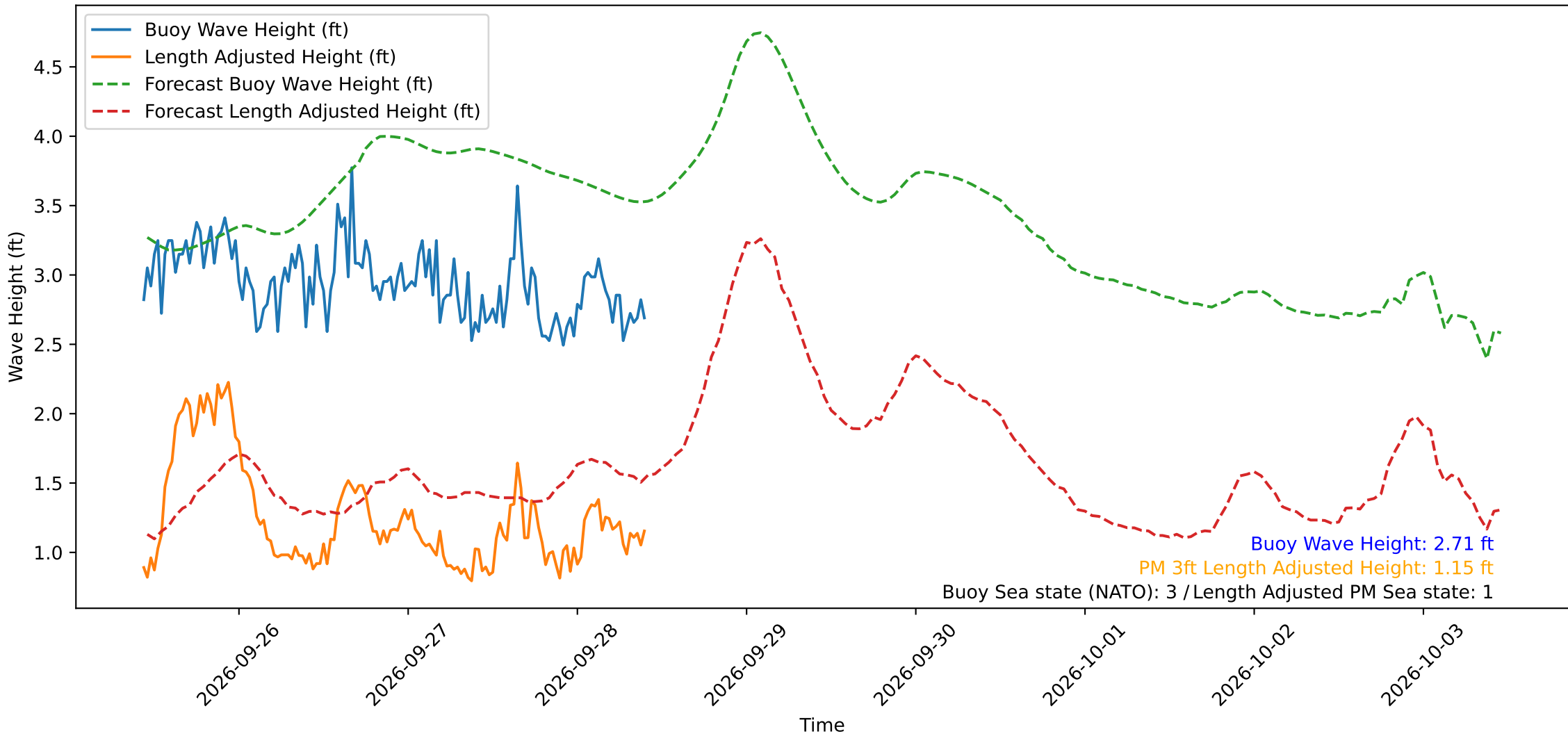
Wave Heights over Time for Oceanside Harbor at 2026-09-28 10:30:29
