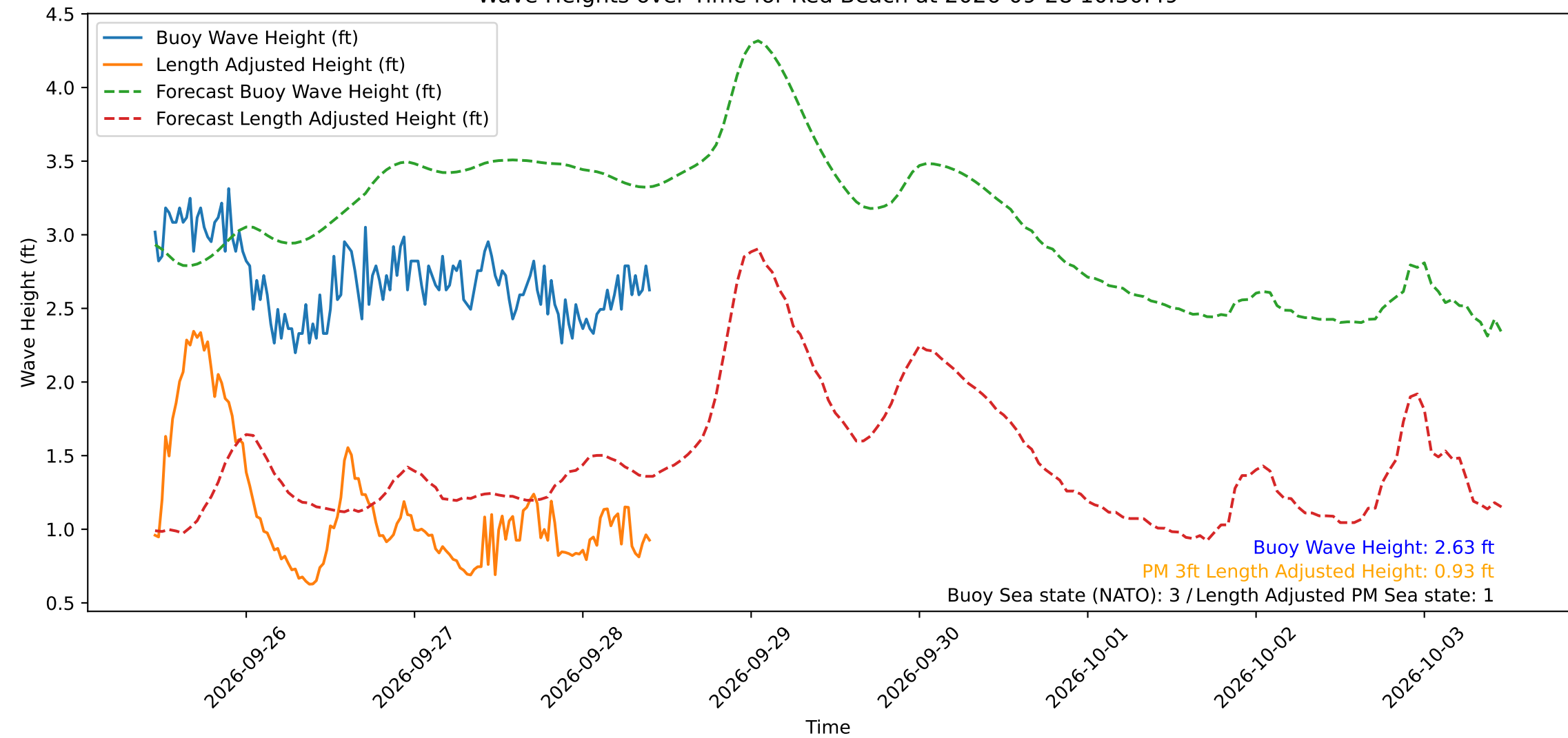
Wave Heights over Time for Red Beach at 2026-09-28 10:30:49
