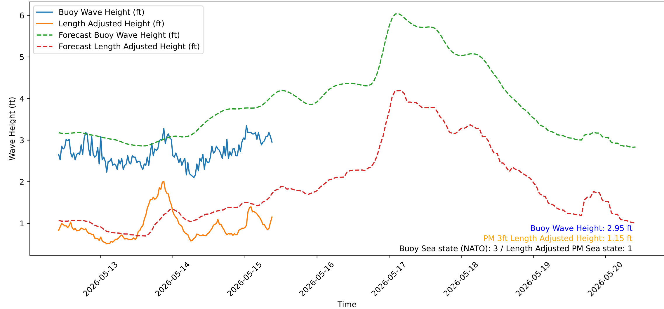
Wave Heights over Time for Green Beach at 2026-05-15 10:01:14
