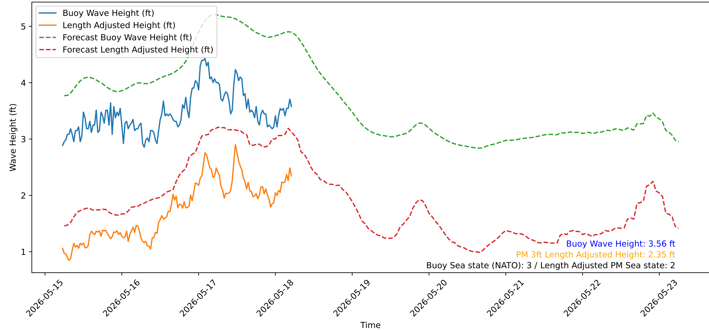
Wave Heights over Time for Green Beach at 2026-05-18 05:41:14
