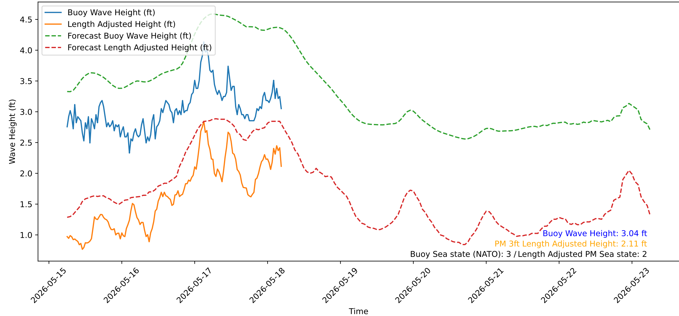
Wave Heights over Time for Red Beach at 2026-05-18 05:40:51
