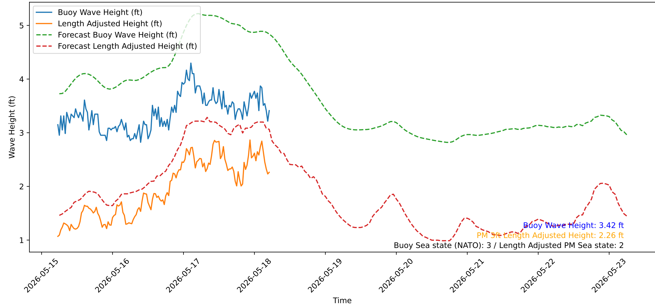
Wave Heights over Time for Oceanside Harbor at 2026-05-18 05:40:31
