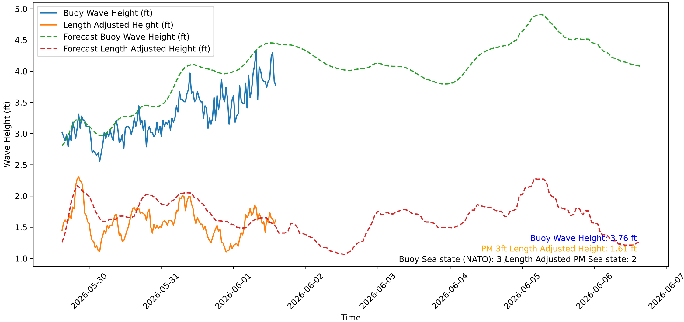
Wave Heights over Time for Green Beach at 2026-06-01 15:01:08
