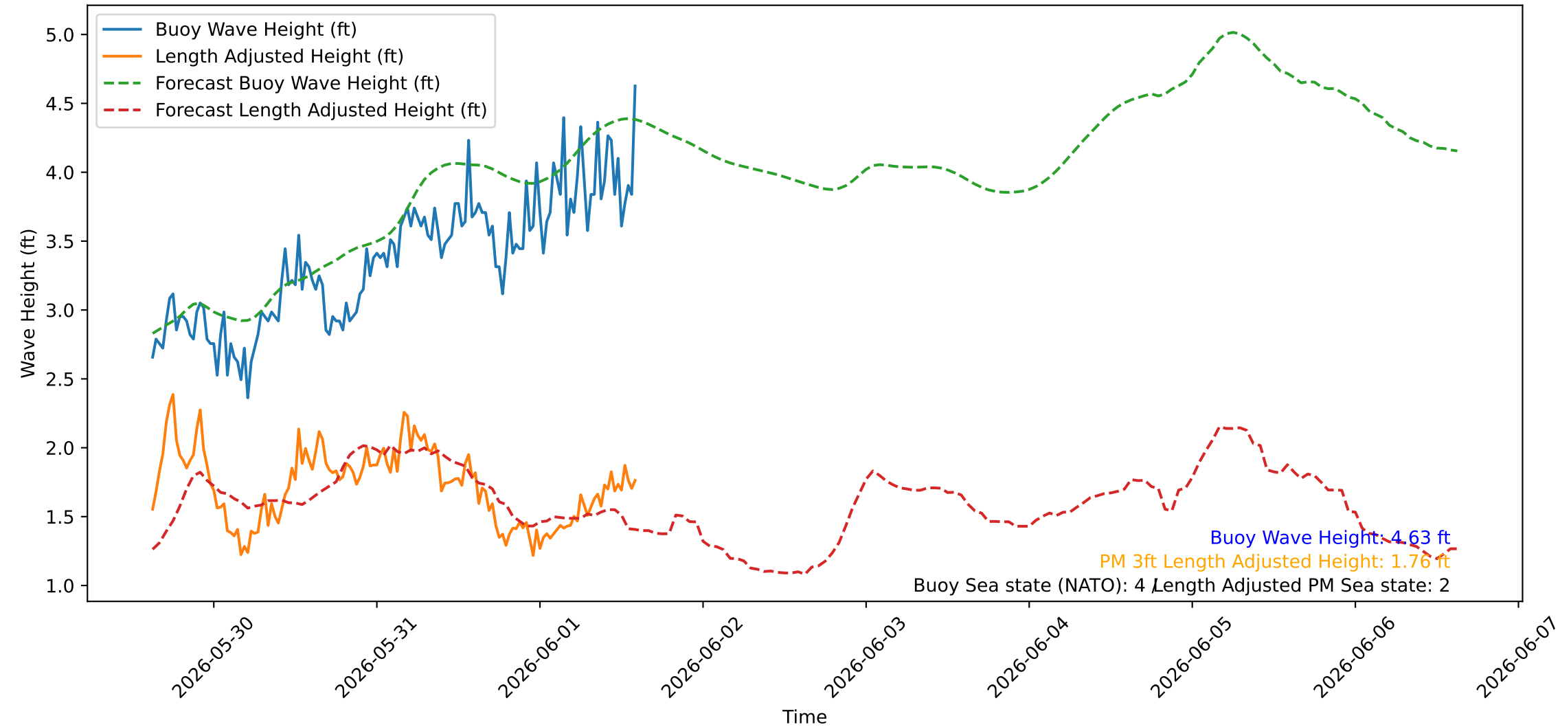
Wave Heights over Time for Oceanside Harbor at 2026-06-01 15:00:26
