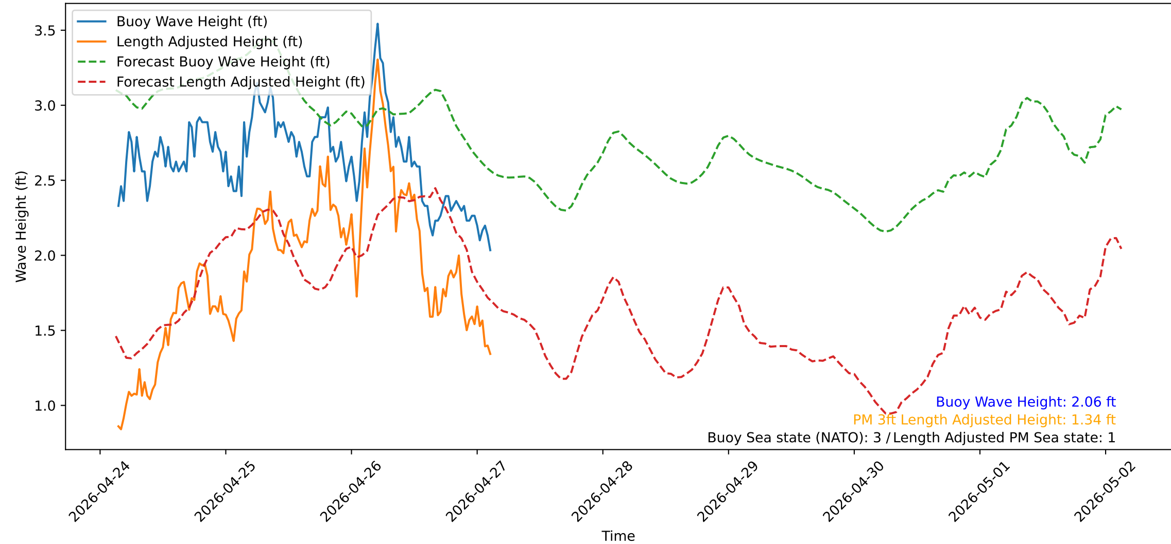
Wave Heights over Time for Red Beach at 2026-04-27 03:20:51
