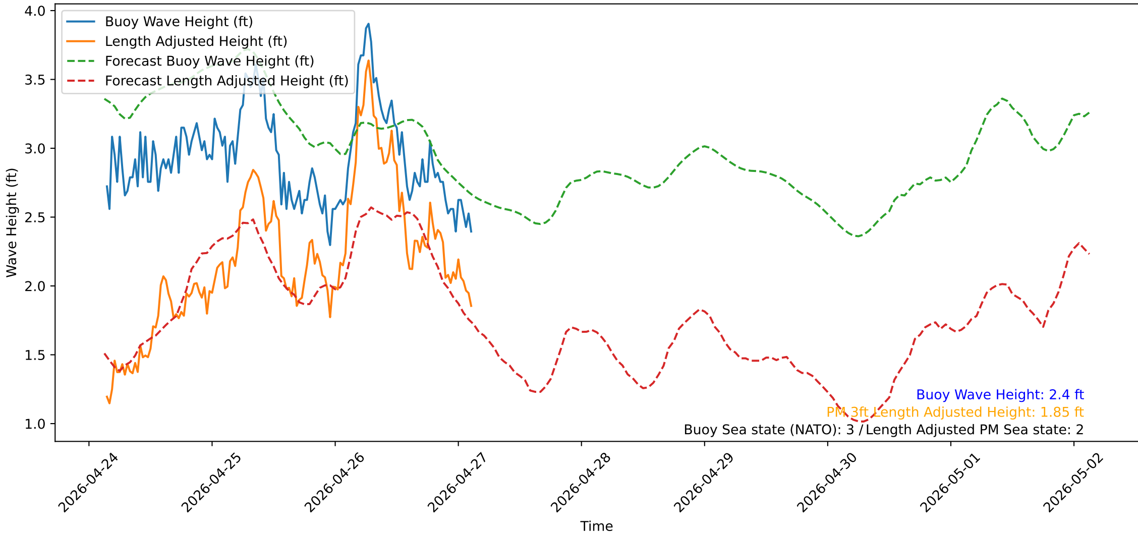
Wave Heights over Time for Oceanside Harbor at 2026-04-27 03:20:31
