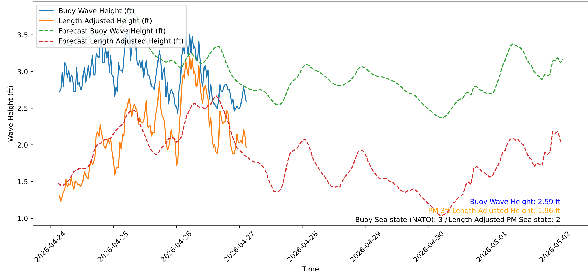
Wave Heights over Time for Green Beach at 2026-04-27 03:21:14
