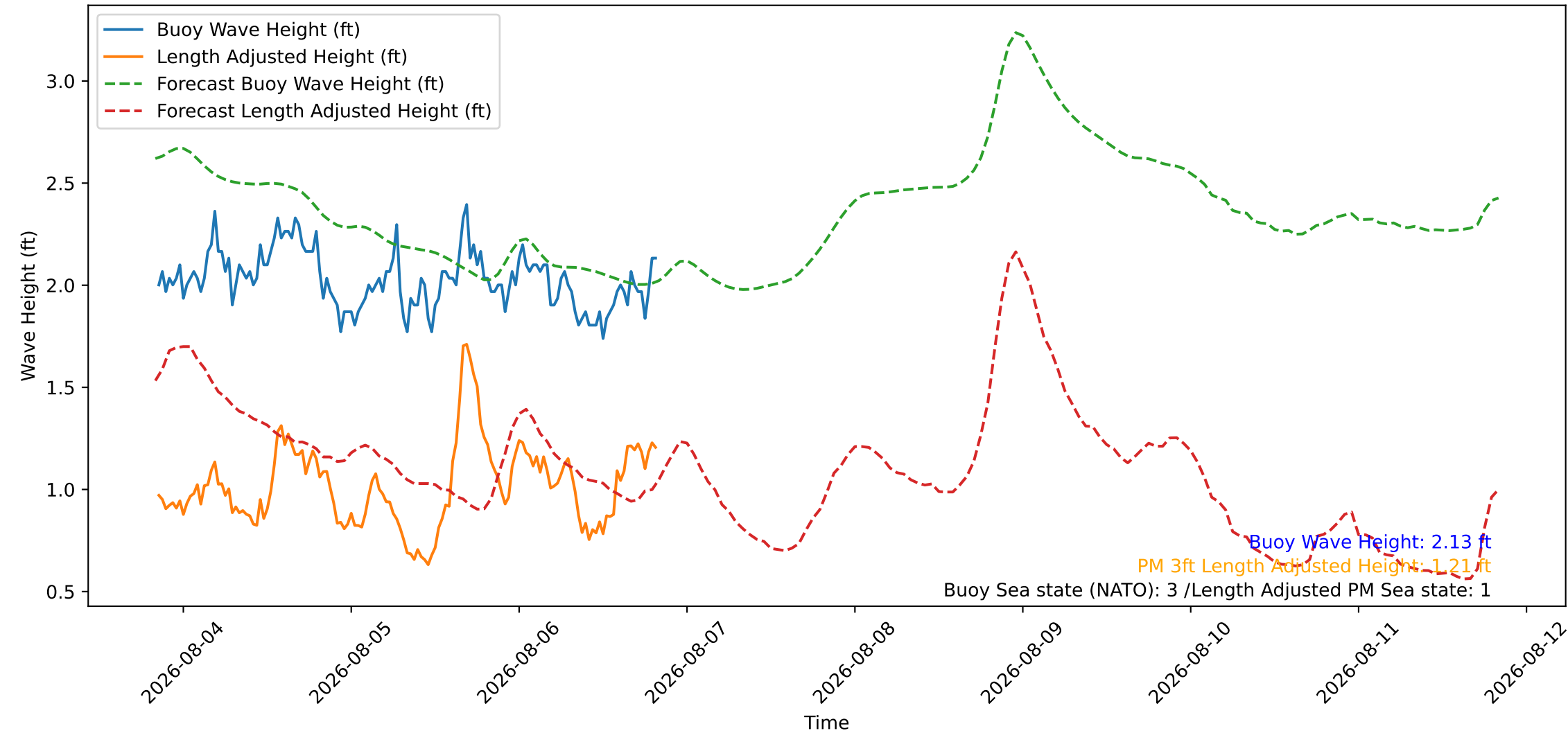
Wave Heights over Time for Red Beach at 2026-08-06 20:20:47
