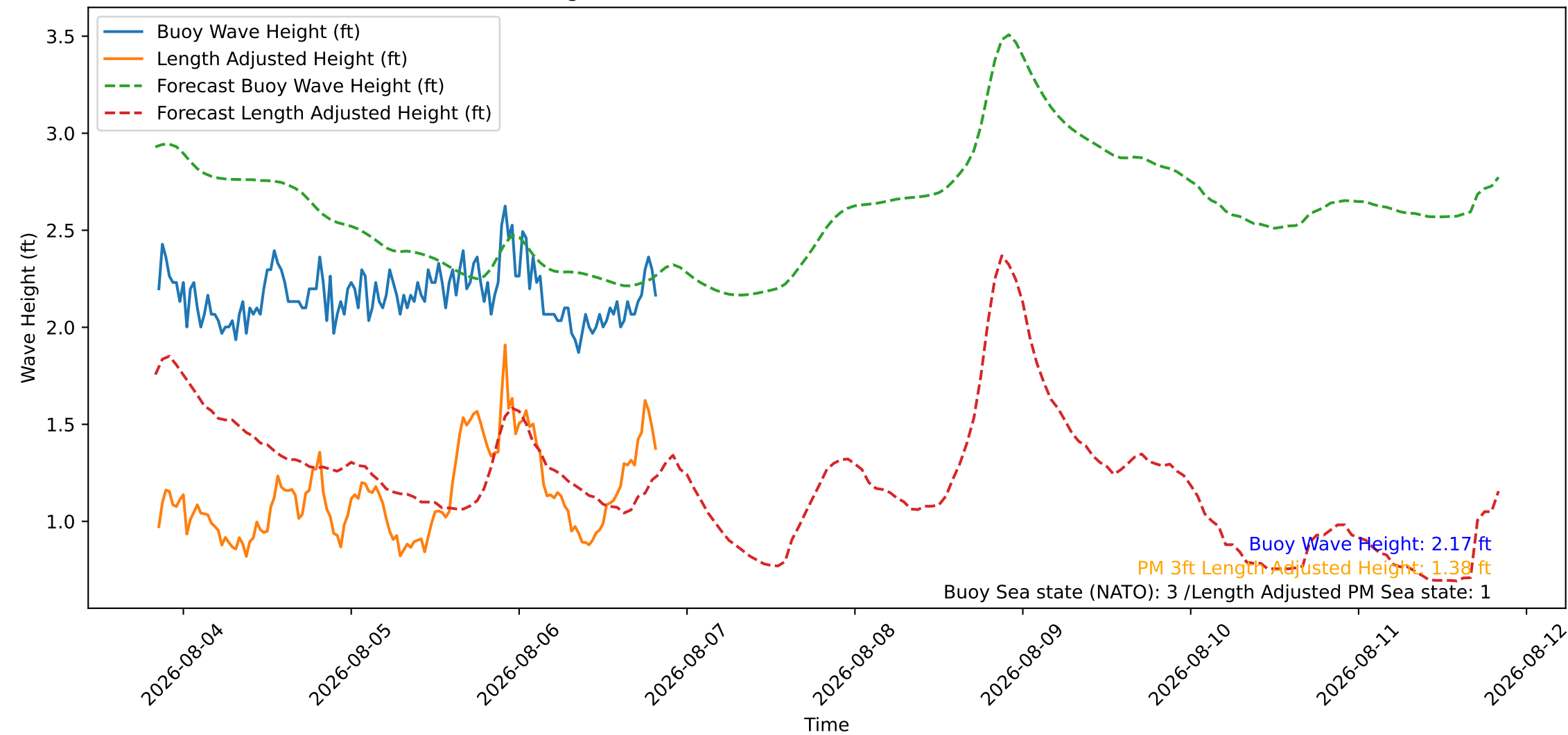
Wave Heights over Time for Green Beach at 2026-08-06 20:21:09
