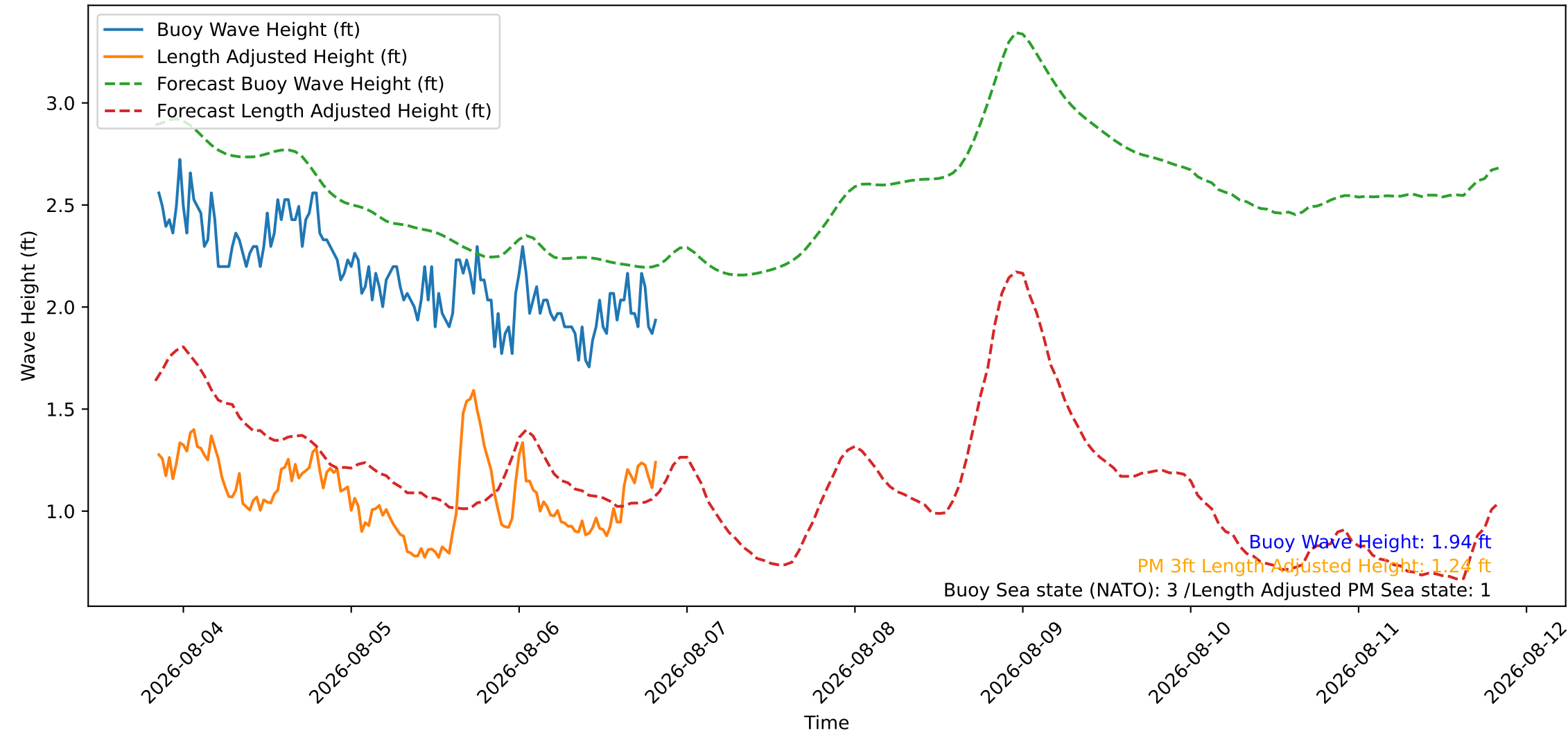
Wave Heights over Time for Oceanside Harbor at 2026-08-06 20:20:26
