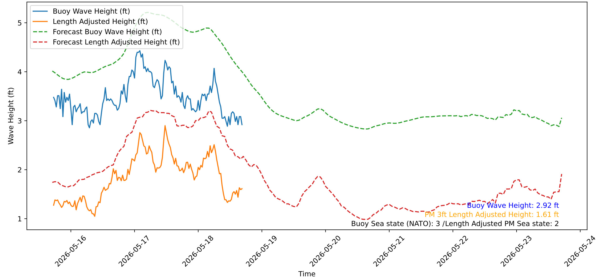
Wave Heights over Time for Green Beach at 2026-05-18 17:21:14
