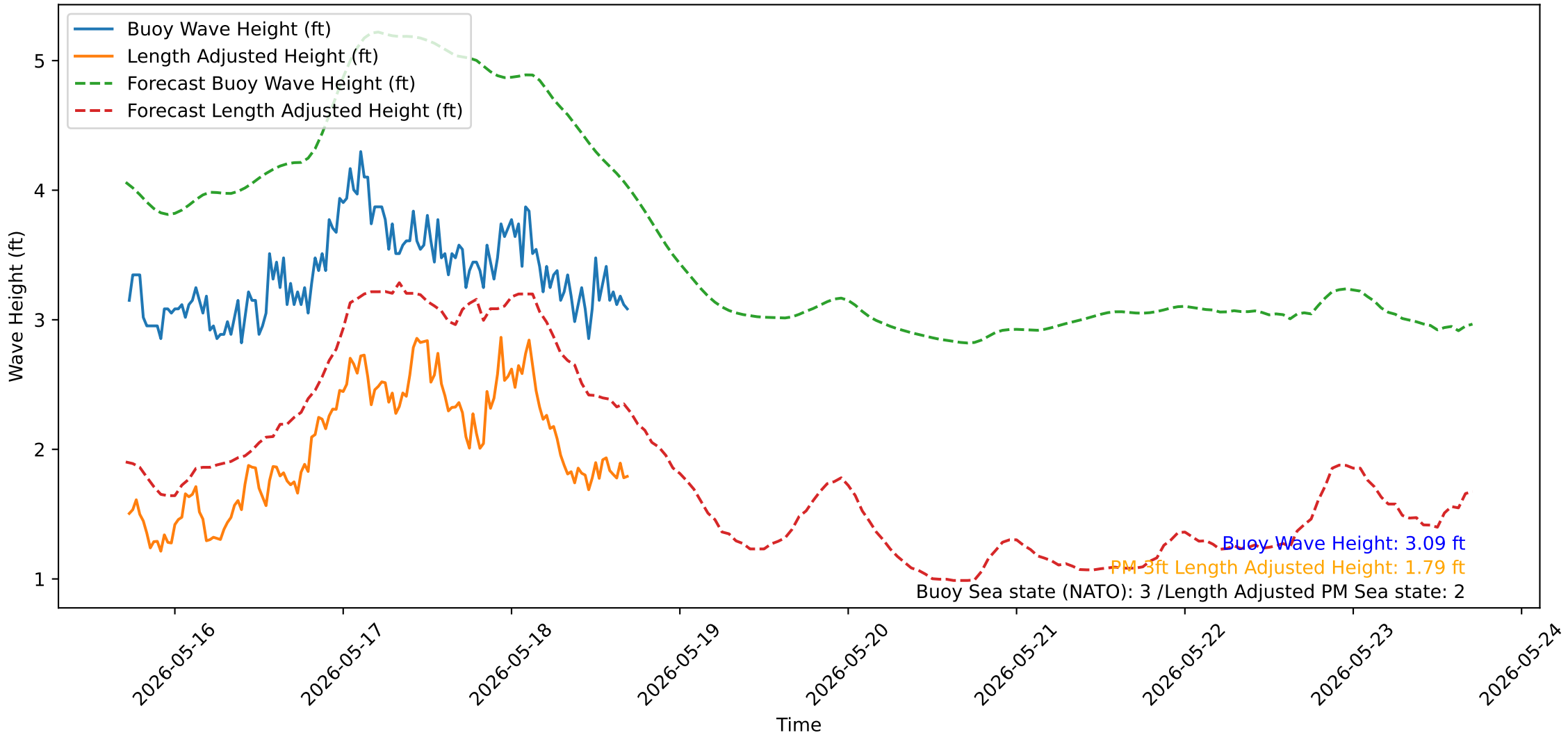
Wave Heights over Time for Oceanside Harbor at 2026-05-18 17:20:31
