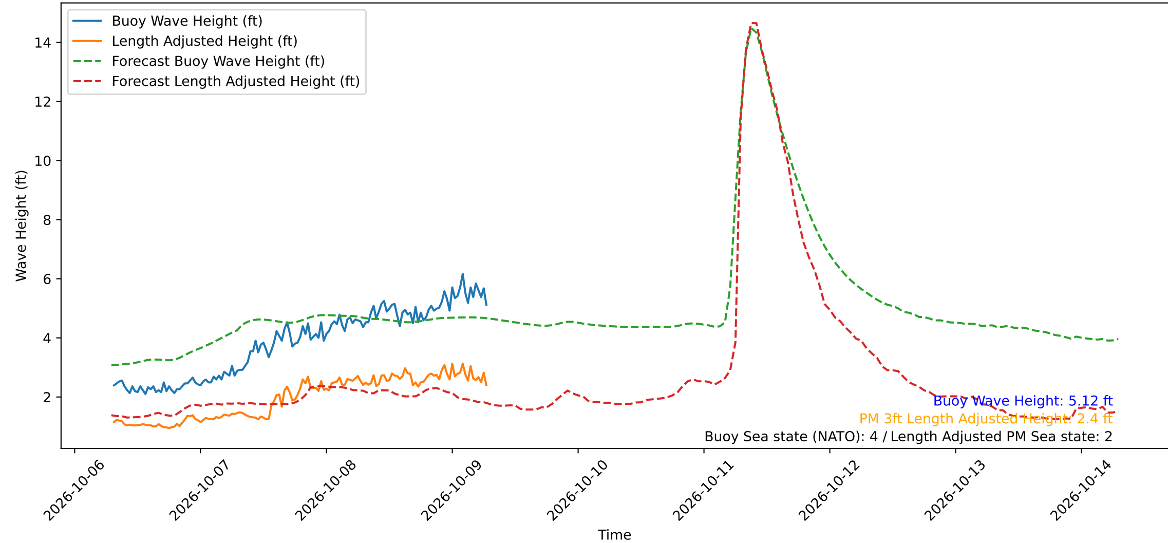
Wave Heights over Time for Green Beach at 2026-10-09 07:11:11
