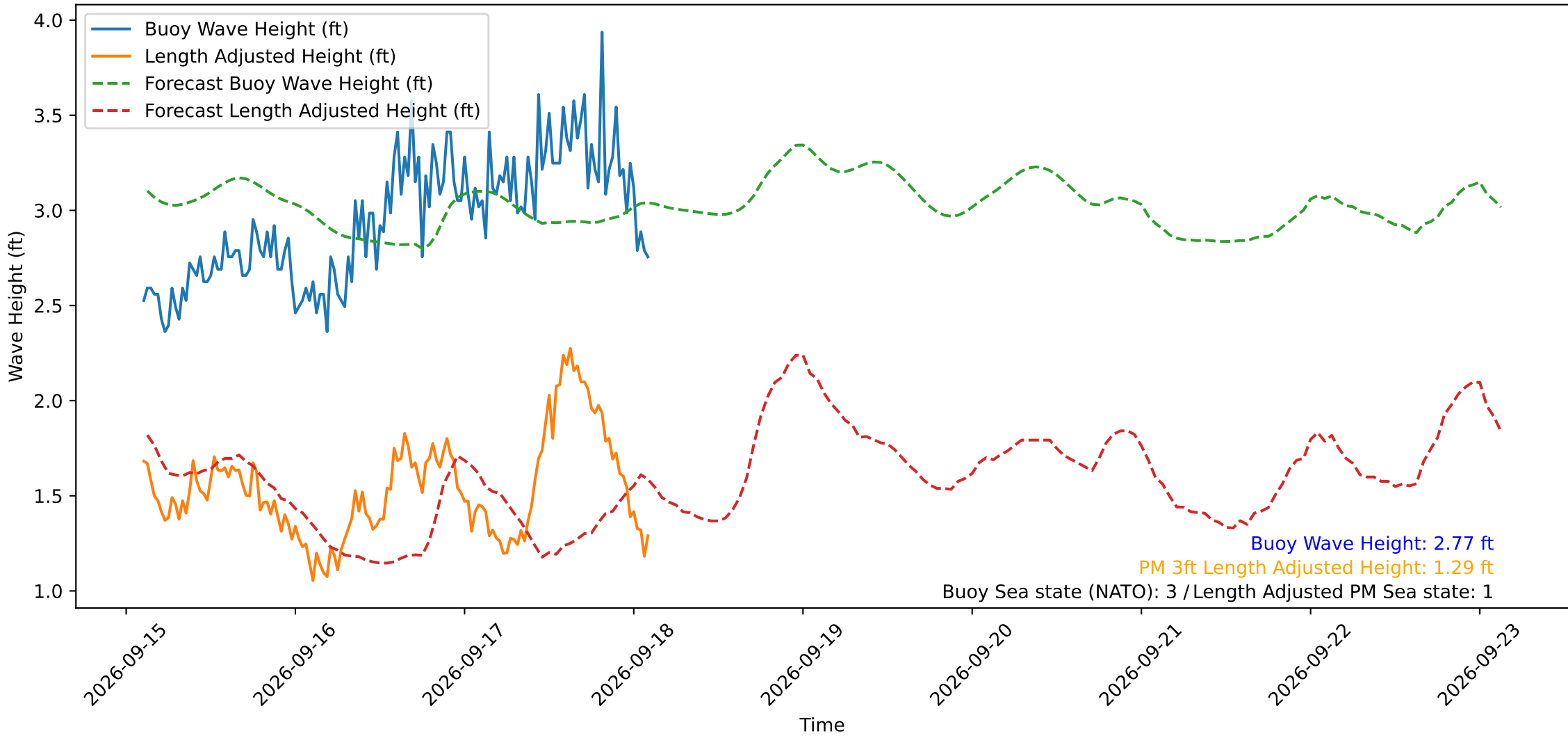
Wave Heights over Time for Oceanside Harbor at 2026-09-18 02:40:29
