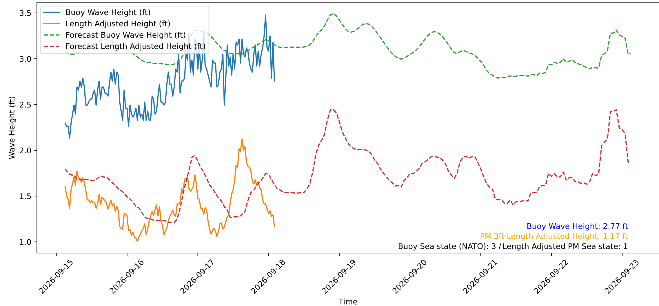
Wave Heights over Time for Green Beach at 2026-09-18 02:41:11
