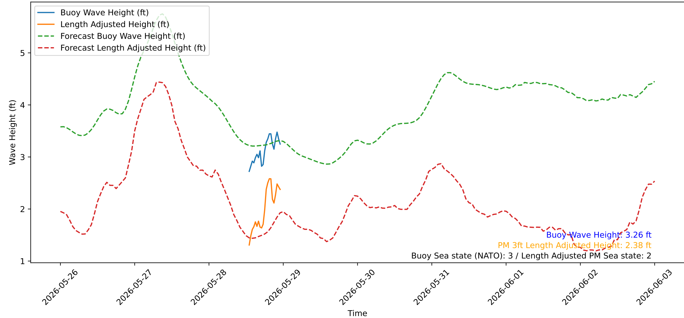
Wave Heights over Time for Oceanside Harbor at 2026-05-29 00:00:21
