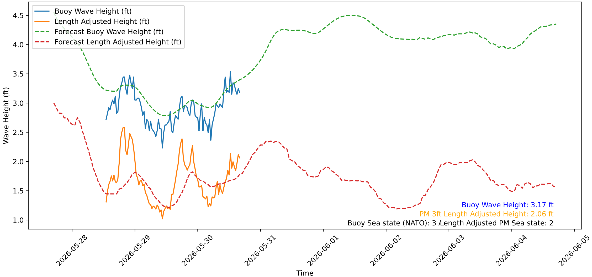
Wave Heights over Time for Oceanside Harbor at 2026-05-30 16:50:24
