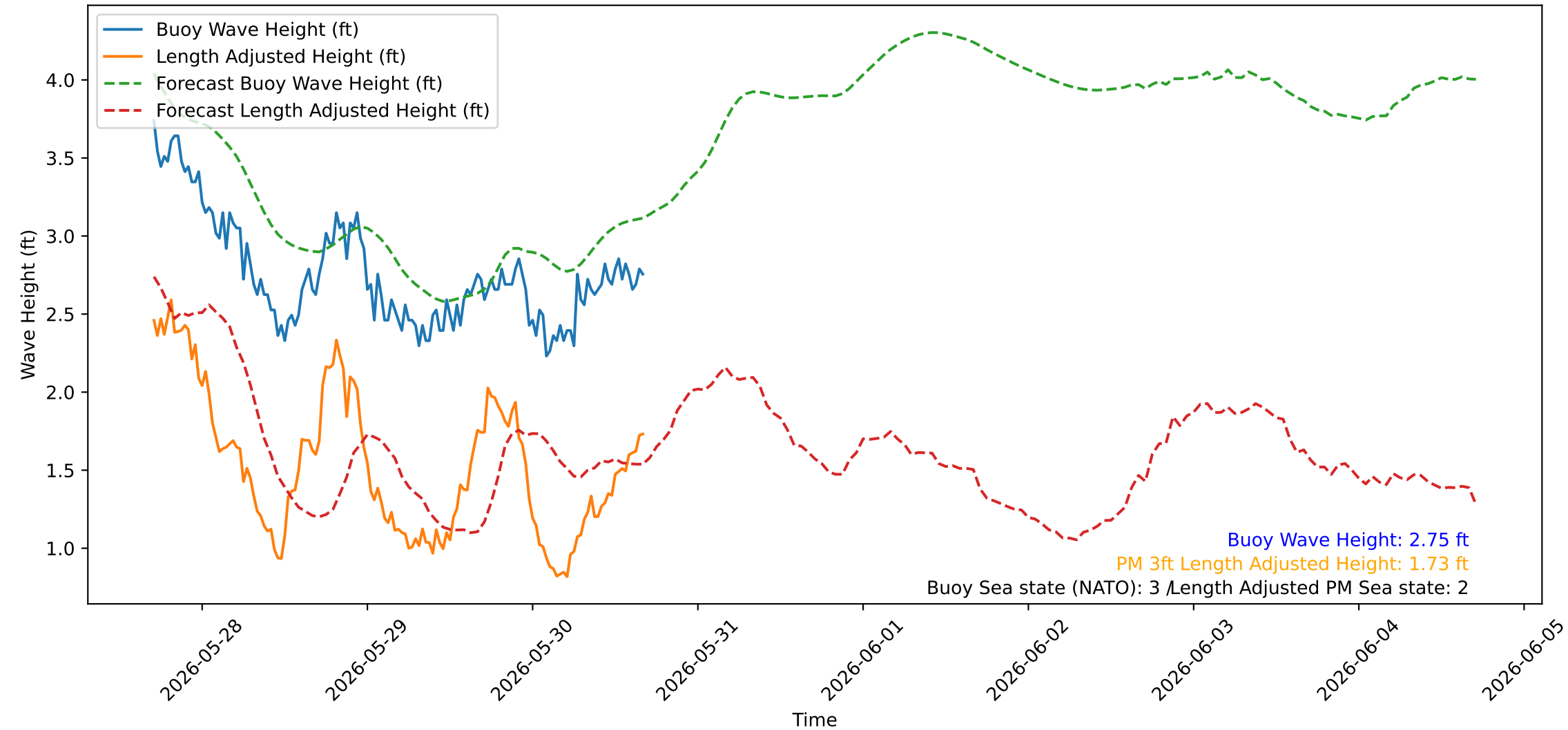
Wave Heights over Time for Red Beach at 2026-05-30 16:50:44
