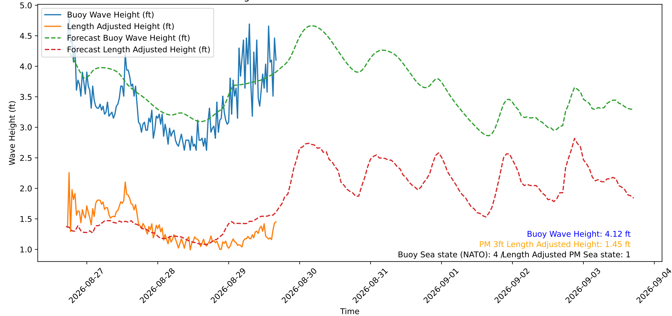
Wave Heights over Time for Red Beach at 2026-08-29 17:00:48
