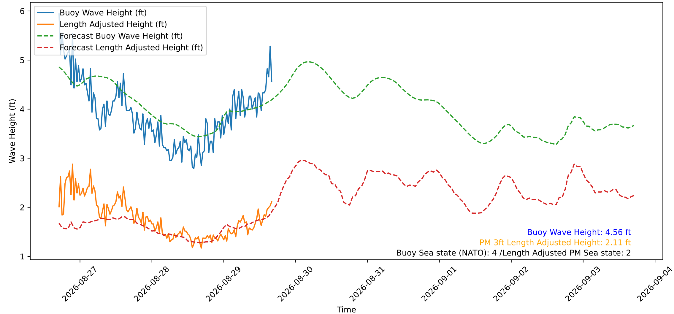
Wave Heights over Time for Oceanside Harbor at 2026-08-29 17:00:29
