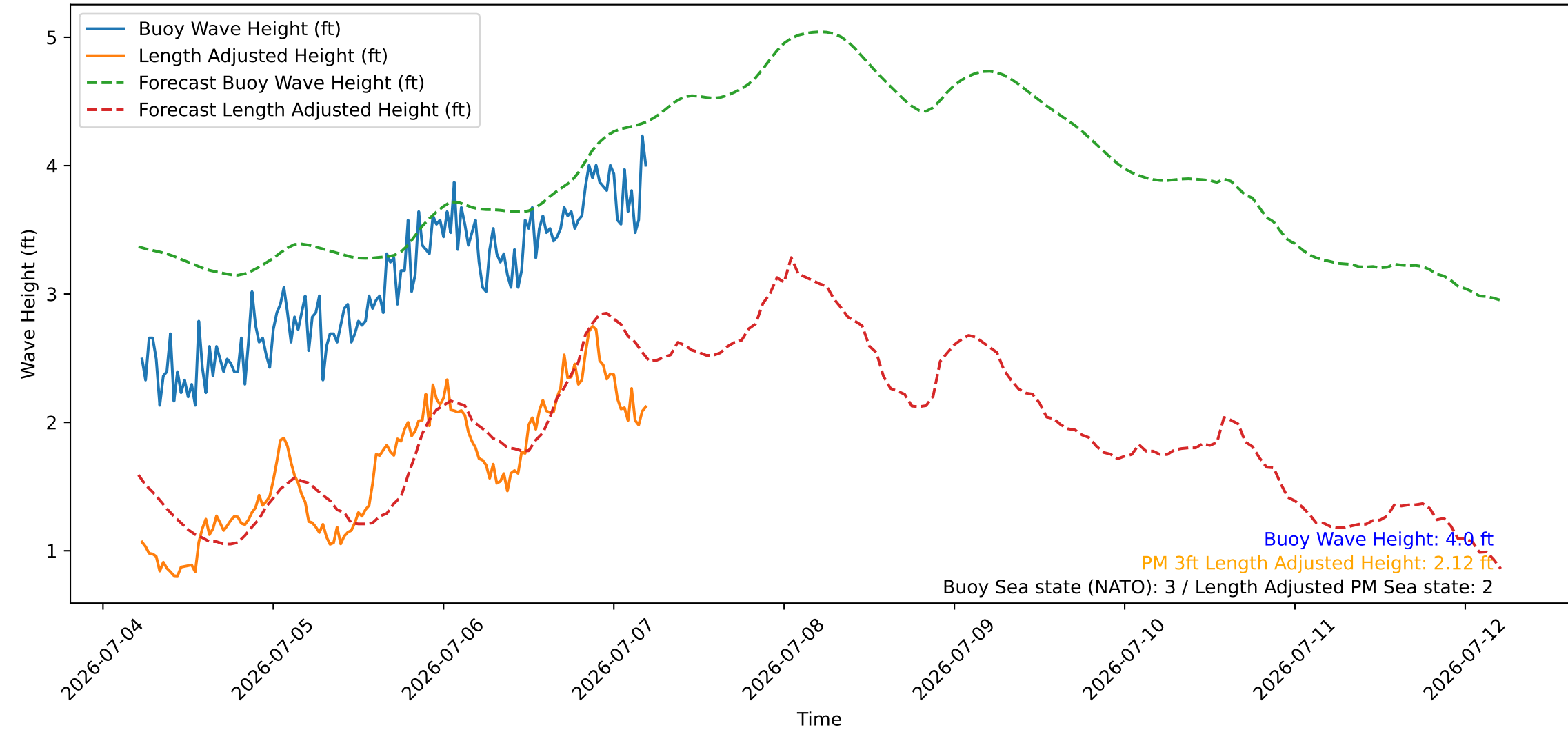
Wave Heights over Time for Oceanside Harbor at 2026-07-07 05:20:26
