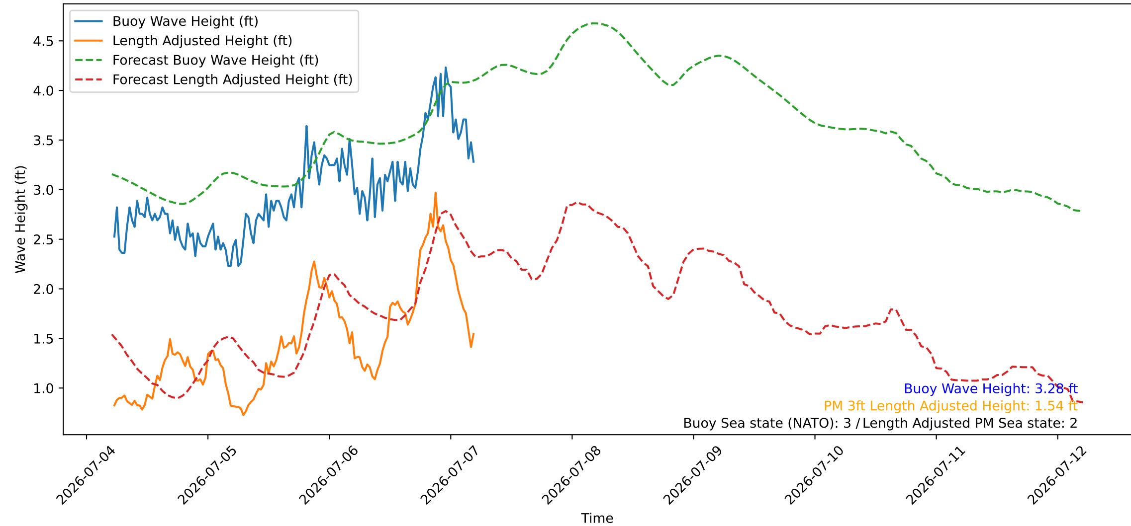
Wave Heights over Time for Red Beach at 2026-07-07 05:20:47
