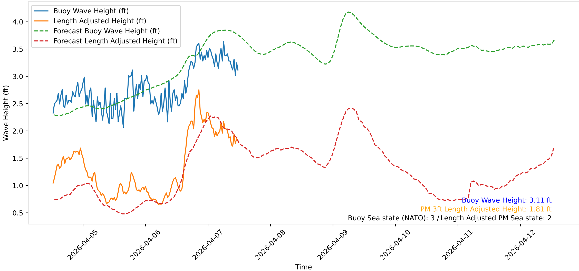
Wave Heights over Time for Oceanside Harbor at 2026-04-07 12:30:32
