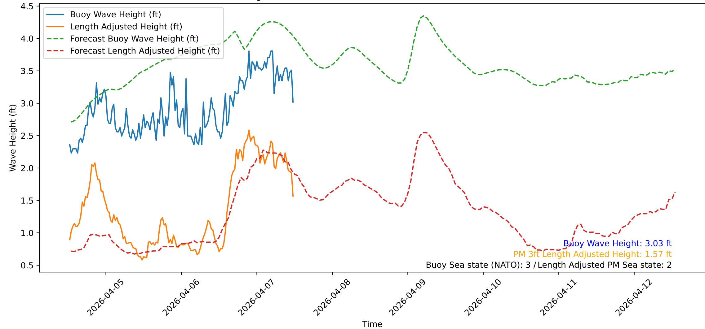
Wave Heights over Time for Green Beach at 2026-04-07 12:31:11
