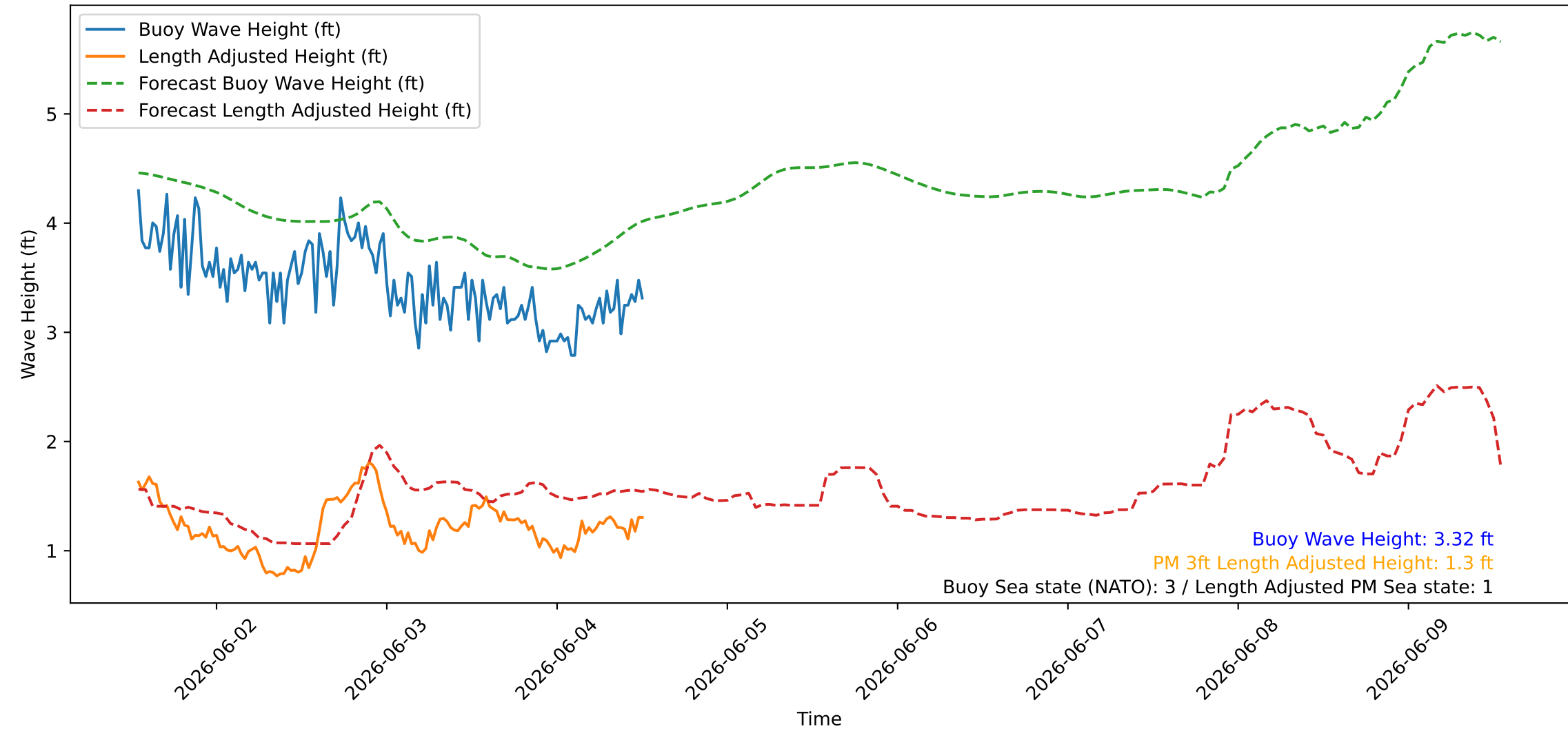
Wave Heights over Time for Green Beach at 2026-06-04 13:01:07
