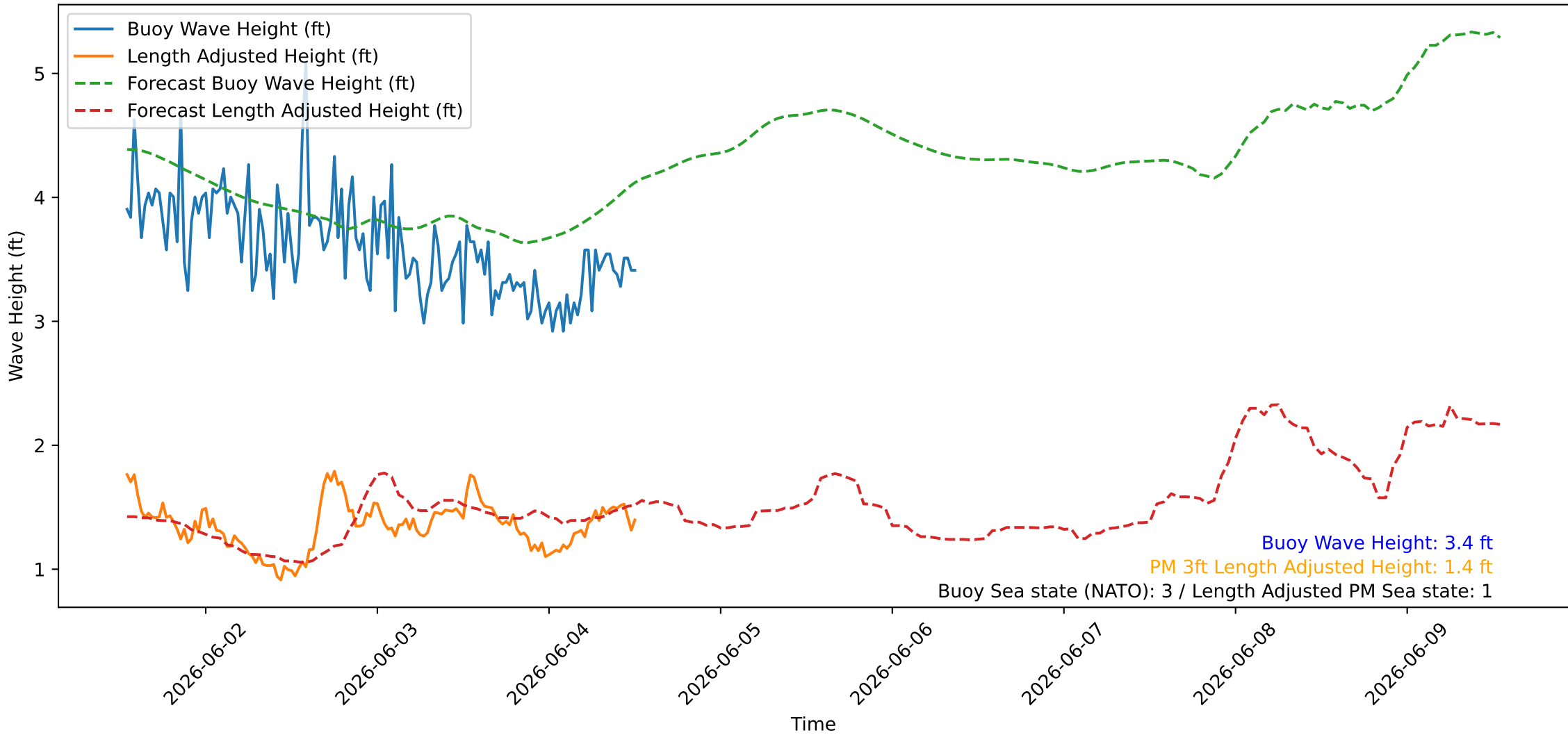
Wave Heights over Time for Oceanside Harbor at 2026-06-04 13:00:26
