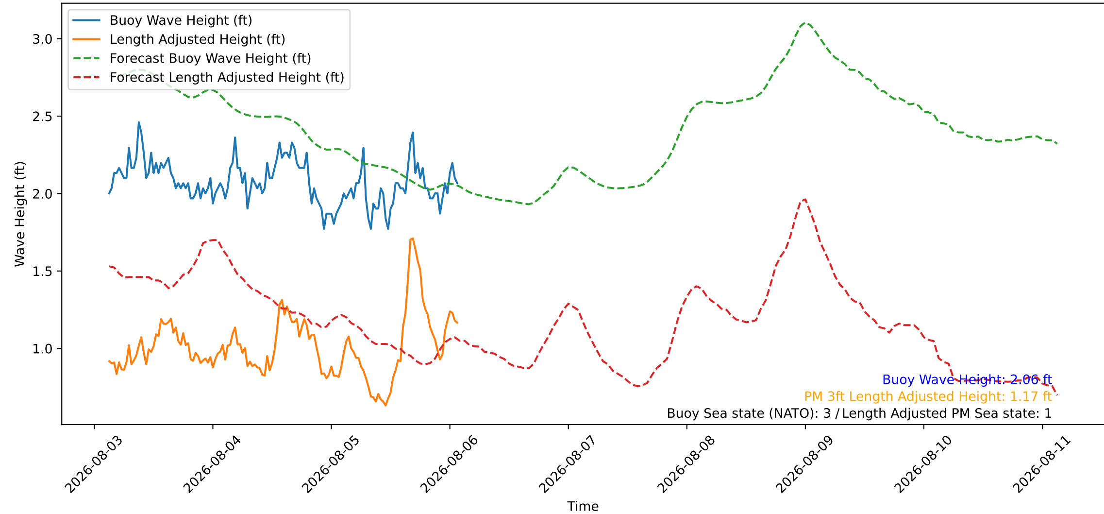
Wave Heights over Time for Red Beach at 2026-08-06 02:30:45
