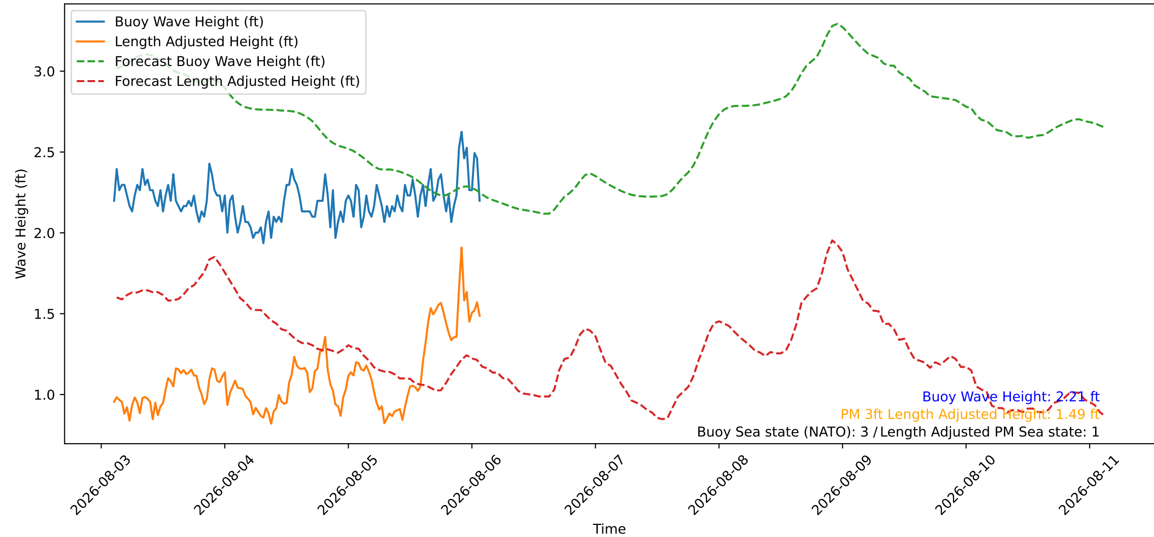
Wave Heights over Time for Green Beach at 2026-08-06 02:31:07
