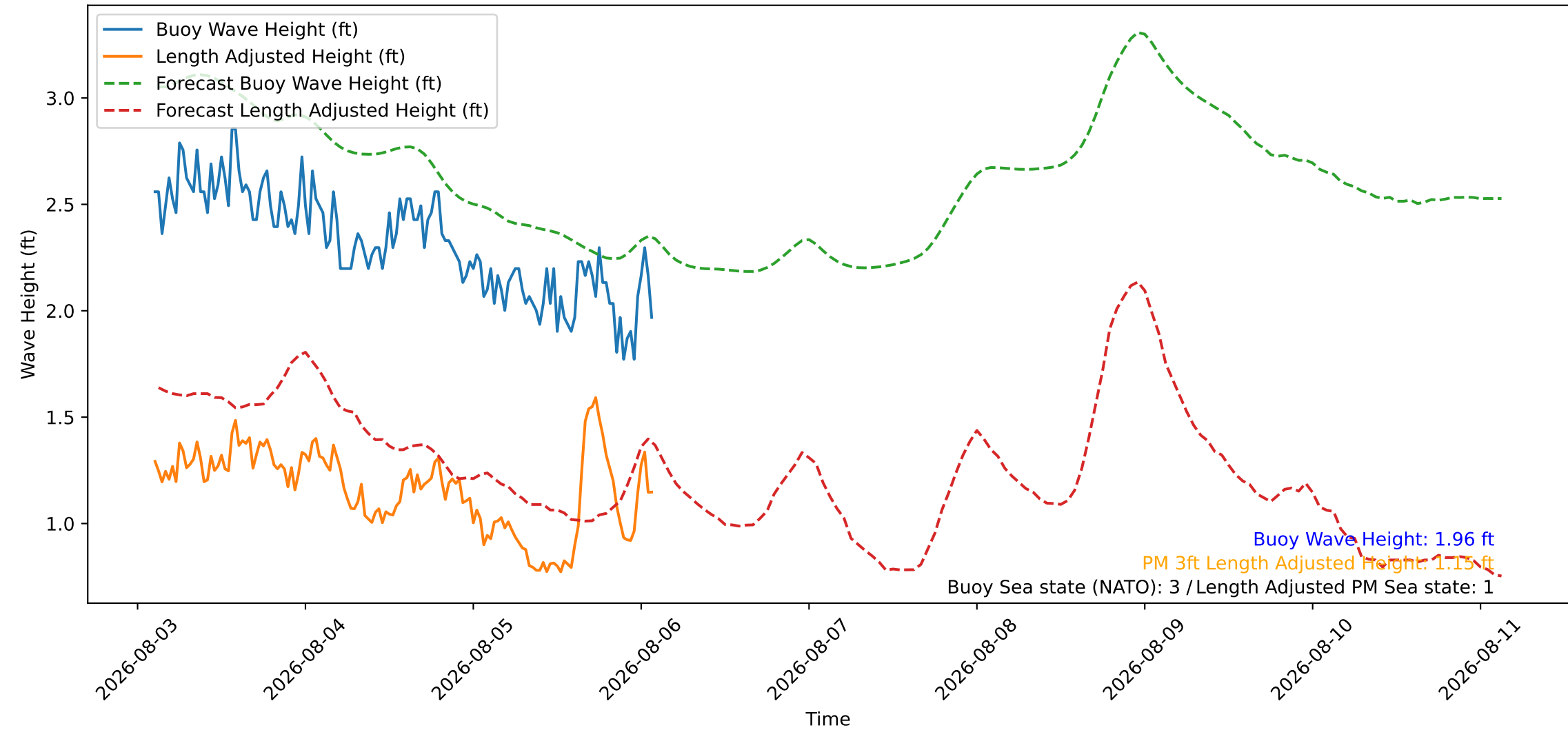
Wave Heights over Time for Oceanside Harbor at 2026-08-06 02:30:26
