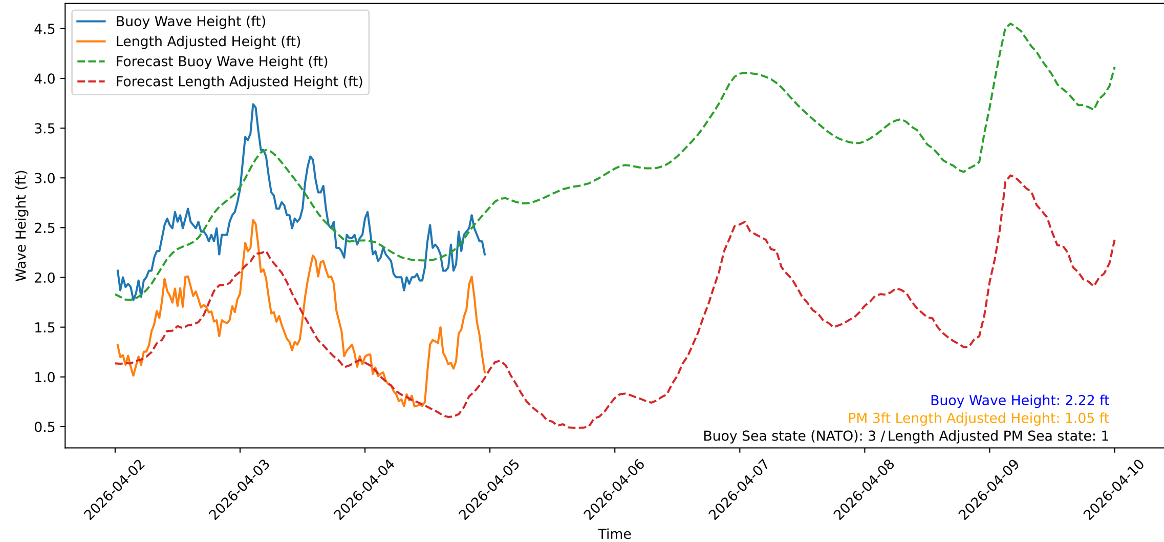
Wave Heights over Time for Red Beach at 2026-04-05 00:00:48
