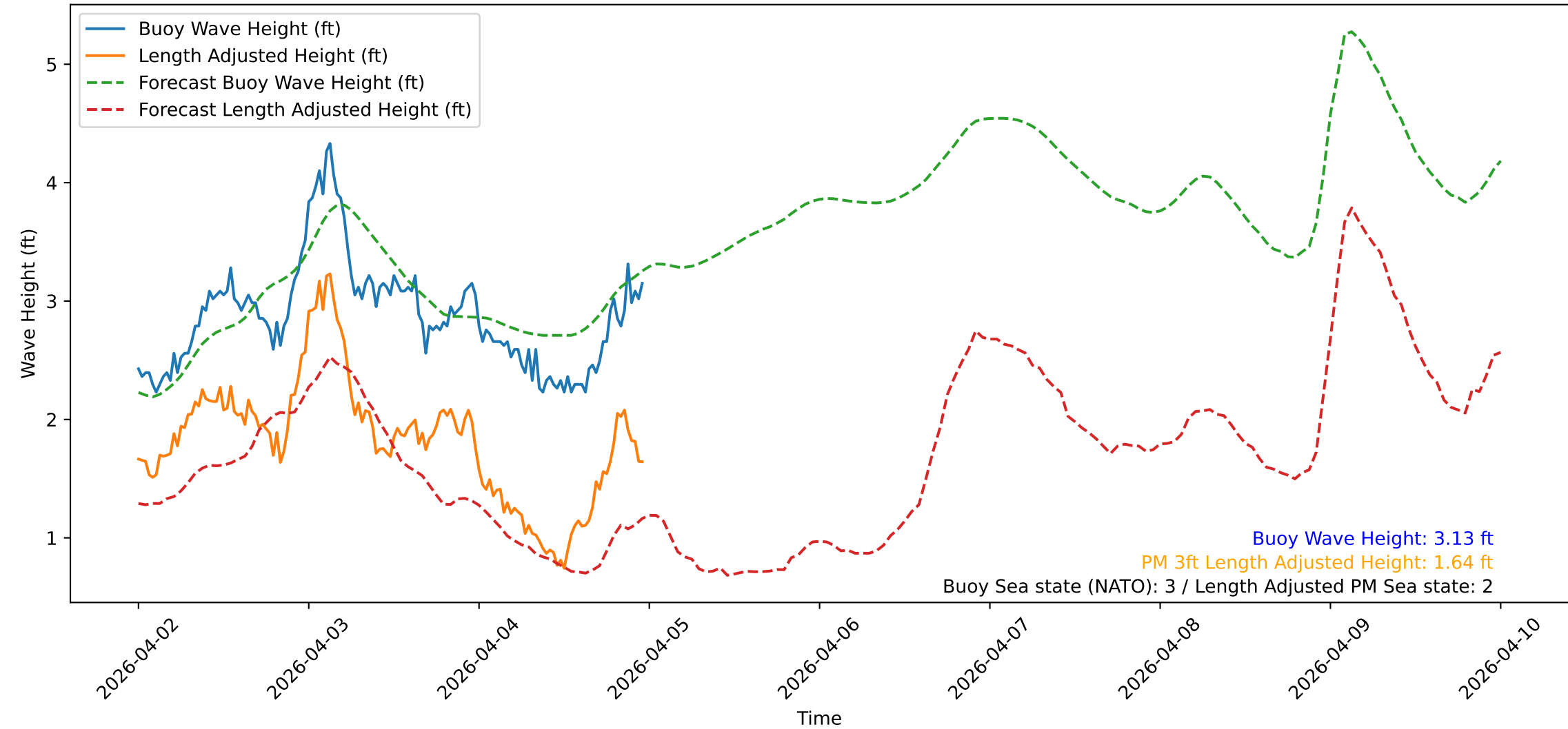
Wave Heights over Time for Green Beach at 2026-04-05 00:01:10
