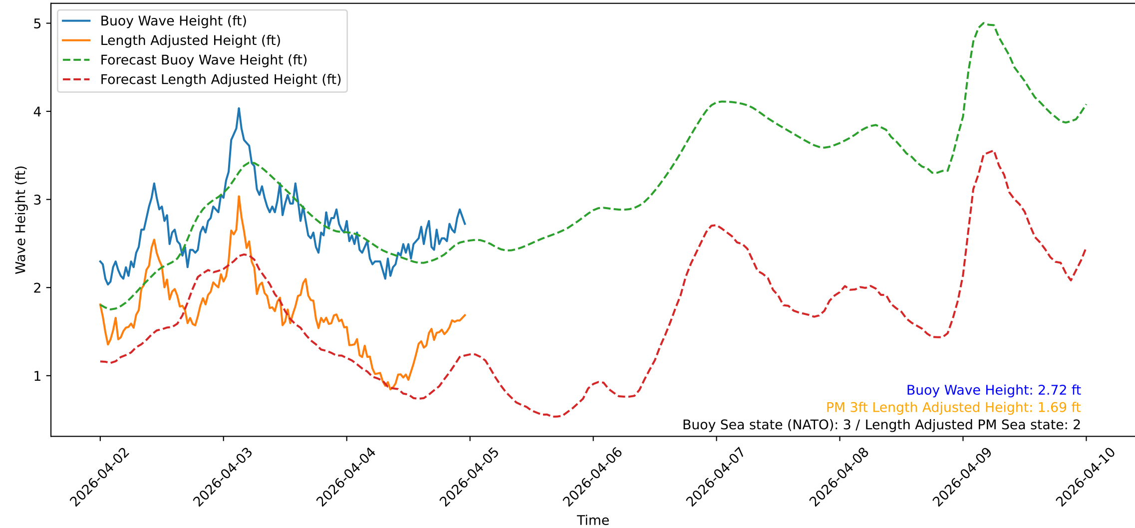
Wave Heights over Time for Oceanside Harbor at 2026-04-05 00:00:32
