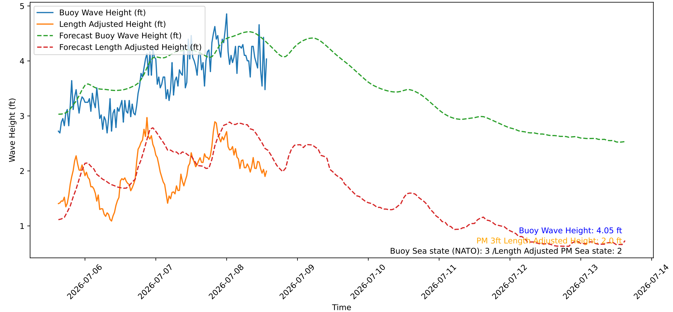
Wave Heights over Time for Red Beach at 2026-07-08 14:50:48
