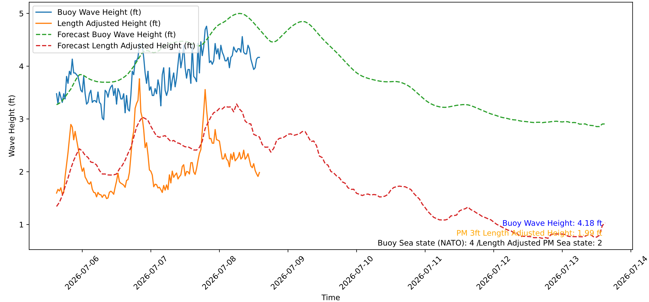
Wave Heights over Time for Green Beach at 2026-07-08 14:51:10
