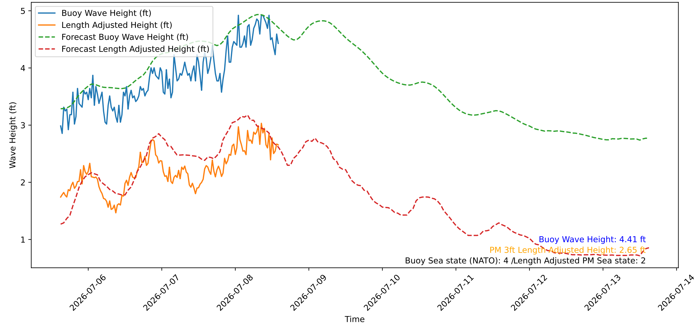
Wave Heights over Time for Oceanside Harbor at 2026-07-08 14:50:26
