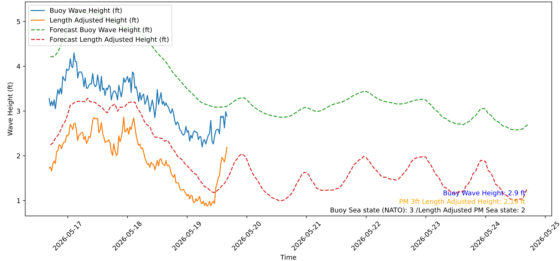
Wave Heights over Time for Oceanside Harbor at 2026-05-19 16:30:31
