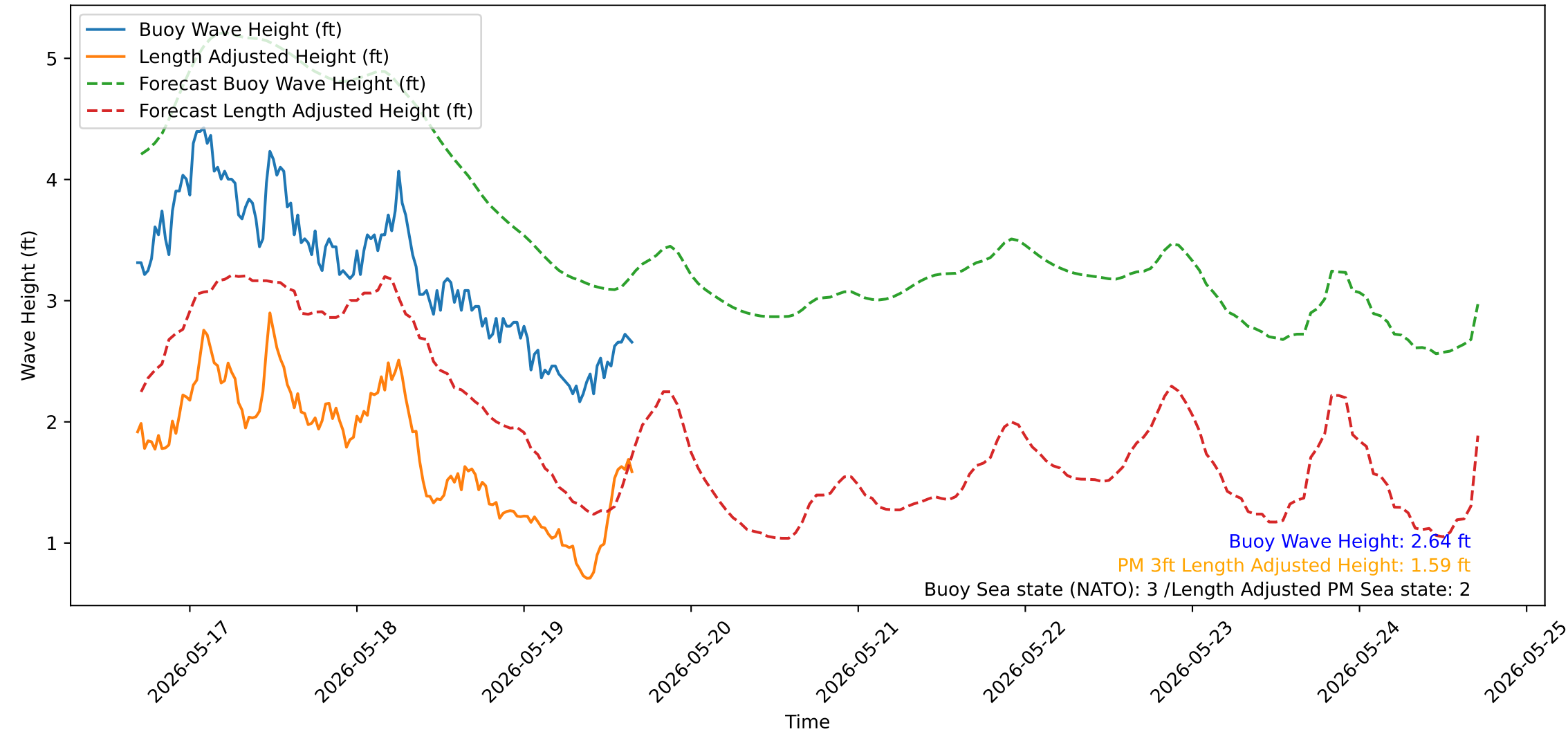
Wave Heights over Time for Green Beach at 2026-05-19 16:31:13
