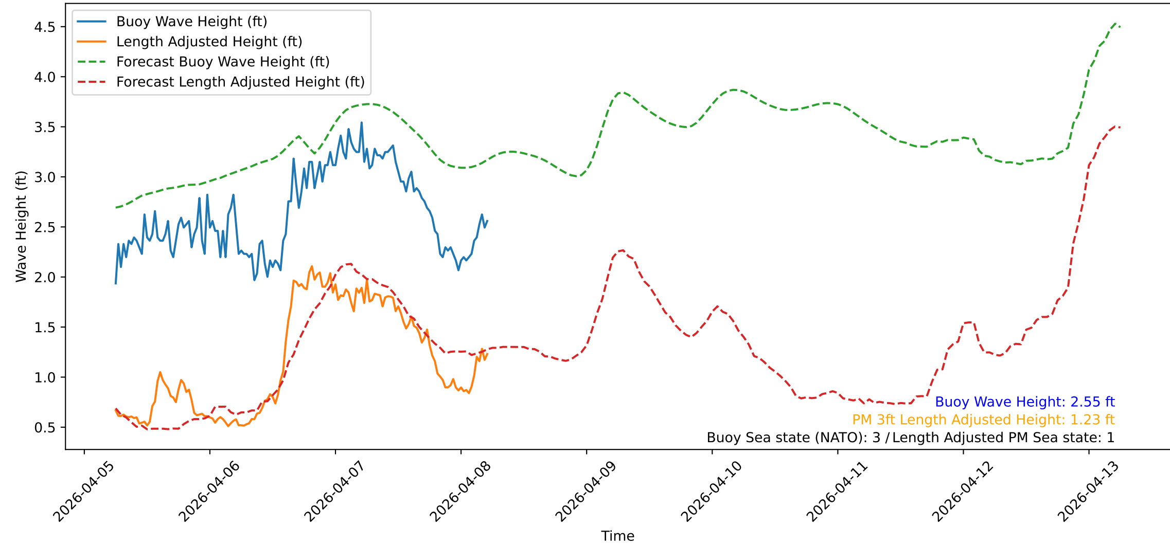
Wave Heights over Time for Red Beach at 2026-04-08 05:40:47
