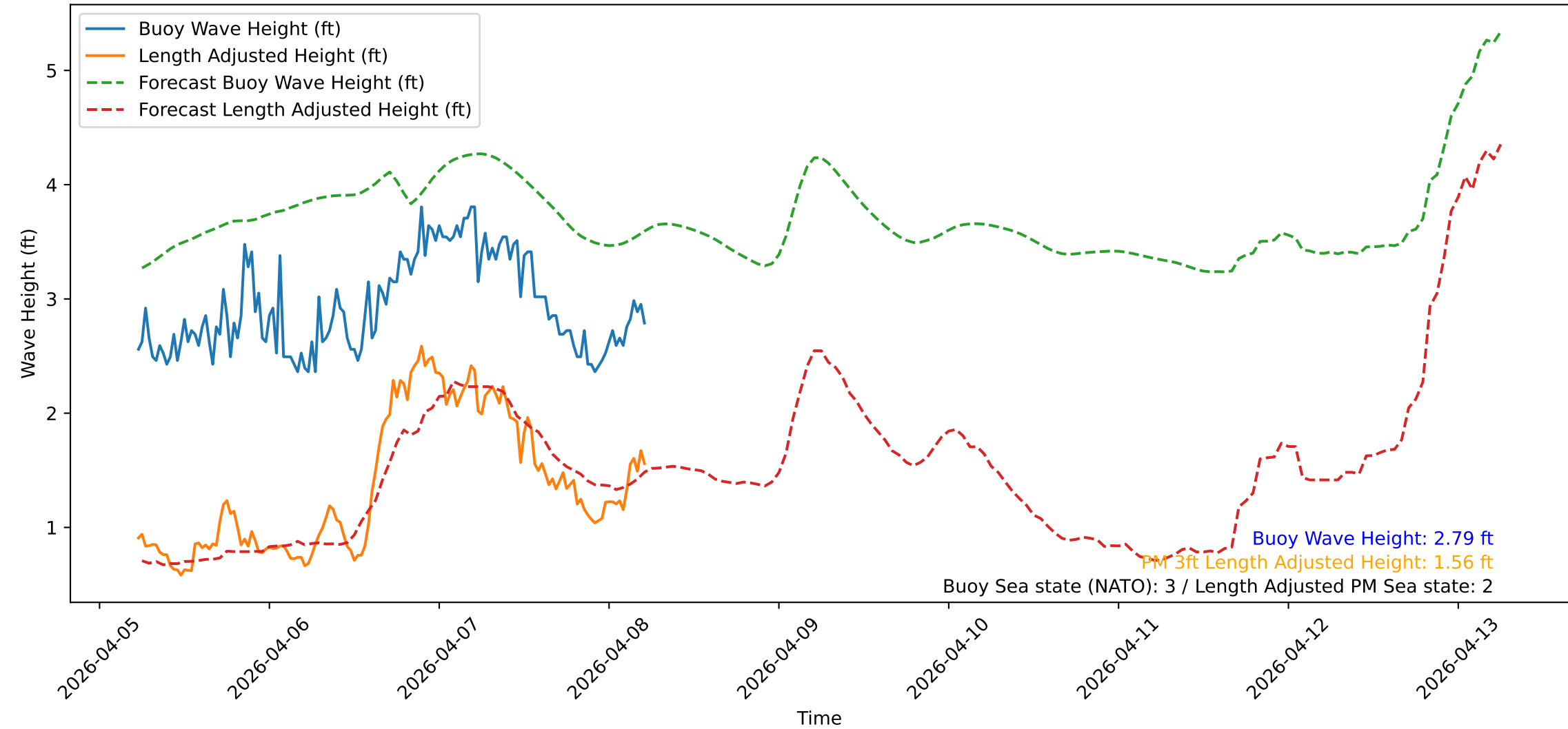
Wave Heights over Time for Green Beach at 2026-04-08 05:41:10
