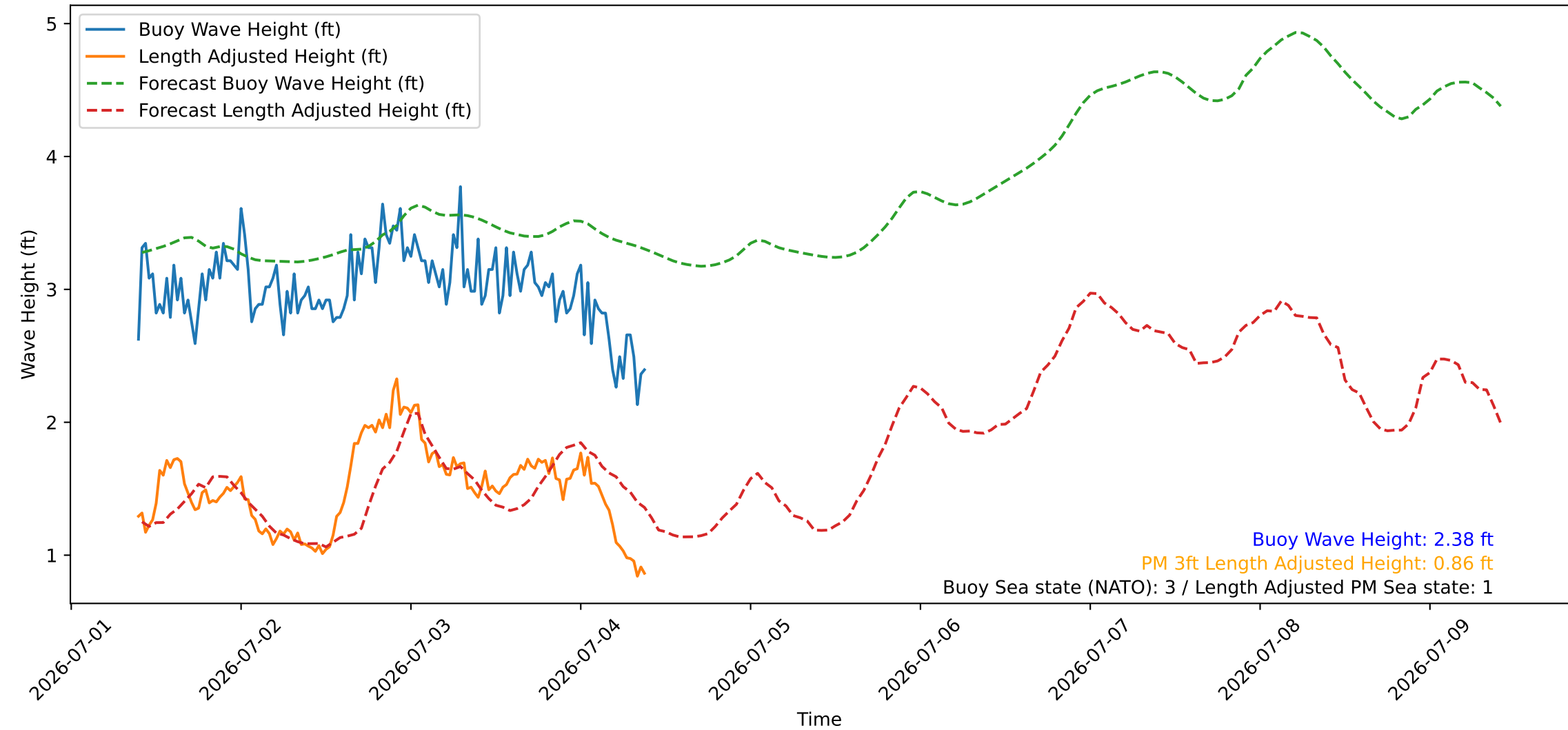
Wave Heights over Time for Oceanside Harbor at 2026-07-04 09:40:27
