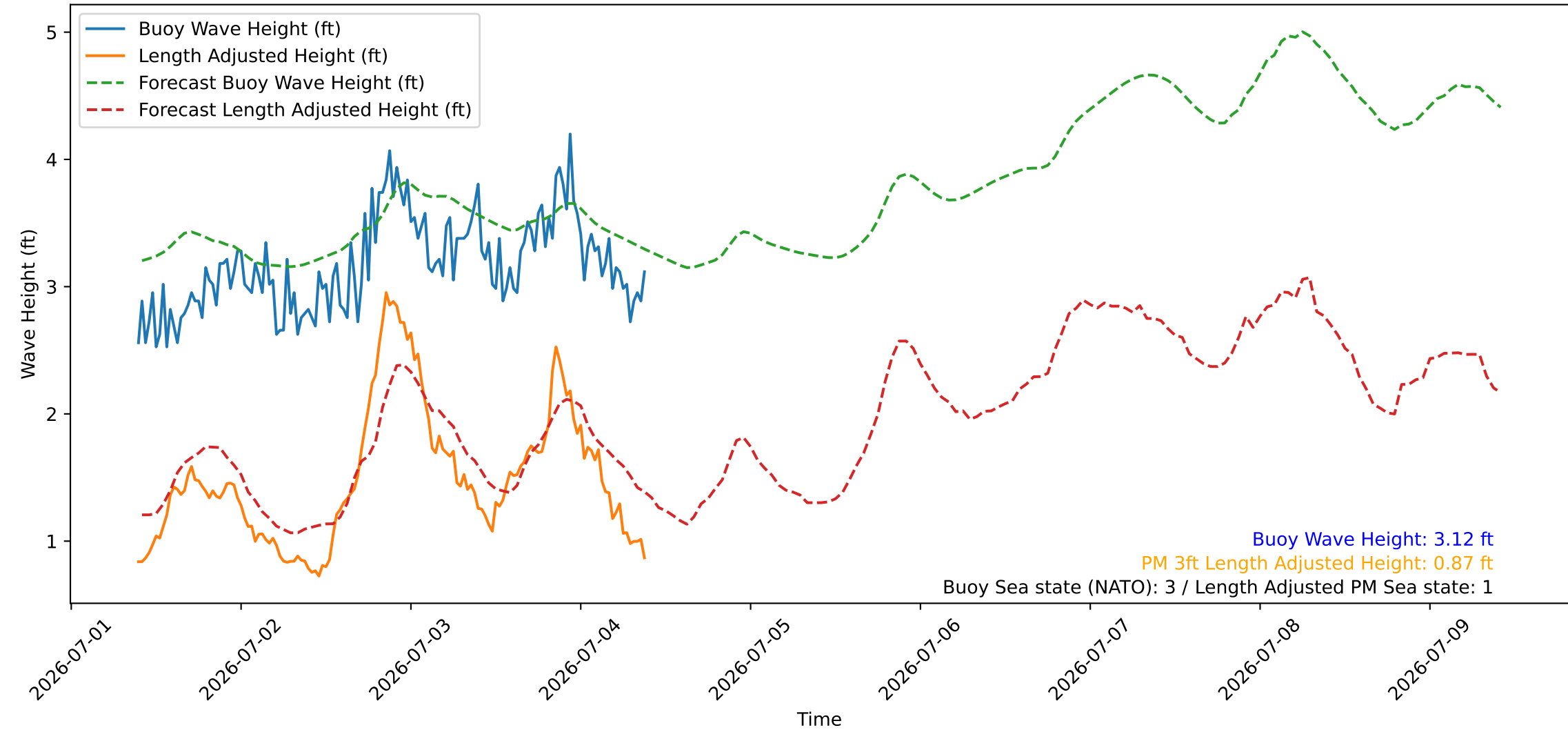
Wave Heights over Time for Green Beach at 2026-07-04 09:41:10
