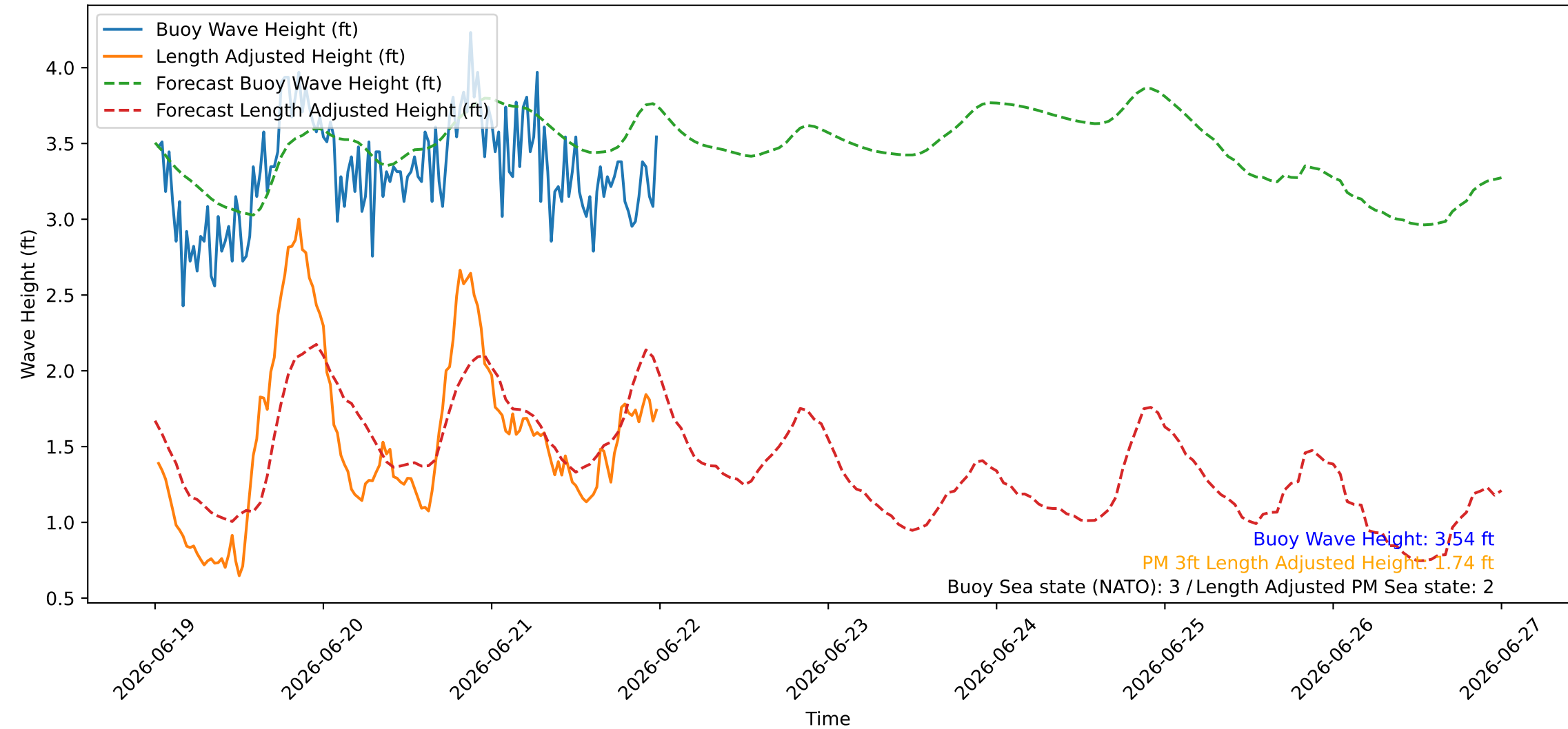
Wave Heights over Time for Green Beach at 2026-06-22 00:21:10
