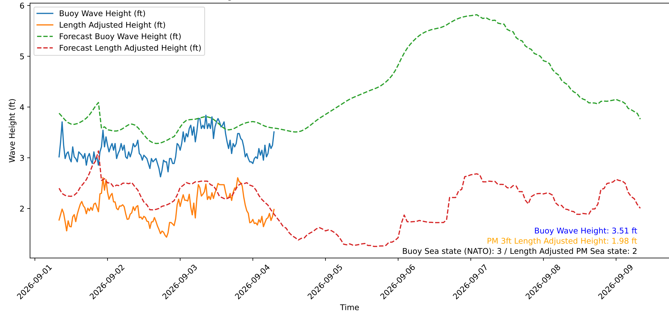
Wave Heights over Time for Oceanside Harbor at 2026-09-04 08:00:30
