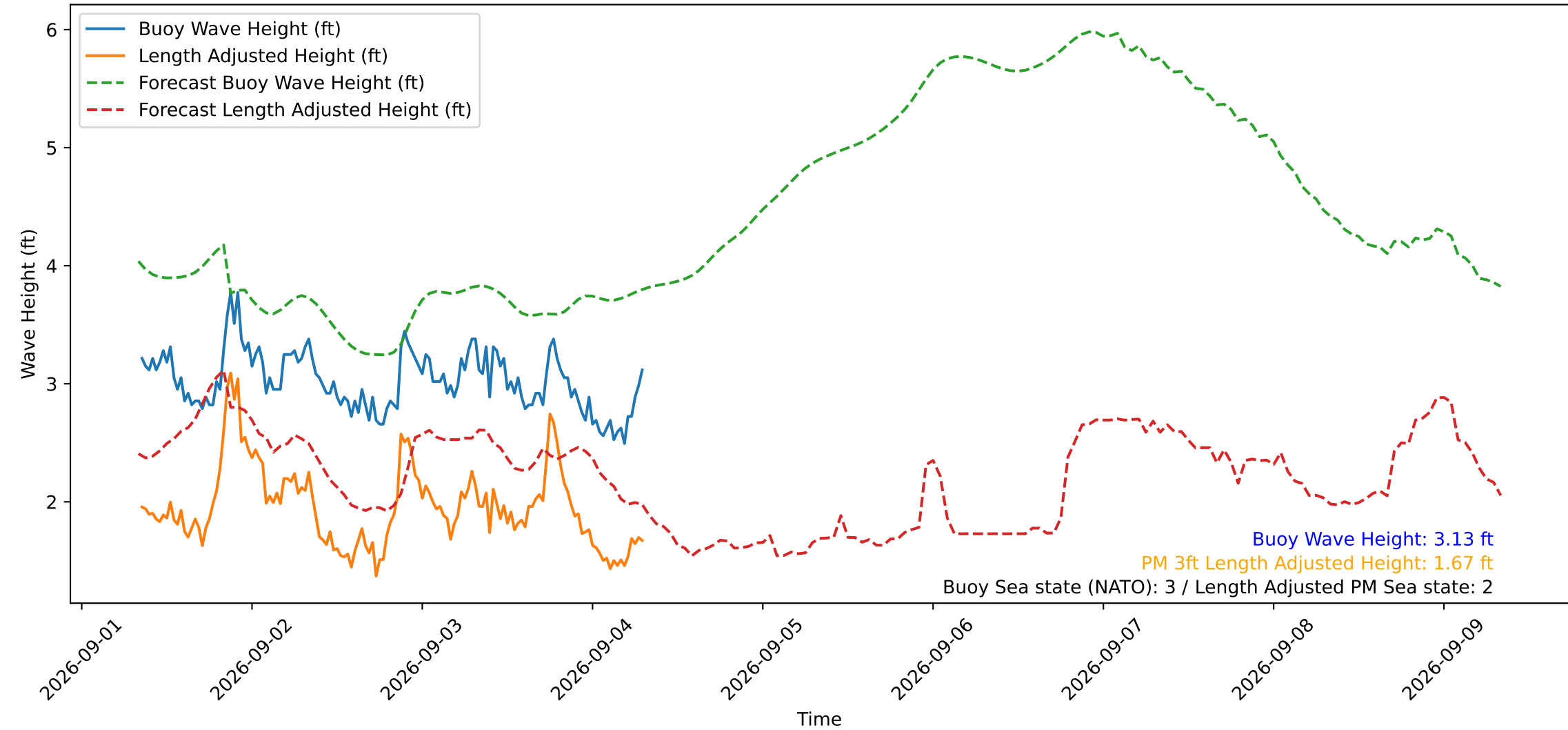
Wave Heights over Time for Green Beach at 2026-09-04 08:01:13
