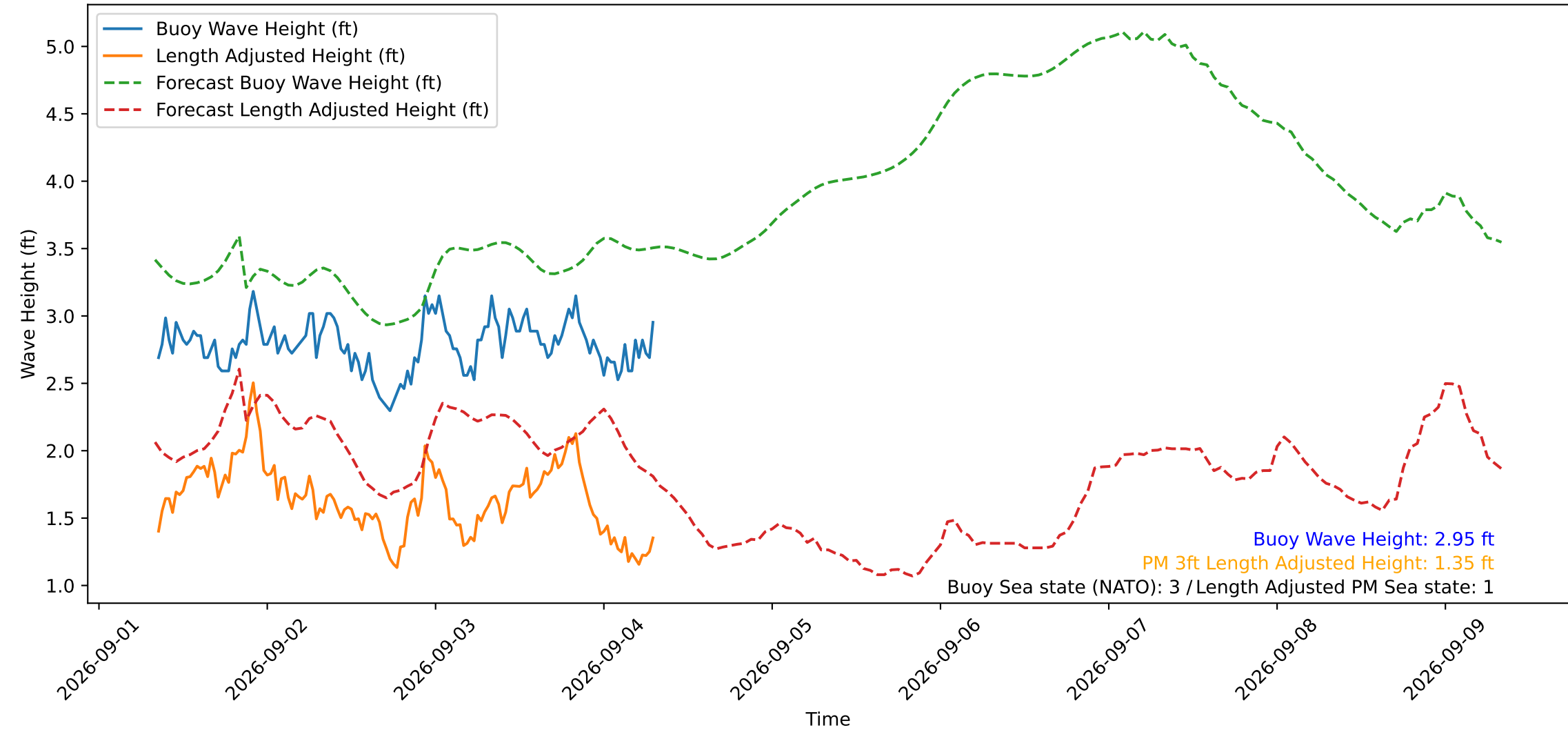
Wave Heights over Time for Red Beach at 2026-09-04 08:00:50
