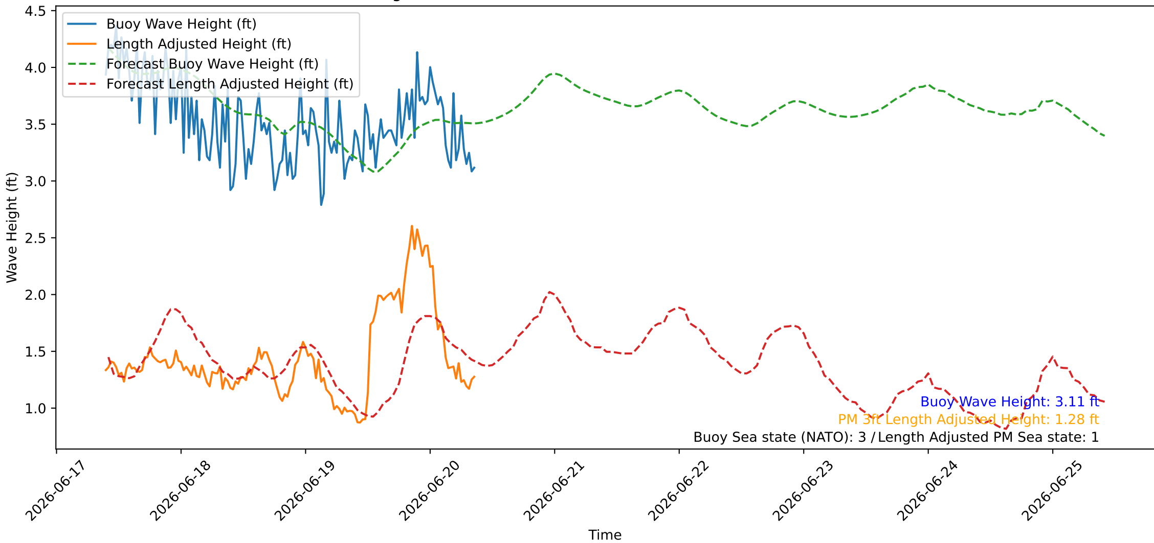
Wave Heights over Time for Oceanside Harbor at 2026-06-20 09:30:25
