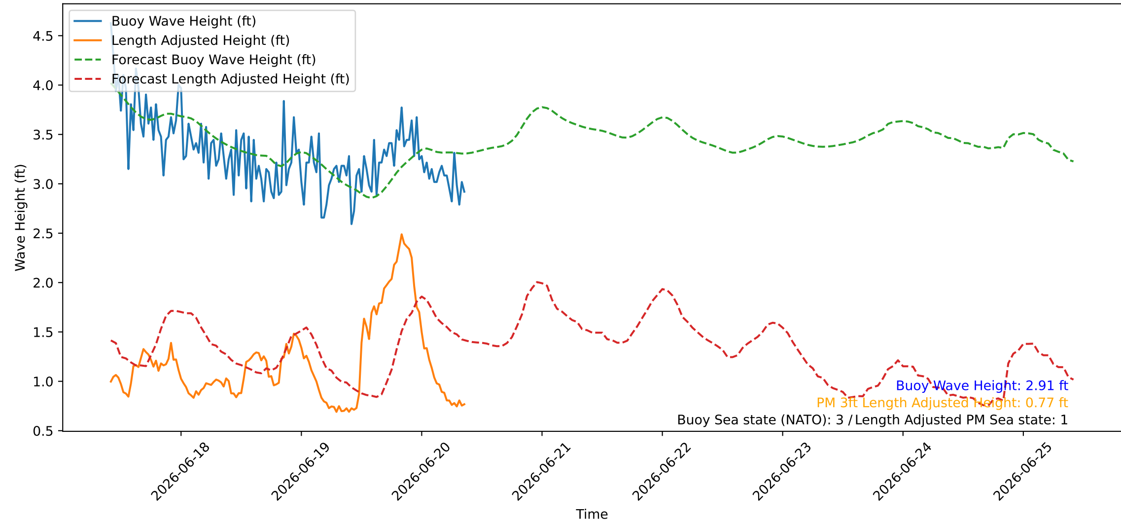
Wave Heights over Time for Red Beach at 2026-06-20 09:30:44
