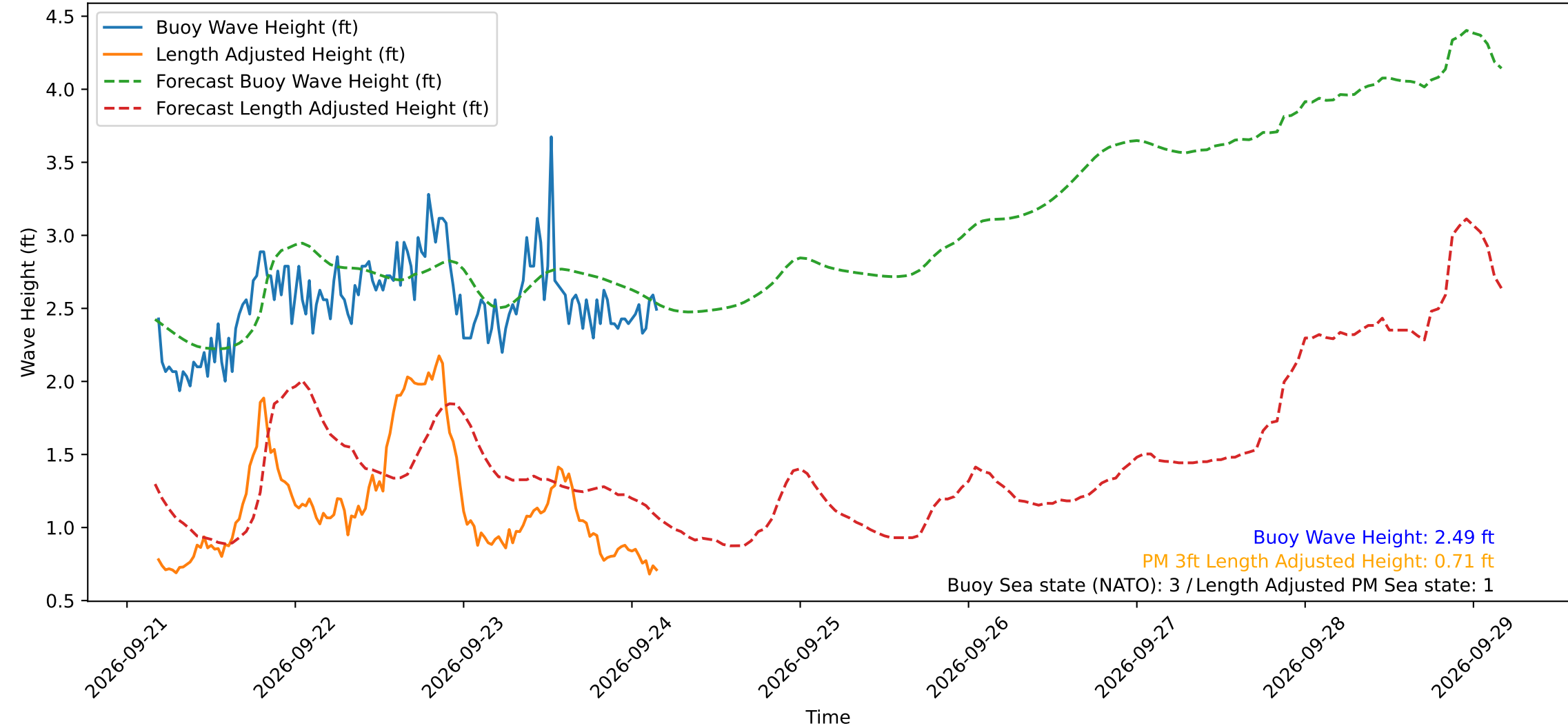
Wave Heights over Time for Red Beach at 2026-09-24 04:20:49
