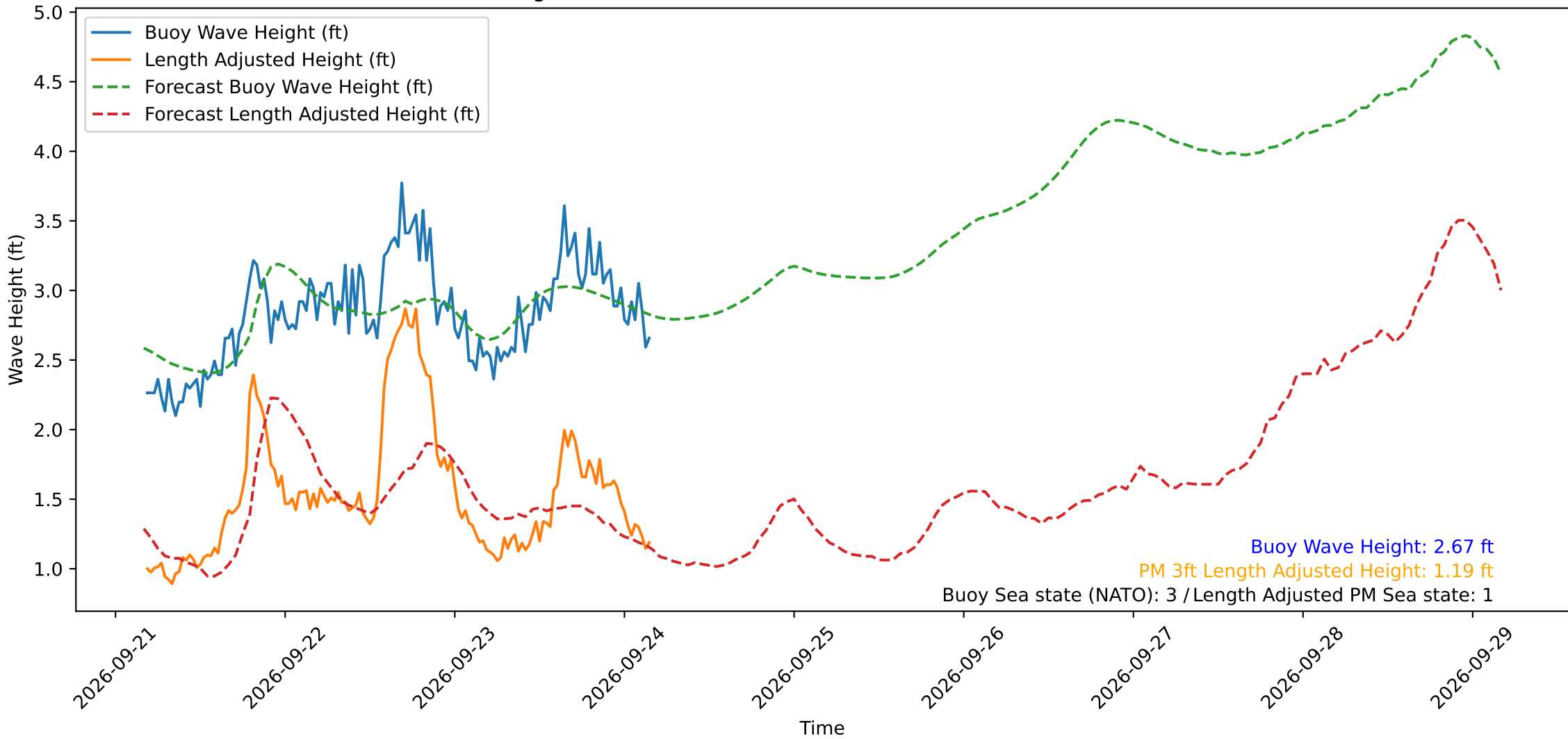
Wave Heights over Time for Oceanside Harbor at 2026-09-24 04:20:29
