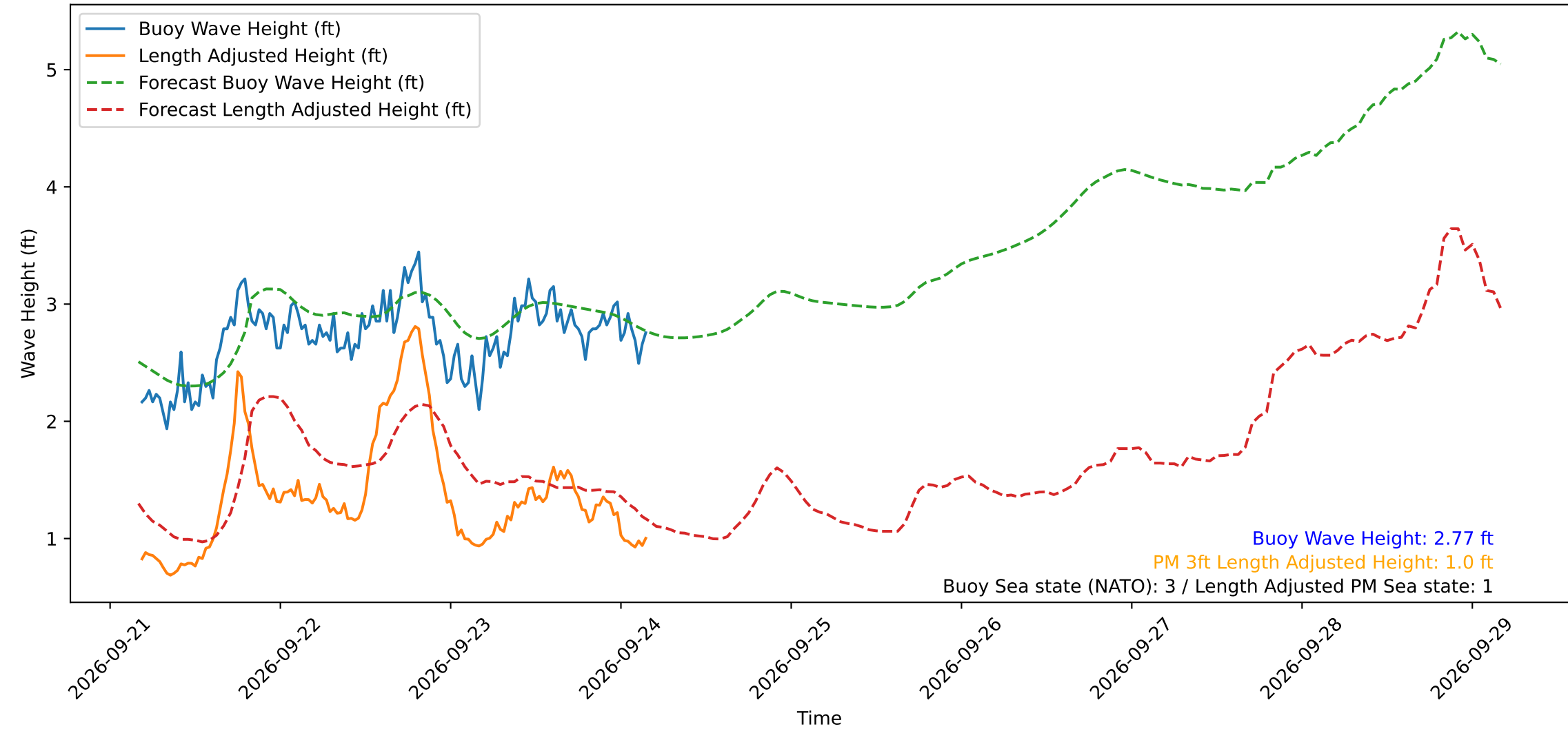
Wave Heights over Time for Green Beach at 2026-09-24 04:21:13
