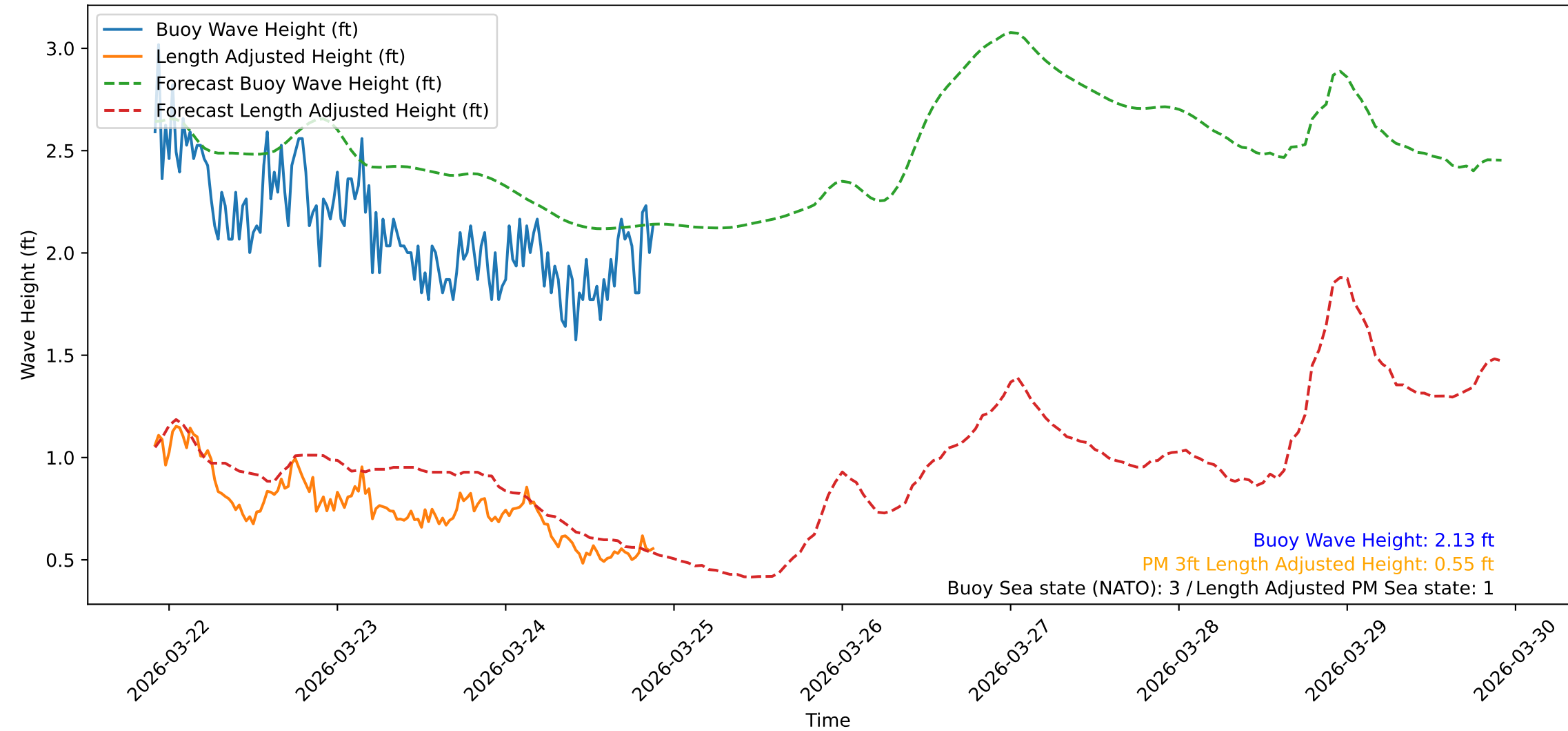
Wave Heights over Time for Oceanside Harbor at 2026-03-24 21:50:31
