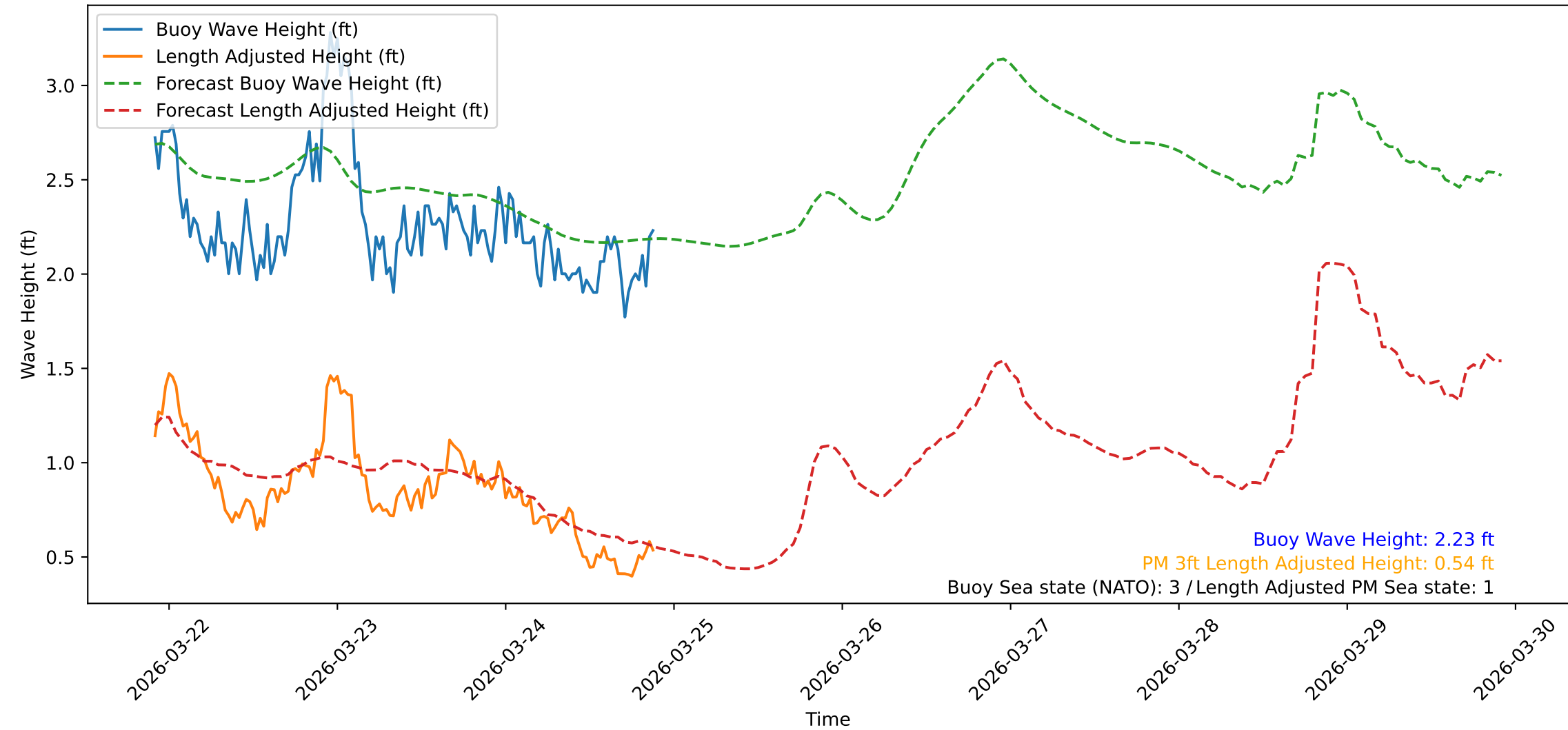
Wave Heights over Time for Green Beach at 2026-03-24 21:51:09
