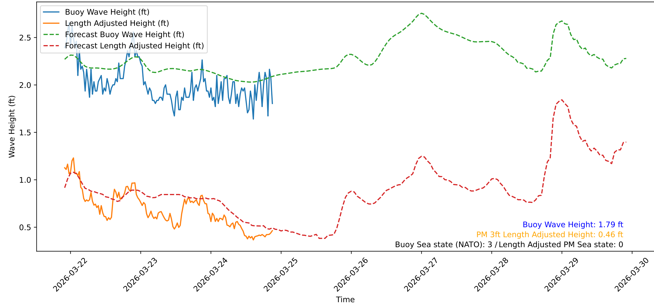
Wave Heights over Time for Red Beach at 2026-03-24 21:50:47
